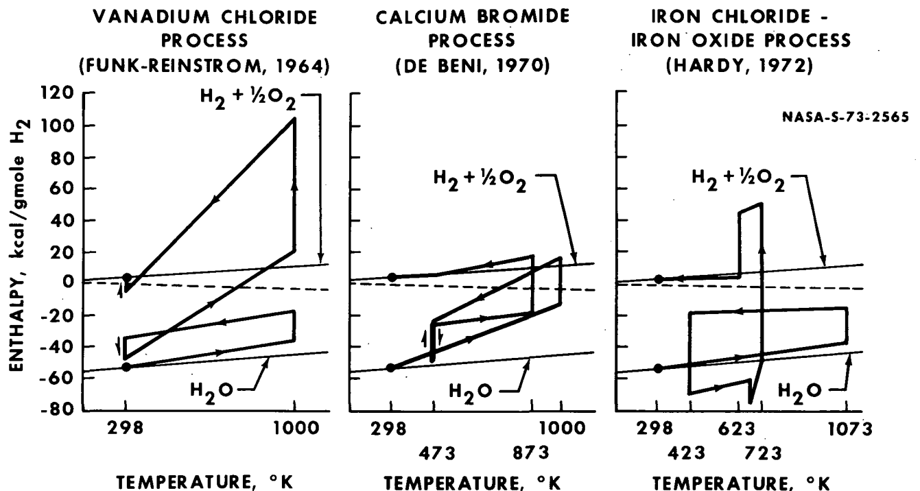
FIGURE 3-15 THREE MULTISTEP WATER SPLITTING PROCESSES (H-T DIAGRAMS)
