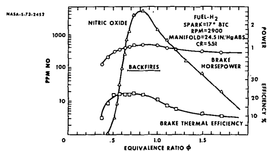
FIGURE 5-7 EMISSION CHARACTERISTICS- CARBURETED H 2 ENGINE
