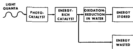
FIGURE 3-16 ENERGY PATH OF PHOTOLYSIS
