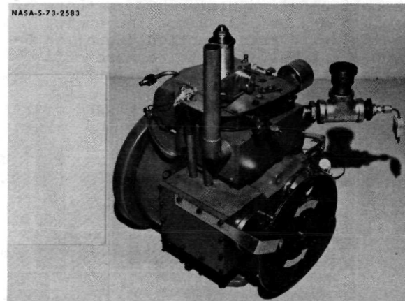
FIGURE 5-5 OKLAHOMA STATE UNIVERSITY HYDROGEN FUELED ENGINE
