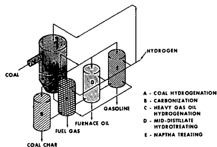
FIGURE 3-9 HYDROGENATION OF COAL TO PRODUCE CONVENTIONAL HYDROCARBONS
