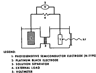
FIGURE 3-18 PHOTO-ELECTROCHEMICAL CELL
