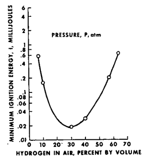
FIGURE 5-13 SPARK IGNITION ENERGIES FOR HYDROGEN-AIR MIXTURES AT VARIOUS PRESSURES
