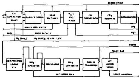
FIGURE 5-28 AMMONIA PROCESS WITH FUEL GASIFICATION PLANT AND AIR SEPARATION
