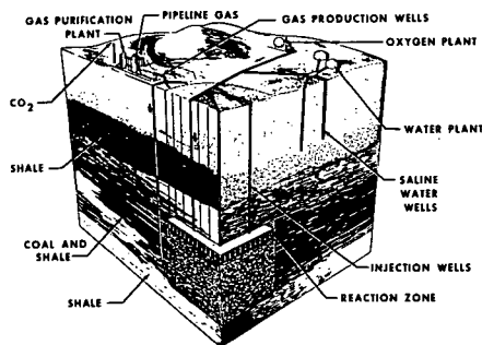
FIGURE 3-12 IN SITU COAL GASIFICATION
