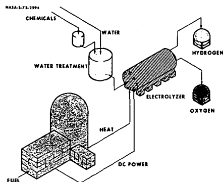
FIGURE 3-26 NUCLEAR-ELECTROLYSIS PLANT
