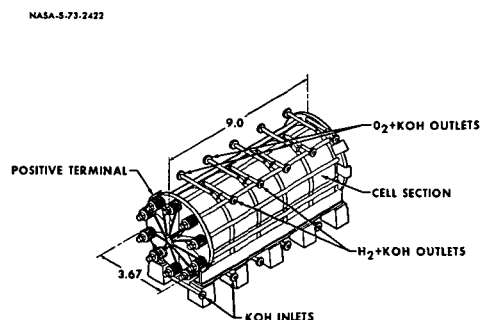
FIGURE 3-5 ADVANCED ELECTROLYSIS CELL
