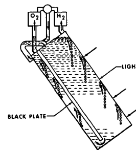
FIGURE 3-17 PHOTOLYSIS CELL
