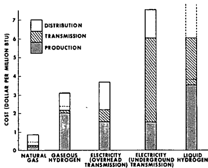
FIGURE 4-1 COMPARATIVE COST OF DELIVERED ENERGY
