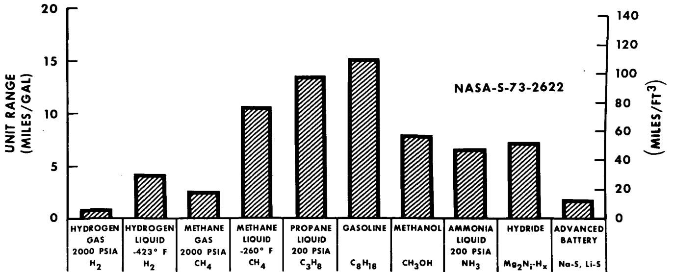
FIGURE 5-23 RELATIVE RANGE FOR SELECTED SYNTHETIC FUELS
