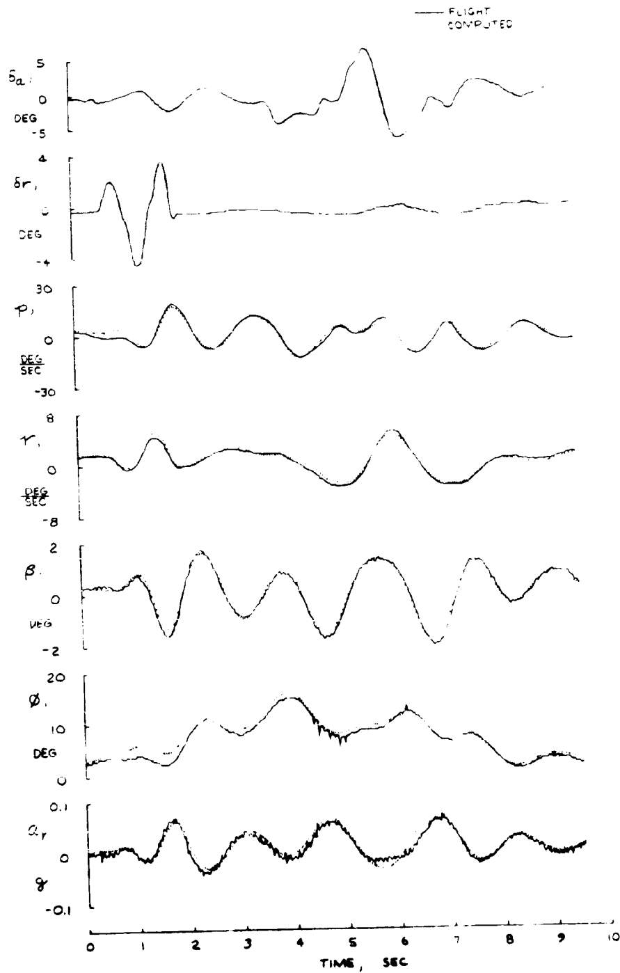
Figure 2. Typical comparison of the flight and computed time histories.
