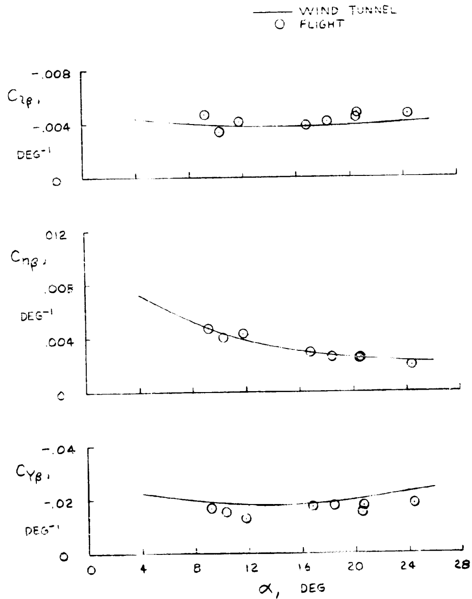
Figure 8. Comparison of derivatives obtained from flight data with wind-tunnel predictions for a Mach number of 1.2.
