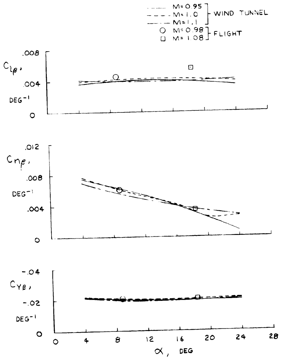
Figure 7. Comparison of derivatives obtained from flight data with wind-tunnel predictions for Mach numbers from 0.95 to 1.1.
