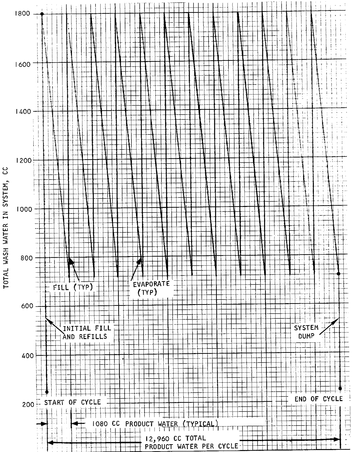
Figure 3-8. Nominal System Cycle
