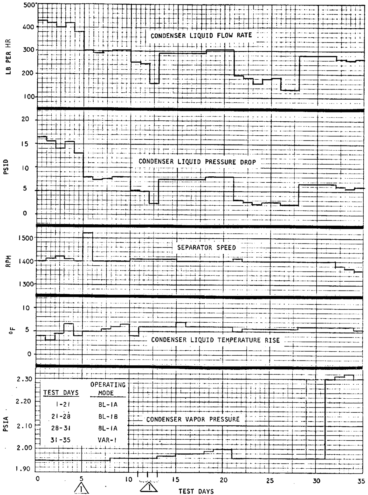
Figure 3-10. Major Operating Parameter Values, Days 1-35
