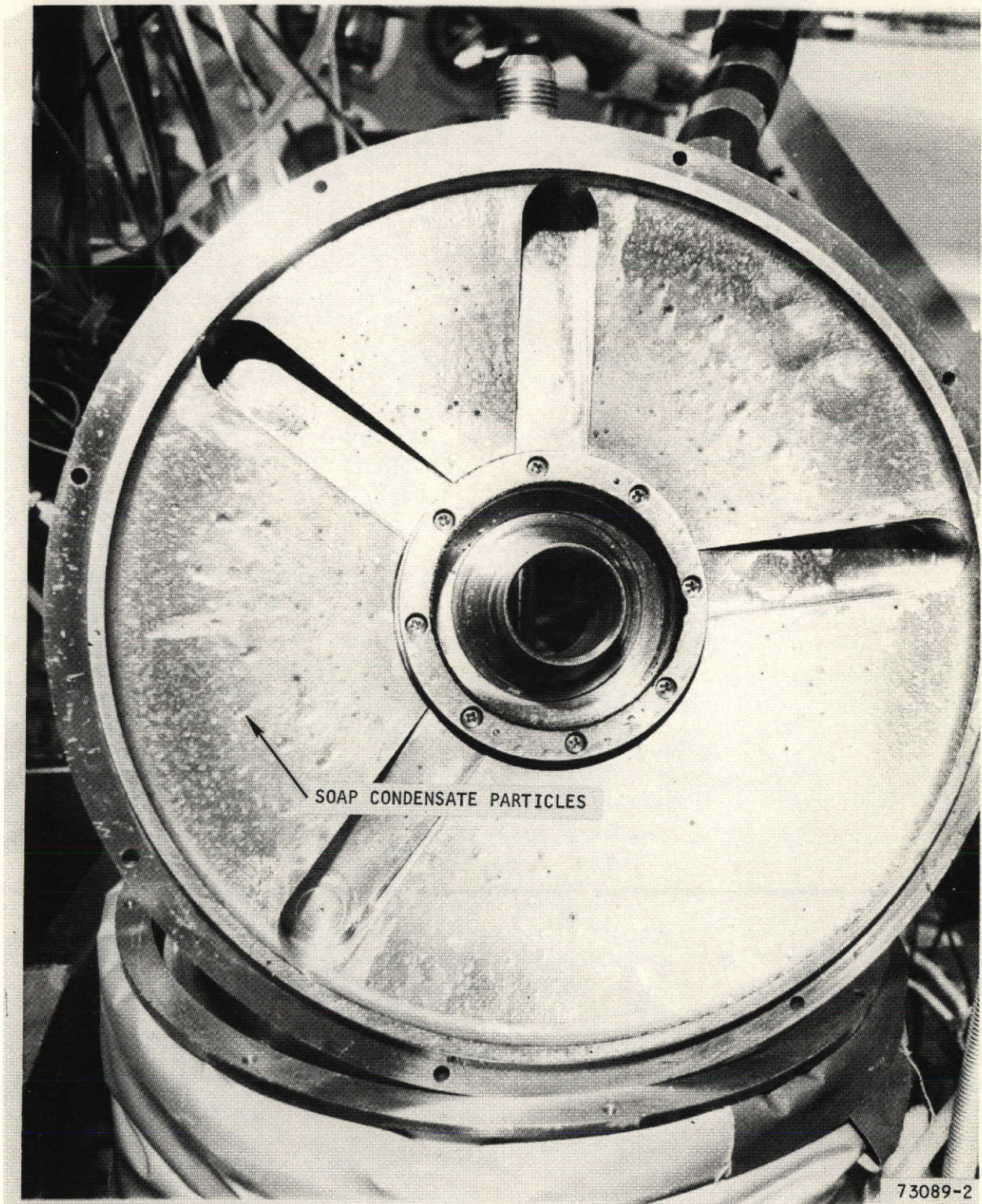
Figure 3-15. Post Phase I Examination, Appearance of Inside Surface of Separator Outer Bowl Top Cover
