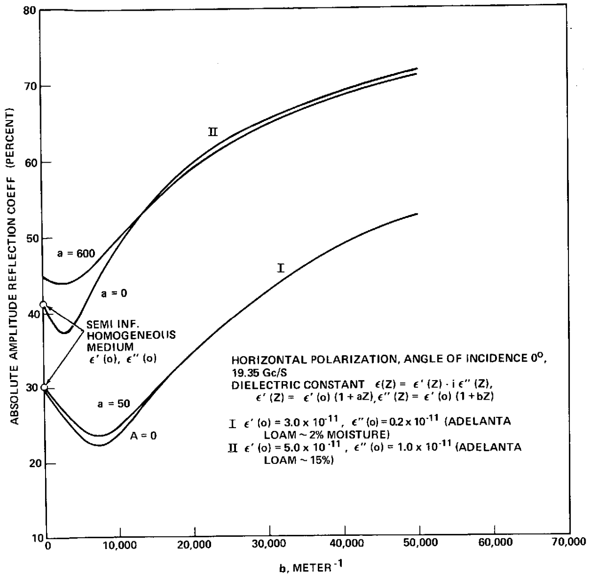
Figure 3. Absolute amplitude reflection coefficient for a semi infinite inhomogeneous medium with dielectric constant linearly dependent on z. No boundary layer; horizontal polarization; angle of incidence, 0^\circ ; frequency, 19.35 Gc/sec.
