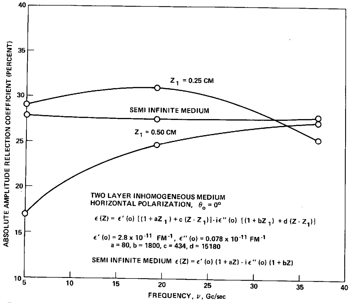
Figure 6. Absolute amplitude reflection coefficient for a two layer inhomogeneous medium as a function of frequency. Dielectric constant of inhomogeneous media linearly dependent on z. Horizontal polarization; angle of incidence, 0^\circ .
