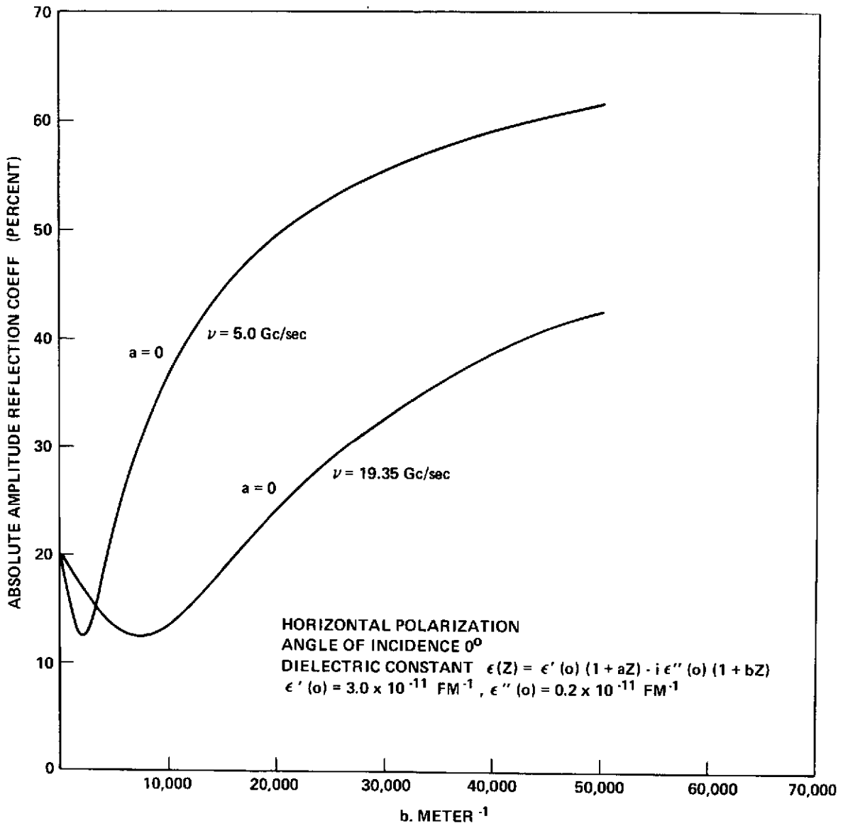
Figure 4. Absolute amplitude reflection coefficient for a semi infinite inhomogeneous medium with dielectric constant linearly dependent on z . No boundary layer; horizontal polarization; angle of incidence, 0^\circ ; frequency, 19.35, and 5.0 Gc/sec.
