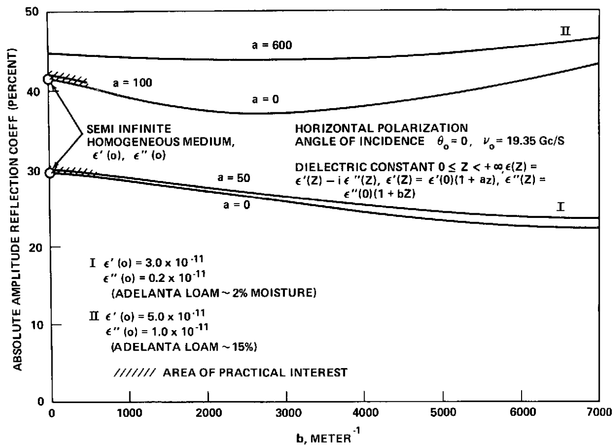
Figure 2. Absolute amplitude reflection coefficient for a semi infinite inhomogeneous medium with dielectric constant linearly dependent on z. No boundary layer; horizontal polarization; angle of incidence, 0^\circ ; frequency, 19.35 Gc/sec.
