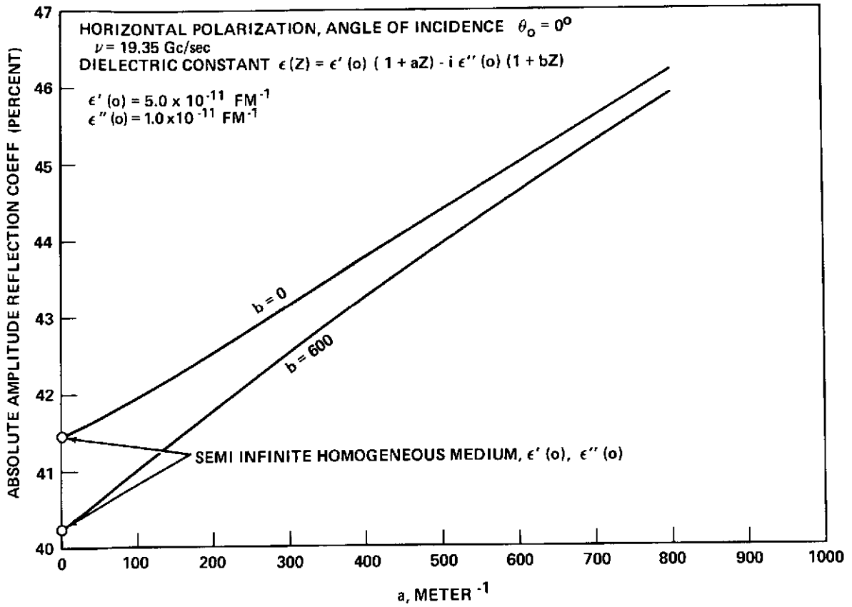
Figure 5. Absolute amplitude reflection coefficient for a semi infinite inhomogeneous medium, with dielectric constant linearly dependent on z, as a function of the parameter a. No boundary layer; horizontal polarization, angle of incidence, 0^\circ ; frequency, 19.35 Gc/sec.
