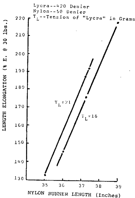
Figure 3. Effect on length elongation of nylon runner length.
