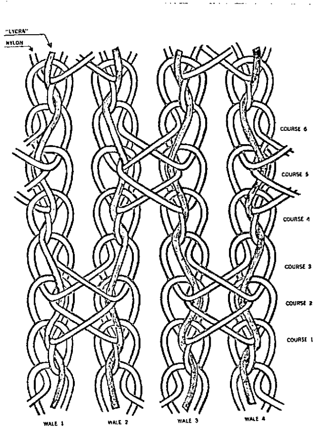
Figure 1. Power-Net Diagram.
