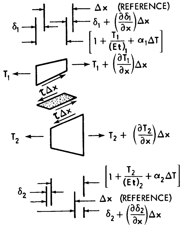
DISPLACEMENTS AND ELEMENT LOADS
