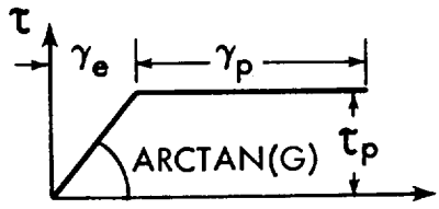
ADHESIVE SHEAR CHARACTERISTIC
