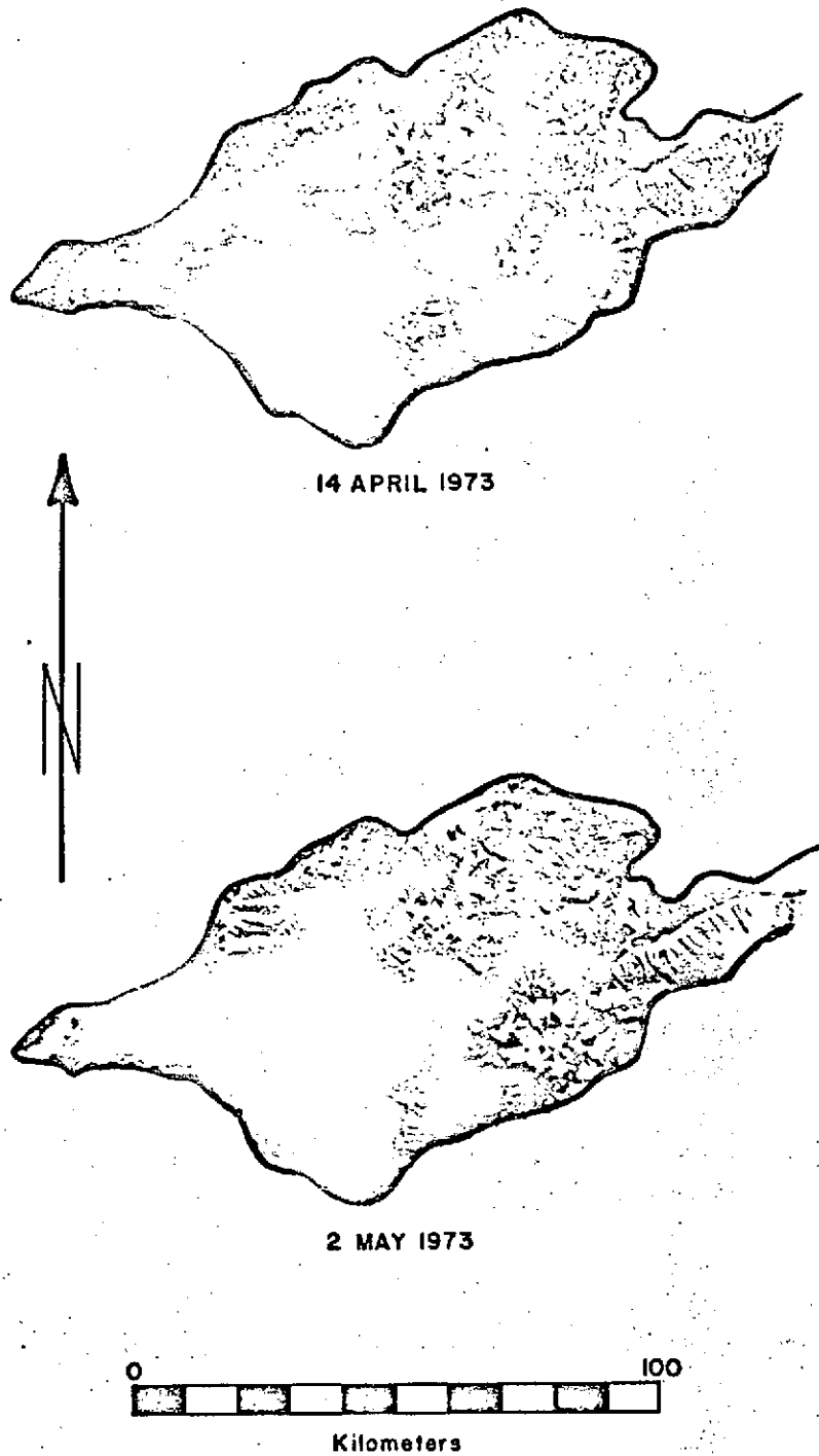
Figure 7. Imagery of the Chena River Basin as seen from ERTS. 7a. 14 April 1973 (Note that most of the area is snow covered.) 7b. 2 May 1973 (Note that the lower lying areas are snow free.)
