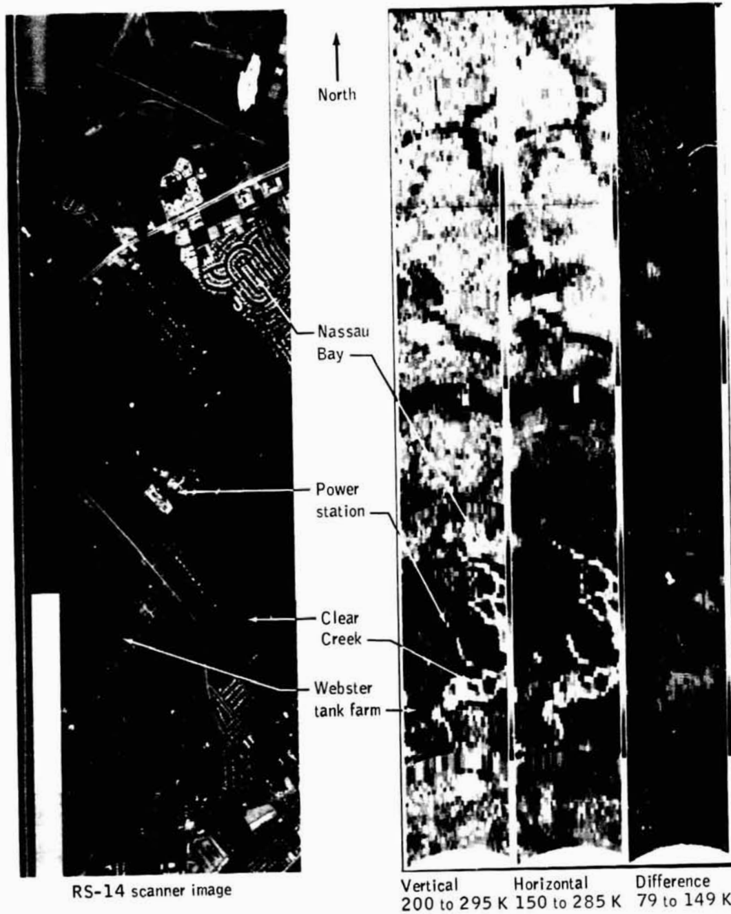
Figure 7.- Infrared (IR) and PMIS images of Webster tank farm and Clear Creek from a 1220-meter (4000-foot) altitude (average size of the PMIS beam position footprint, 137.2 by 68.6 meters (450 by 225 feet)).
