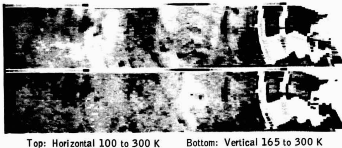
(b) Water of Clear Lake showing influence of warmer land in the antenna side lobes.
