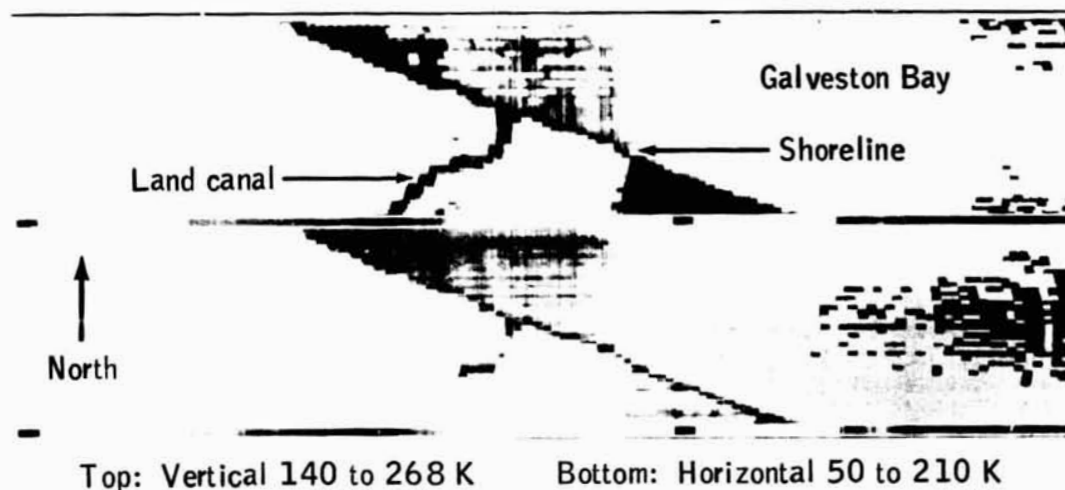
(a) Galveston Bay shoreline showing antenna side-lobe anomalies of the land and water. The warmer water of the canal changes the brightness temperature in the outlet fan but not over the large area shown.
