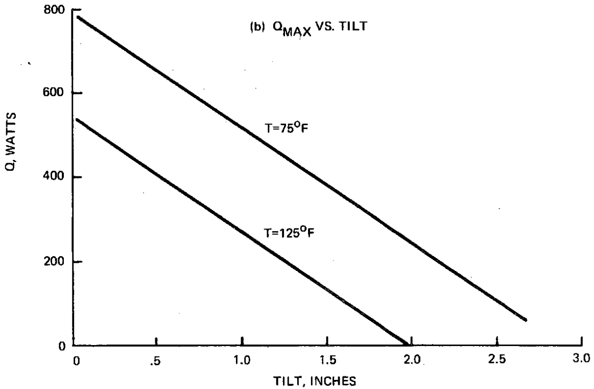
Figure 4-4 Feeder Pipe Performance
