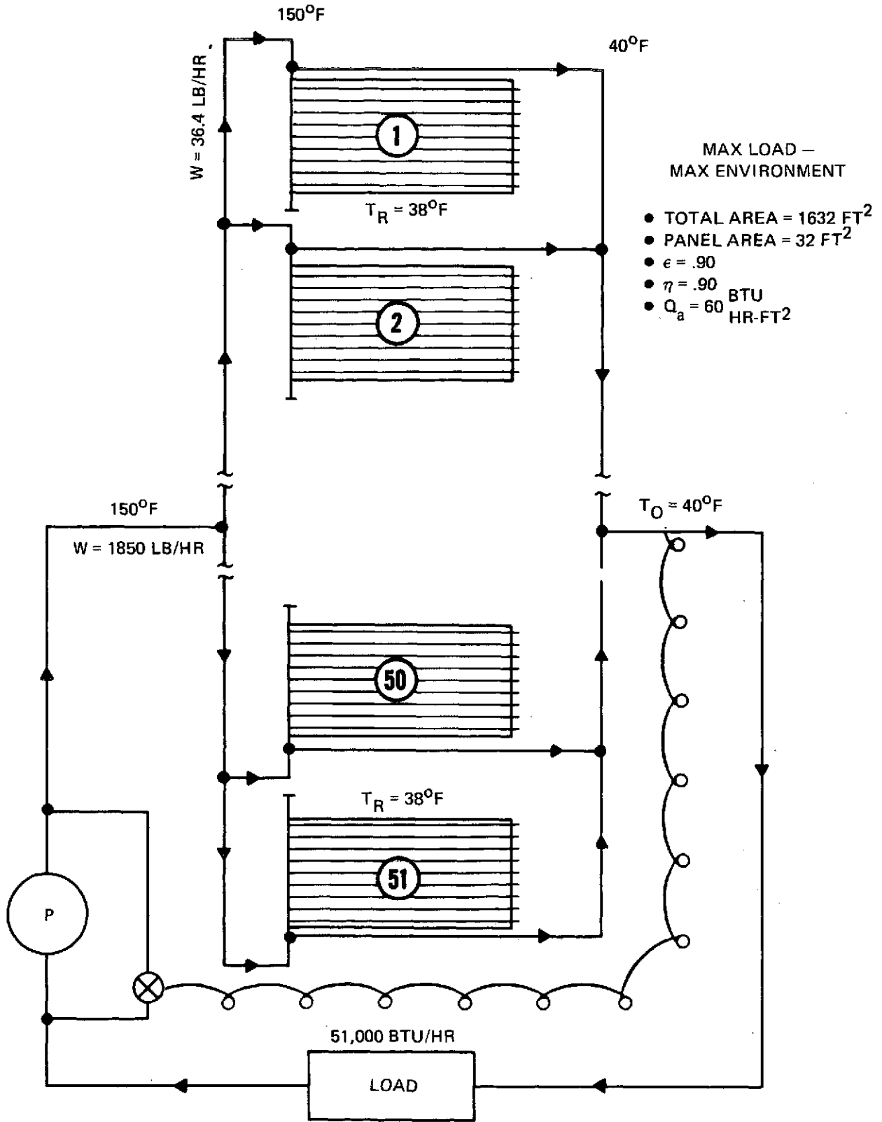
Figure 3-2 Parallel System
