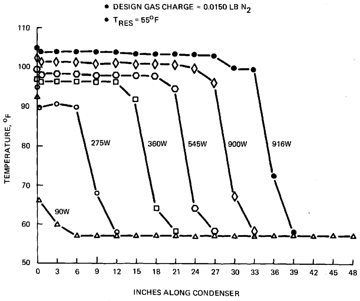
Figure 5-6 VCHP Header Bench Test Data
