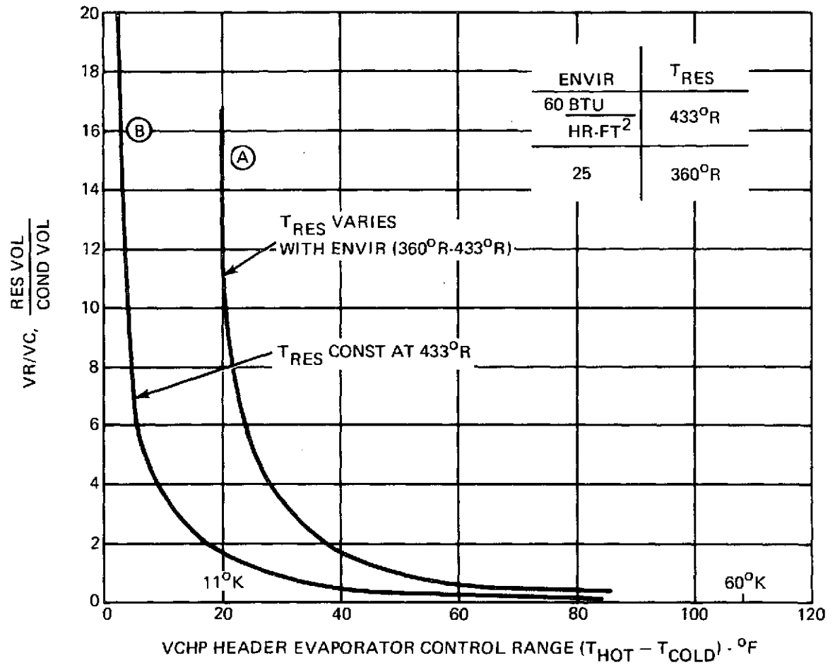
Figure 3-8 Reservoir Size vs Control Range (Based on 35° F Shutoff)
