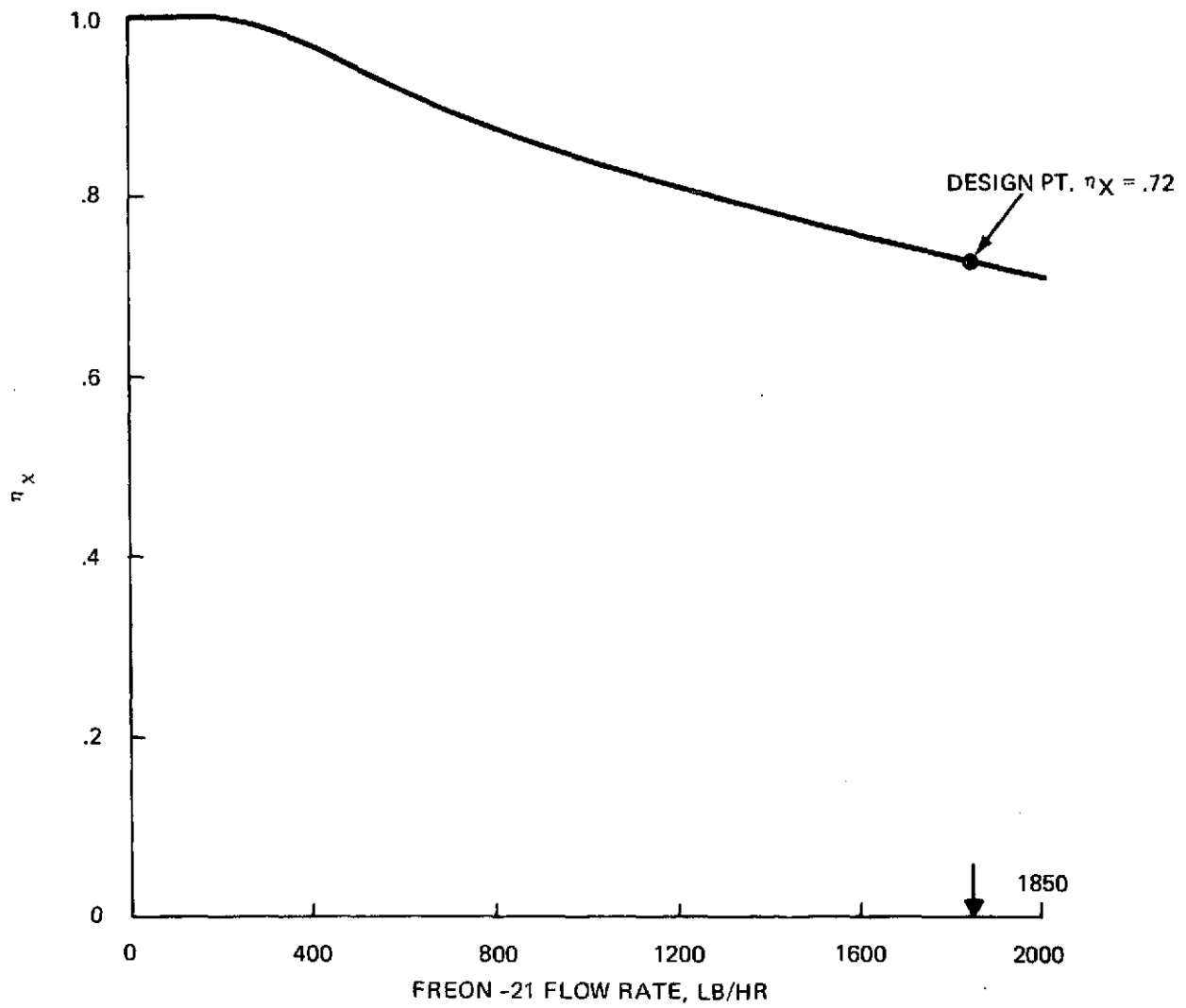
Figure 4-12 Heat Exchanger Effectiveness
