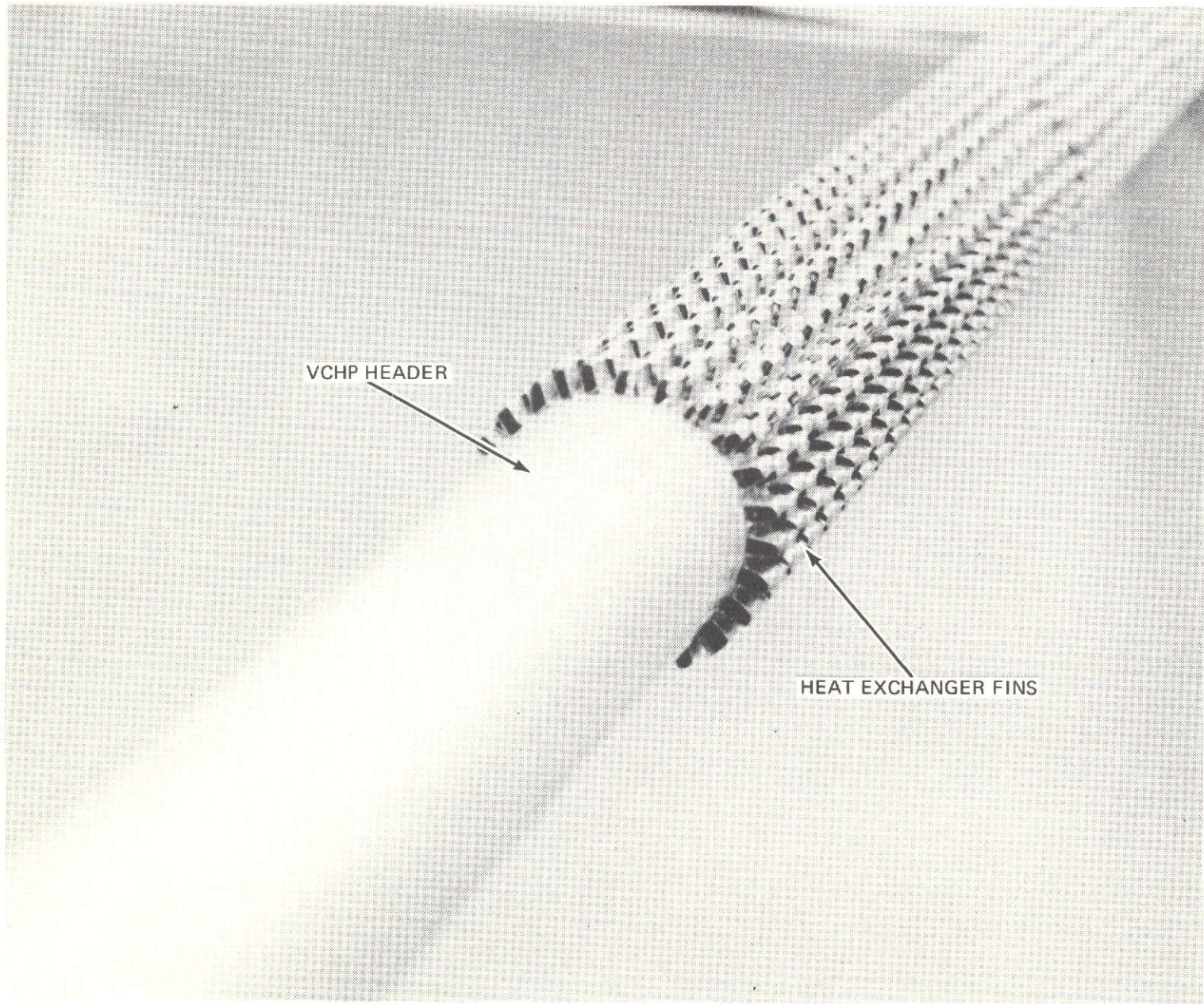
Figure 4-10 Heat Exchanger Core
