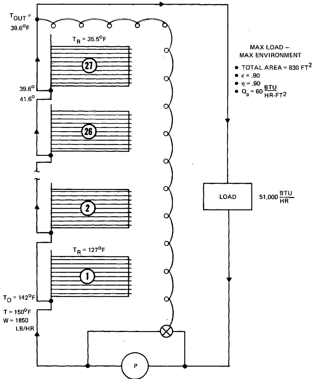
Figure 3-1 Series System
