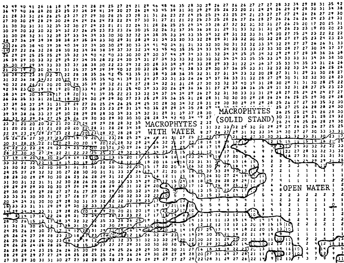
FIGURE 4 Data Posting, Sheboygan Marsh, MSS Band 7 (.8 to 1.1μ), 9 August 1972.
