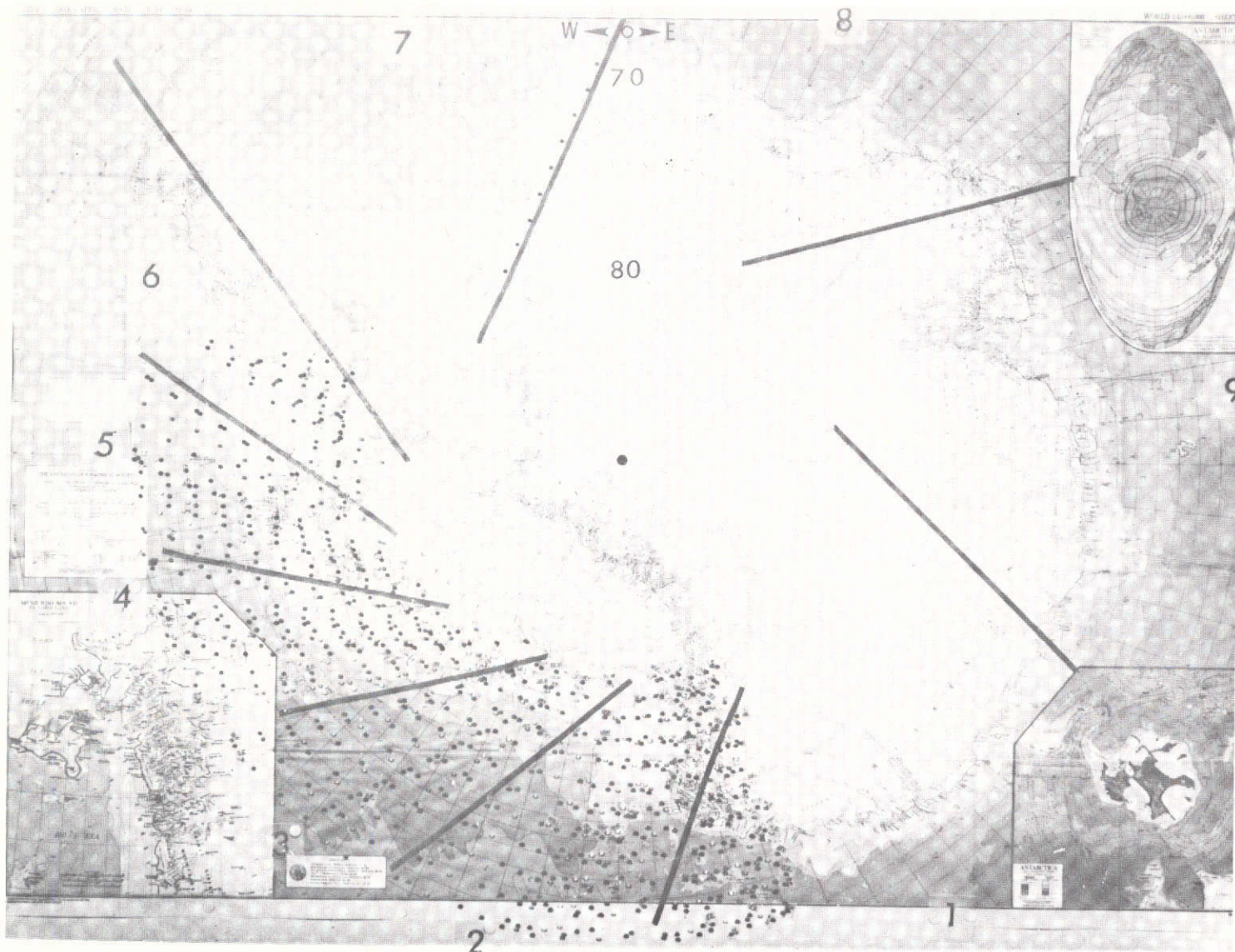
Fig. 2 — Division of Antarctica into 9 sectors and distribution of images
