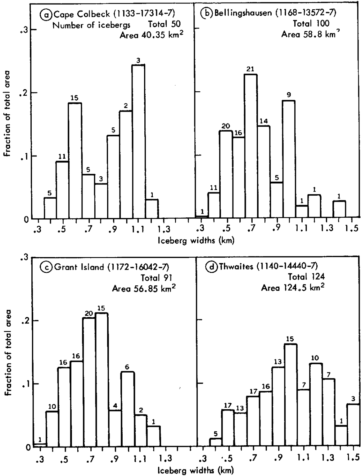
Fig. 6 — Distribution of iceberg widths in sampled areas
