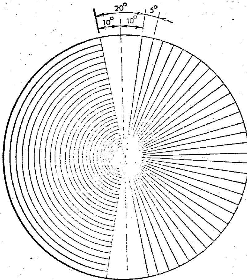
Figure 2. Detector geometry
