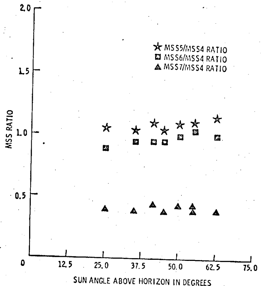
FIGURE 4. MSS BAND RATIOS FROM CCT VS. SUN ANGLE FOR TUTTLE CREEK CONCRETE DAM.
