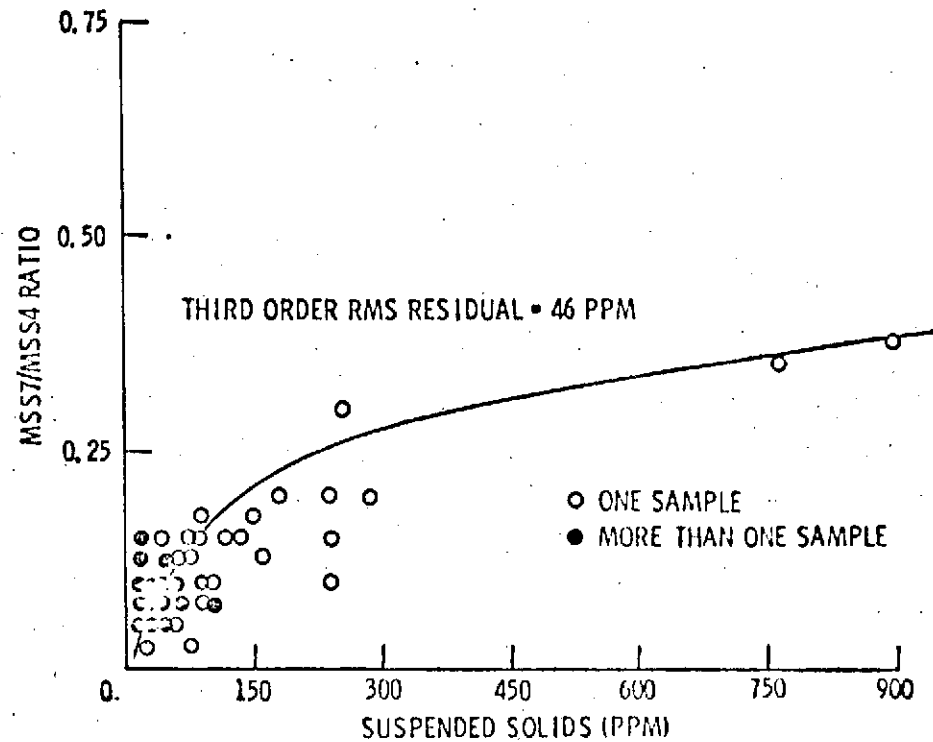
FIGURE 14. MSS7/MSS4 RATIO FROM CCT VS. SUSPENDED SOLIDS FOR 108 WATER SAMPLES FROM 11 ERTS-1 PASSES.
