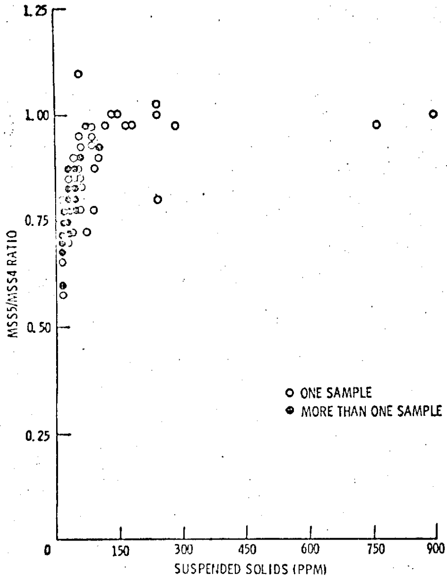
FIGURE 9. MSS5/MSS4 RATIO FROM CCT VS. SUSPENDED SOLIDS FOR 108 WATER SAMPLES FROM 11 ERTS-1 PASSES.
