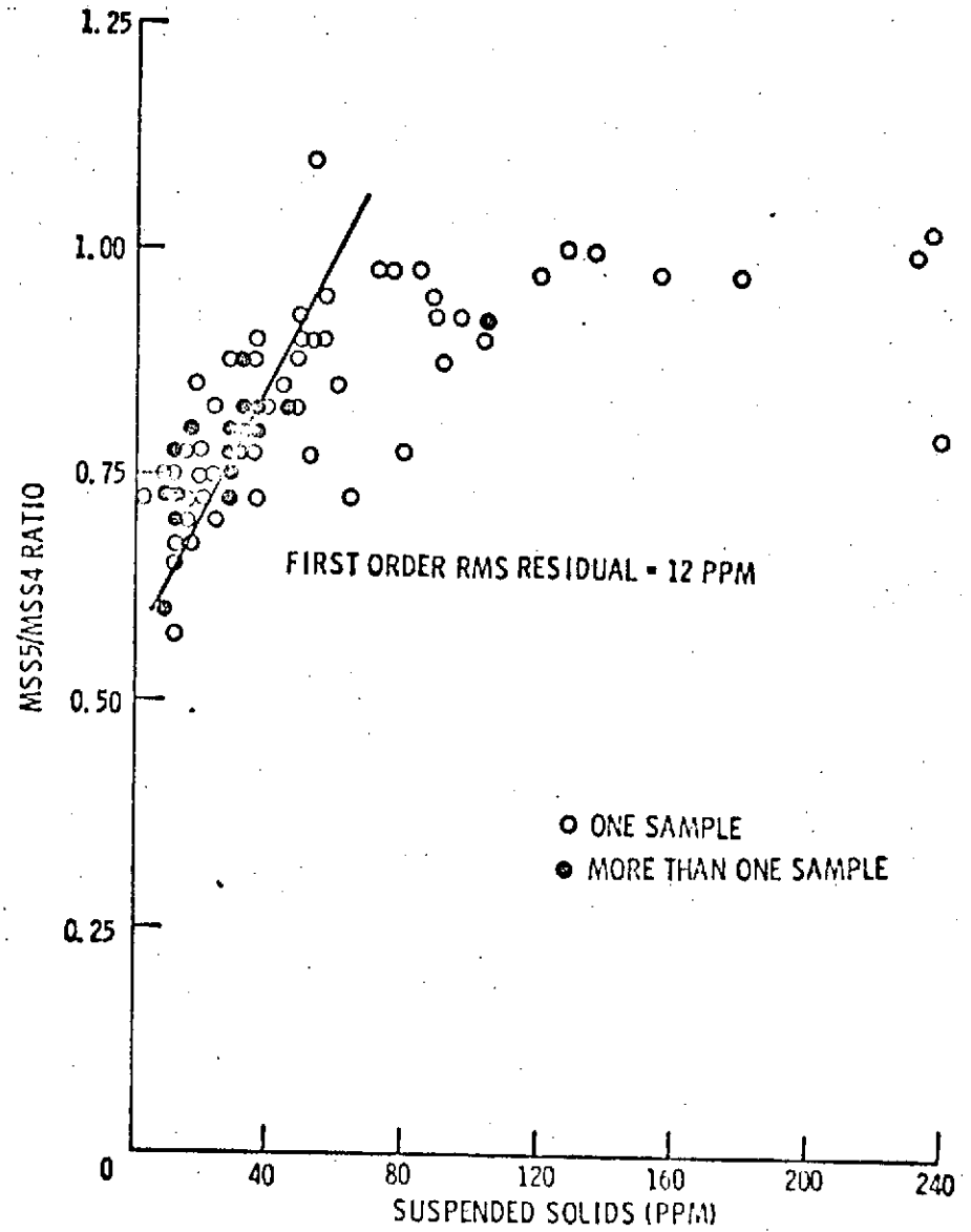
FIGURE 10. MSS5/MSS4 RATIO FROM CCT VS. SUSPENDED SOLIDS FOR 108 WATER SAMPLES FROM 11 ERTS-1 PASSES.
