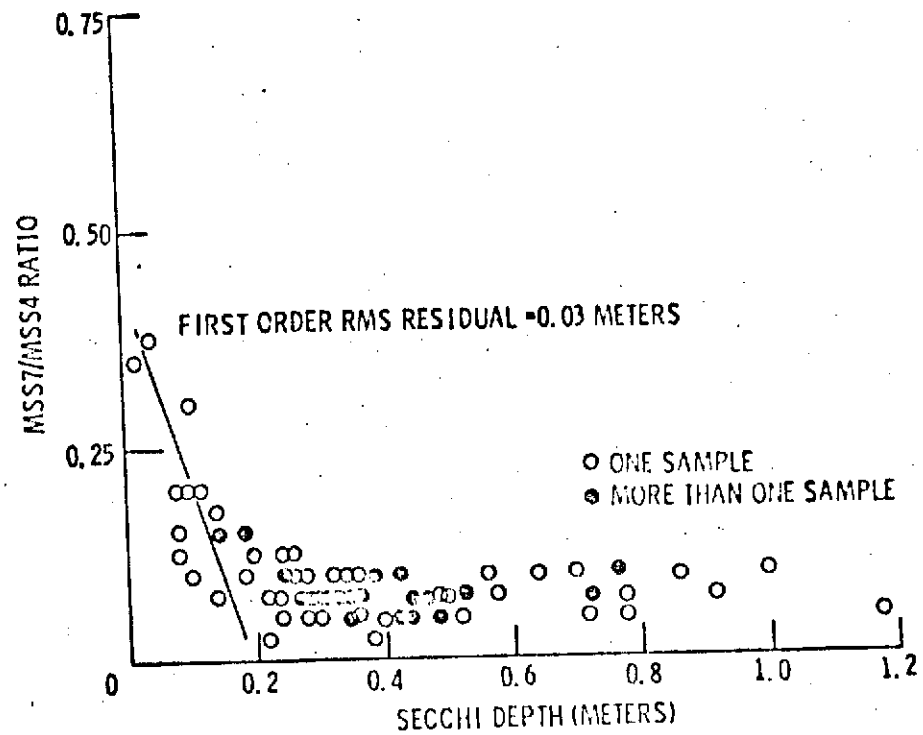
FIGURE 18. MSS7/MSS4 RATIO FROM CCT VS. SECCHI DEPTH FOR 97 SAMPLE STATIONS FROM 10 ERTS-1 PASSES.
