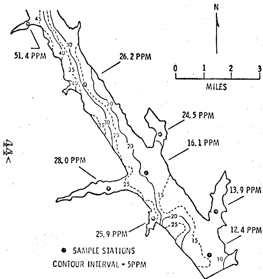
FIGURE 15. SUSPENDED SOLIDS CONTOUR MAP OF TUTTLE CREEK RESERVOIR (AUGUST 14, 1972 ERTS-1 ID NO. 1022-16391-5) DERIVED FROM CCTS (MSS 5) FOR 4 ERTS-1 PASSES.
