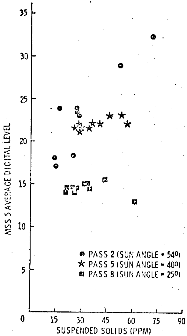
FIGURE 5. MSS5 DIGITAL LEVELS FROM CCT VS. SUSPENDED SOLIDS FOR 28 WATER SAMPLES FROM 3 ERTS-1 PASSES.
