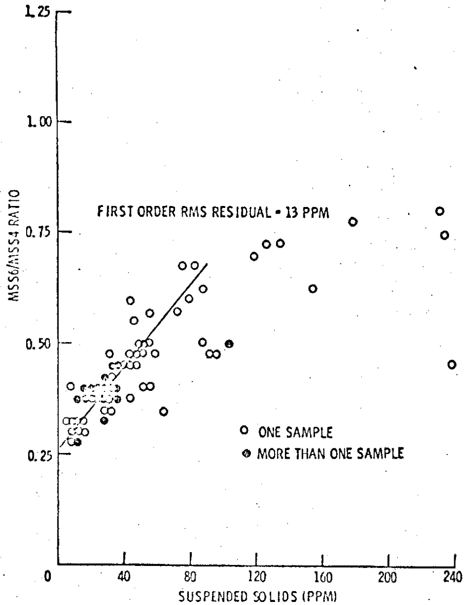
FIGURE 13. MSS6/MSS4 RATIO FROM CCT VS. SUSPENDED SOLIDS FOR 97 WATER SAMPLES FROM 10 ERTS-1 PASSES.
