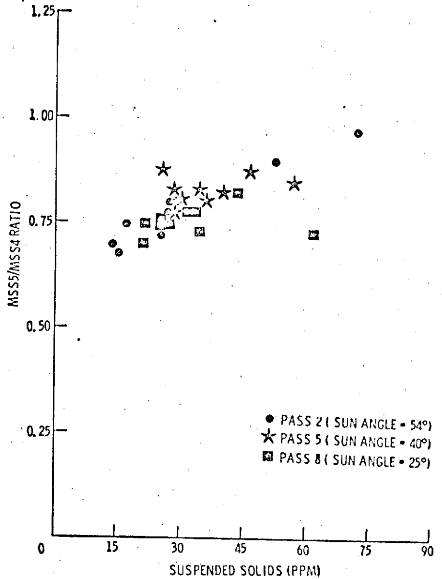
FIGURE 6. MSS5/MSS4 RATIO FROM CCT VS. SUSPENDED SOLIDS FOR 28 WATER SAMPLES FROM 3 ERTS-1 PASSES.
