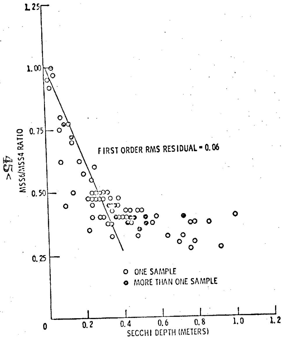
FIGURE 17. MSS6/MSS4 RATIO FROM CCT VS. SECCHI DEPTH FOR 96 SAMPLE STATIONS FROM 10 ERTS-1 PASSES.
