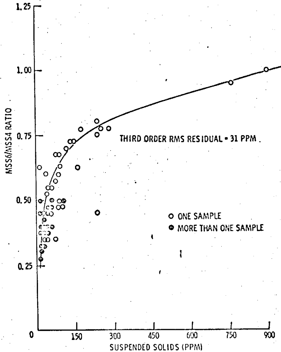
FIGURE 12. MSS6/MSS4 RATIO FROM CCT VS. SUSPENDED SOLIDS FOR 107 WATER SAMPLES FROM 11 ERTS-1 PASSES.
