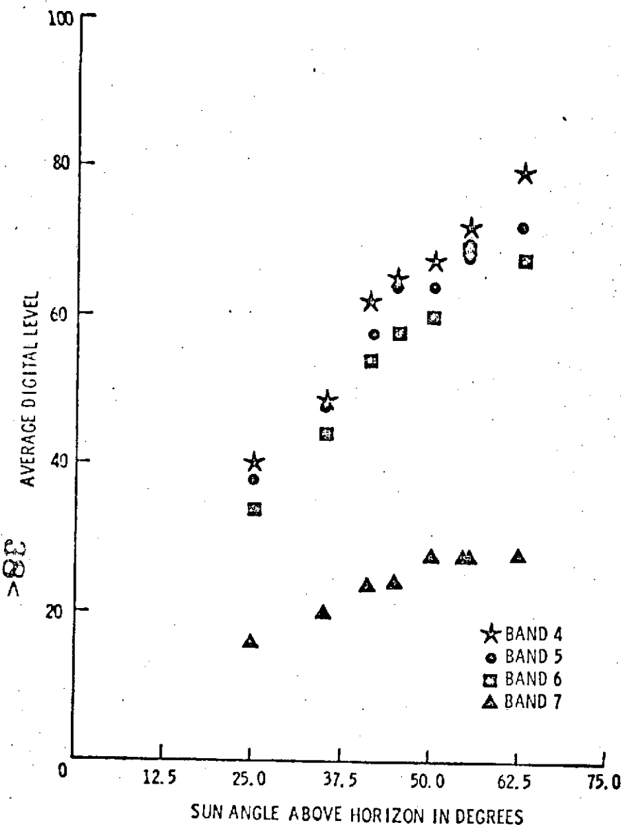
FIGURE 3. MSS DIGITAL LEVELS FROM CCT VS. SUN ANGLE FOR TUTTLE CREEK CONCRETE DAM.
