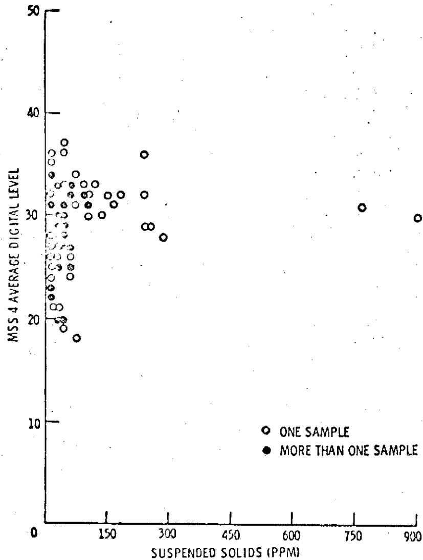
FIGURE 7. MSS 4 DIGITAL LEVEL FROM CCT VS. SUSPENDED SOLIDS FOR 108 WATER SAMPLES FROM 11 ERTS-1 PASSES.
