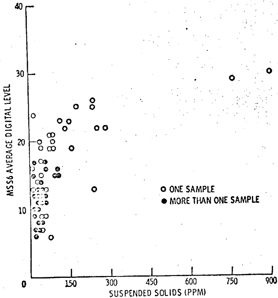
FIGURE 11. MSS6 DIGITAL LEVEL FROM CCT VS. SUSPENDED SOLIDS FOR 108 WATER SAMPLES FROM 11 ERTS-1 PASSES.
