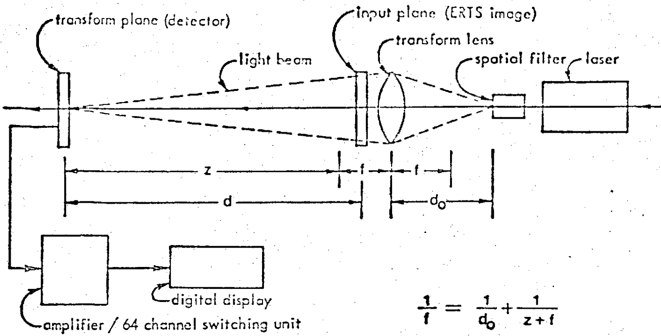
Figure 1. System configuration
