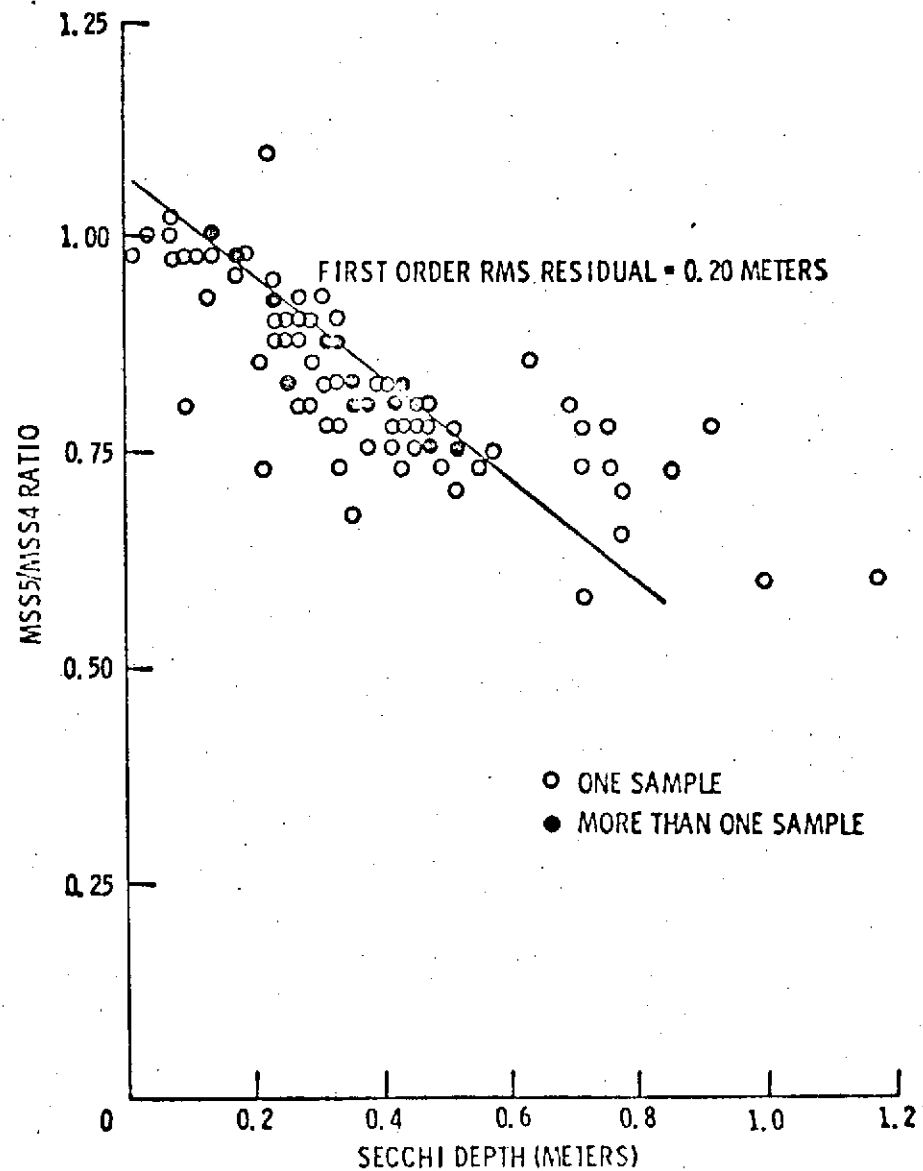
FIGURE 16. MSS5/MSS4 RATIO FROM CCT VS. SECCHI DEPTH FOR 97 SAMPLE STATIONS FROM 10 ERTS-1 PASSES.
