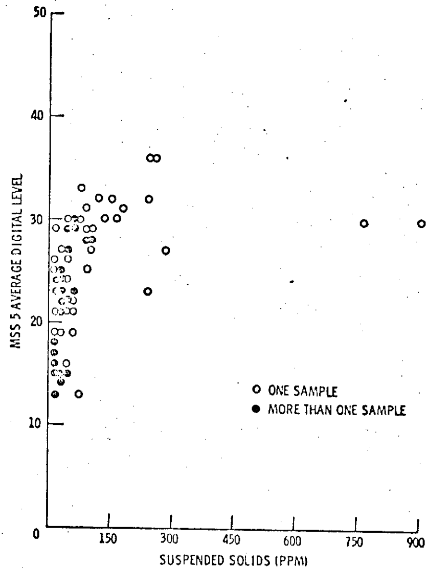
FIGURE 8. MSS 5 DIGITAL LEVEL FROM CCT VS. SUSPENDED SOLIDS FOR 108 WATER SAMPLES FROM 11 ERTS-1 PASSES.
