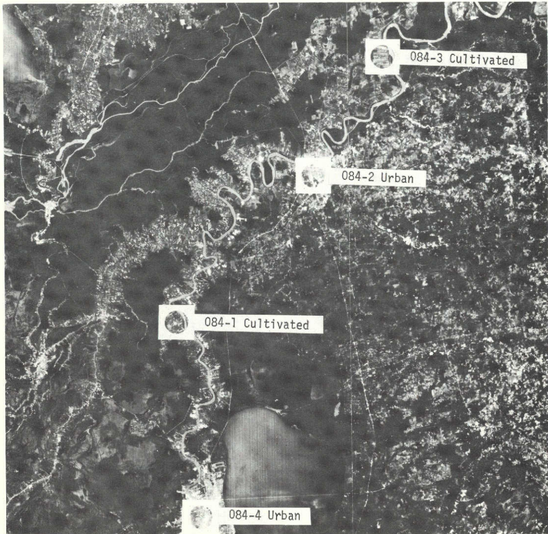
Fig. 4-5 — New Orleans, Louisiana—ERTS image 1070-16037-5
