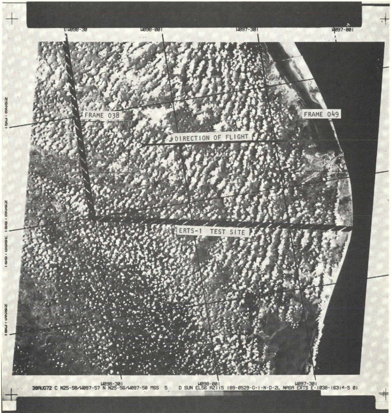
Fig. 2-1 — Annotated ERTS-1 image 1038-16314
