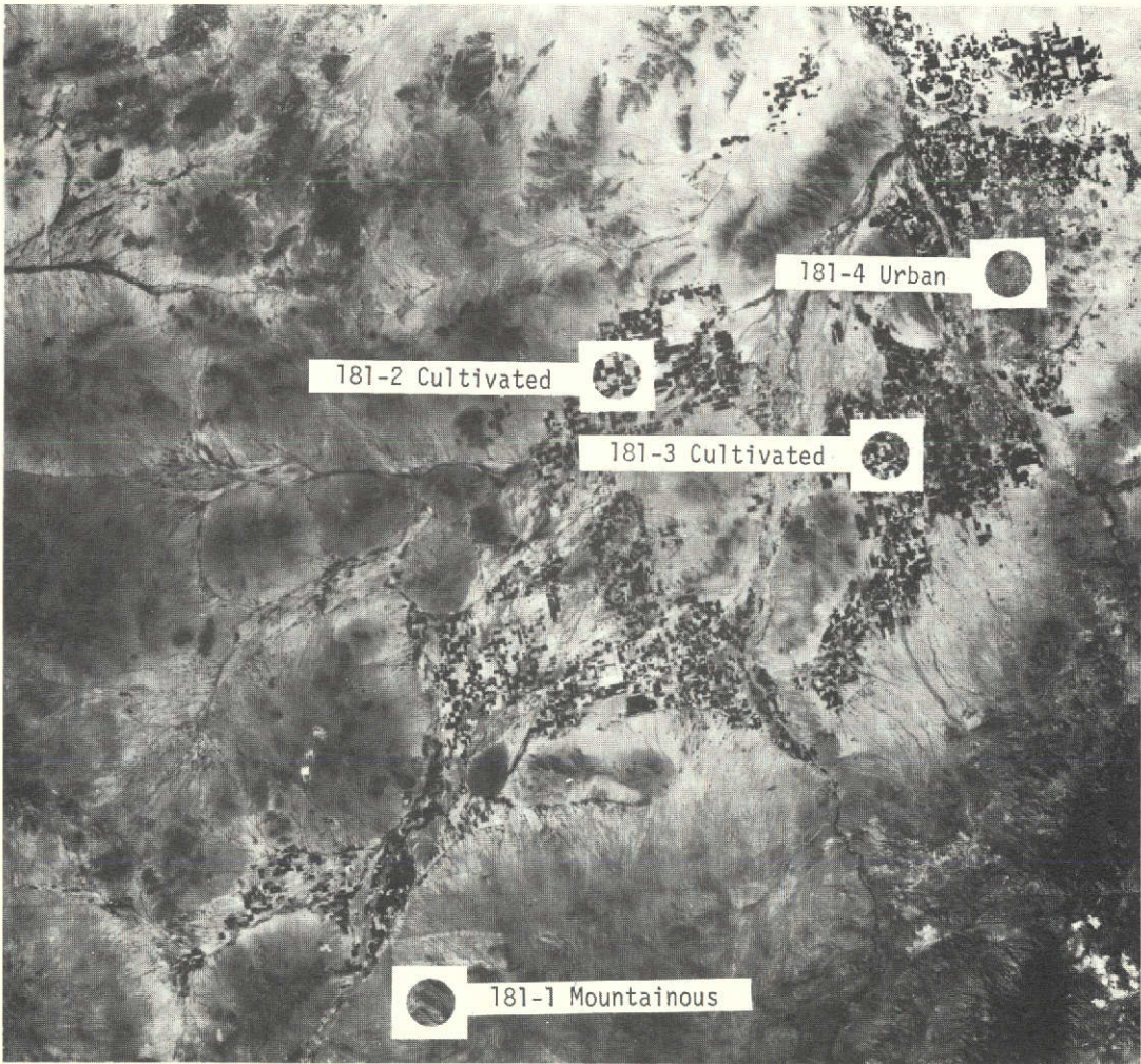
Fig. 4-13 — Phoenix, Arizona—ERTS image 1031-17325-5
