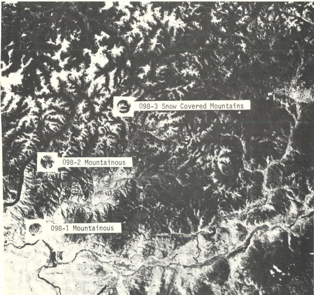
Fig. 4-7 -- Cascade Mountains, Washington--ERTS image 1041-18253-5
