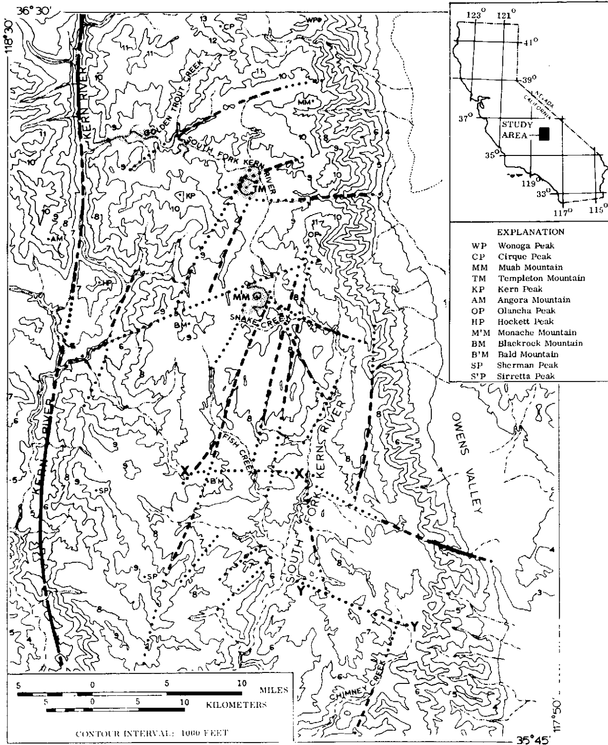
Figure 2: Interpretation of major lineament systems visible in the ERTS-1 image of Figure 1. Location names follow the code shown at right. Topography is from the AMS Fresno and Bakersfield 1° x 2° quadrangles. See text for more detailed discussion.
