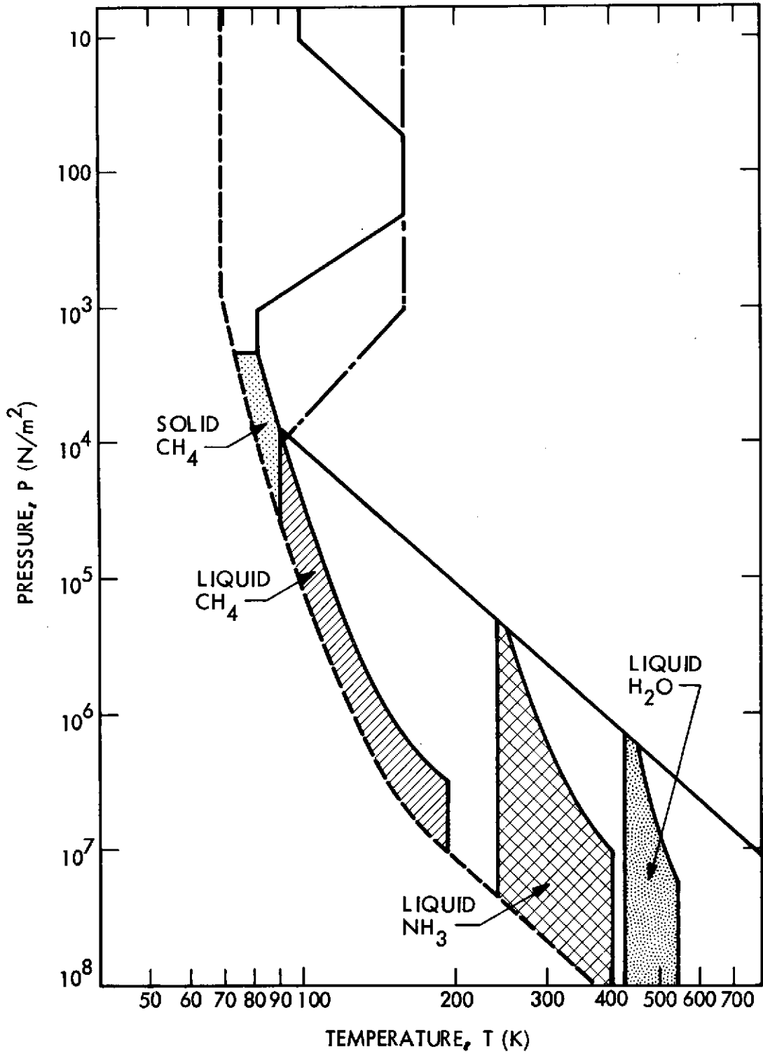
Figure 4. Pressure-temperature domains for various potential condensates in Titan's atmosphere. Portions of the engineering model profiles are reproduced from fig. 2.
