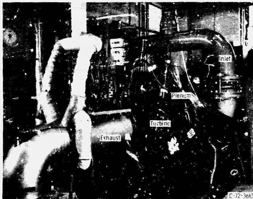
Figure 7. - Test facility.
