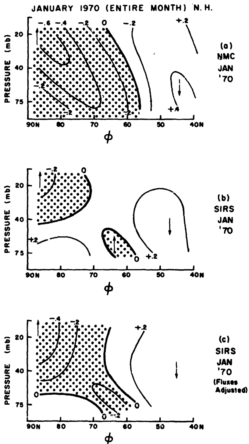
Fig. 3. Zonally-averaged vertical motion patterns for the N. H. for January 1970. Units: mb/day. Stippled area denotes area of ascent.
