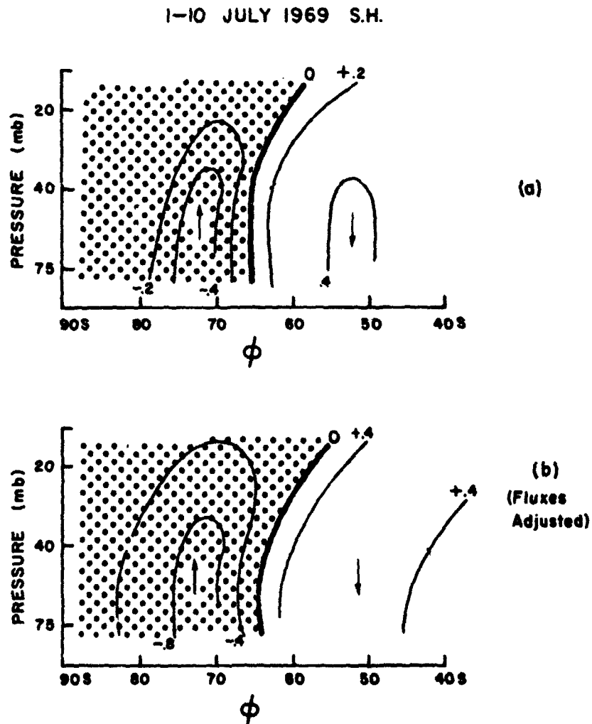
Fig. 5. Zonally-averaged vertical motion patterns for the S. H. for the period 1-10 July 1969, during a minor mid-winter warming. Units: mb/day.
