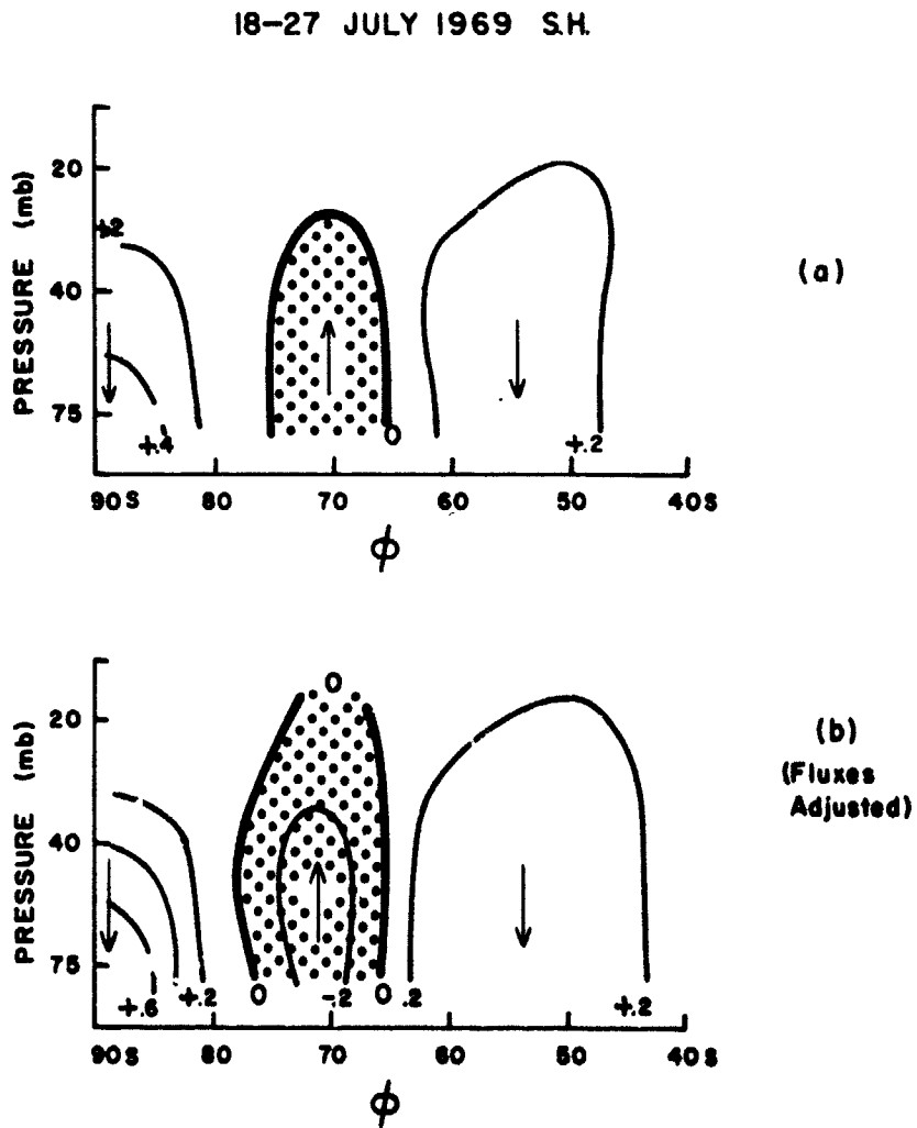
Fig. 6. Zonally-averaged vertical motion patterns for the S. H. for the period 18-27 July 1969, a quiet period. Units: mb/day.
