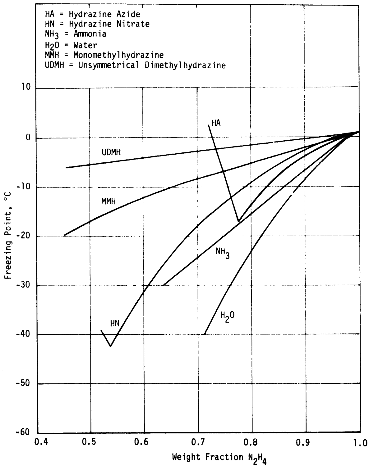
Figure 4. Freezing Point Temperatures of Pure Binary Monopropellants
