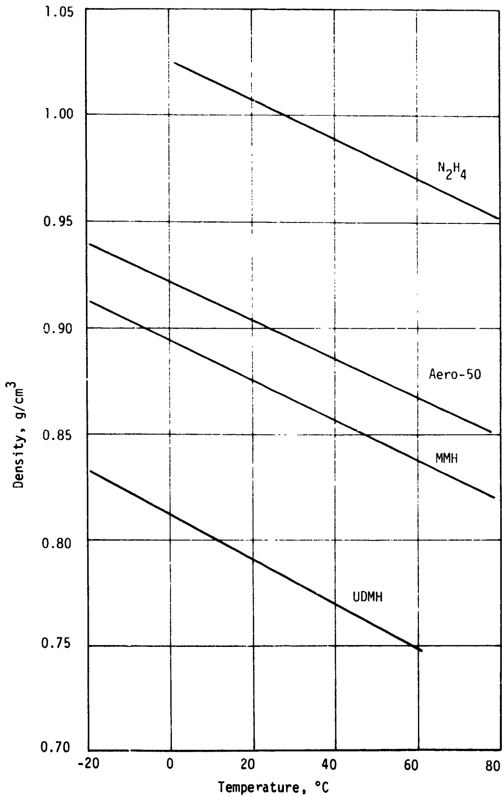
Figure 1. Density of Pure Monopropellants as a Function of Temperature
