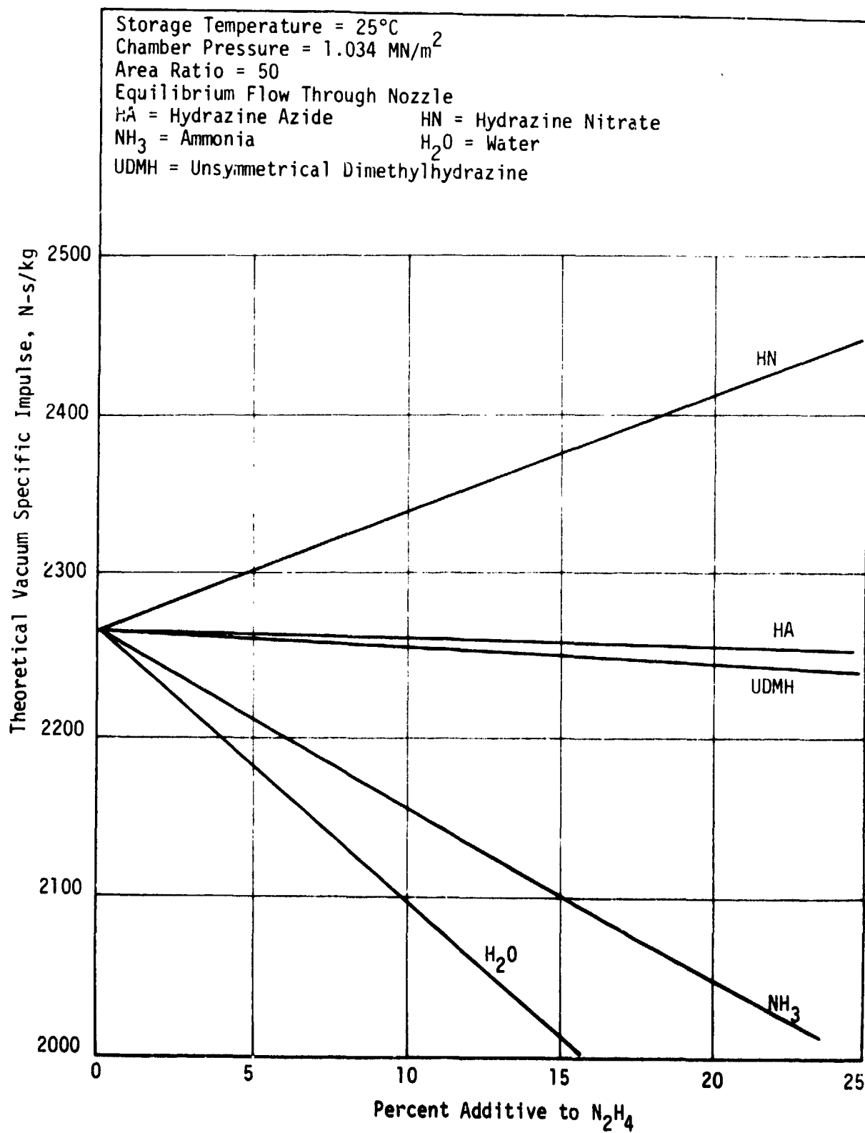
Figure 6. Theoretical Vacuum Specific Impulse of Pure Binary Monopropellants
