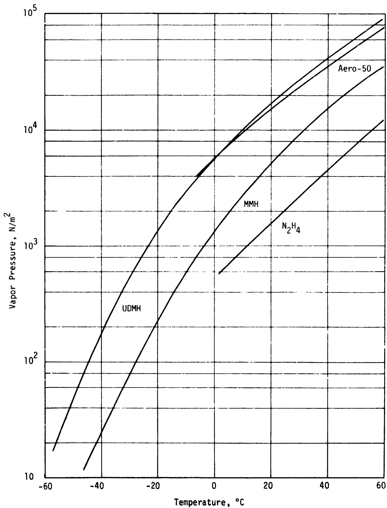
Figure 2. Vapor Pressure of Pure Monopropellants as a Function of Temperature
