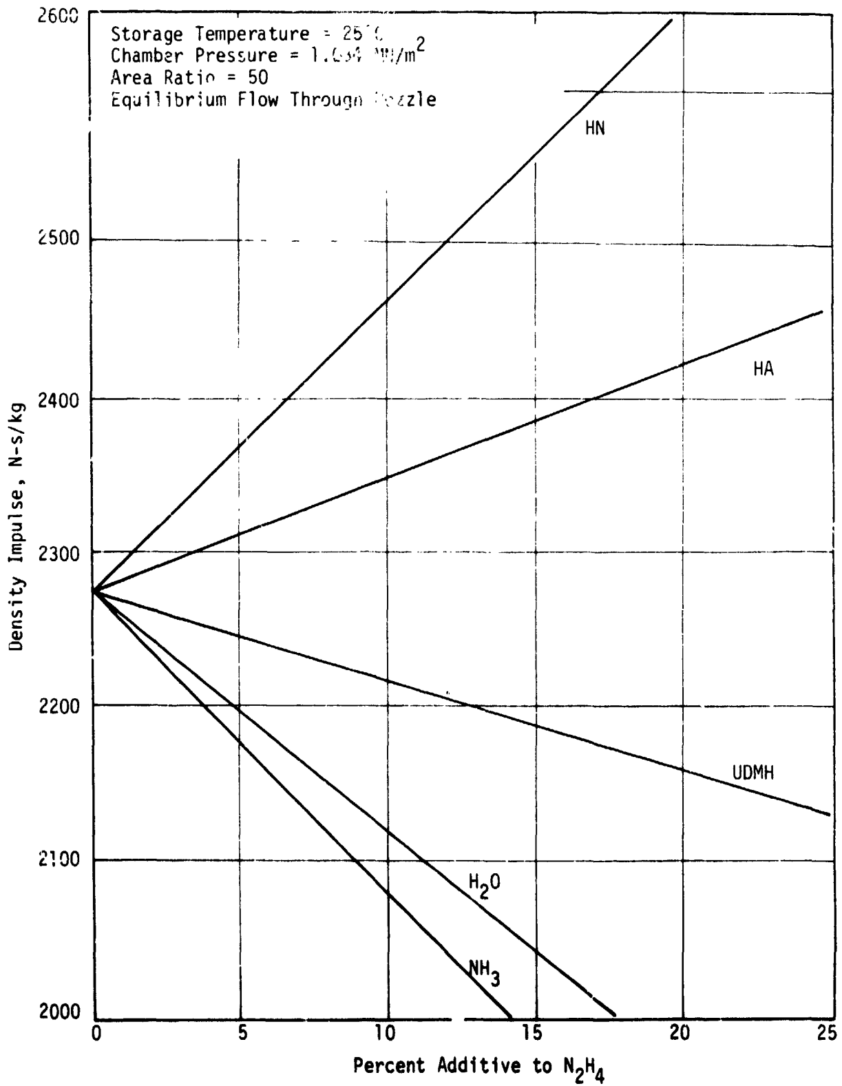
Figure 7. Density Impulse of Pure Binary Monopropellants
