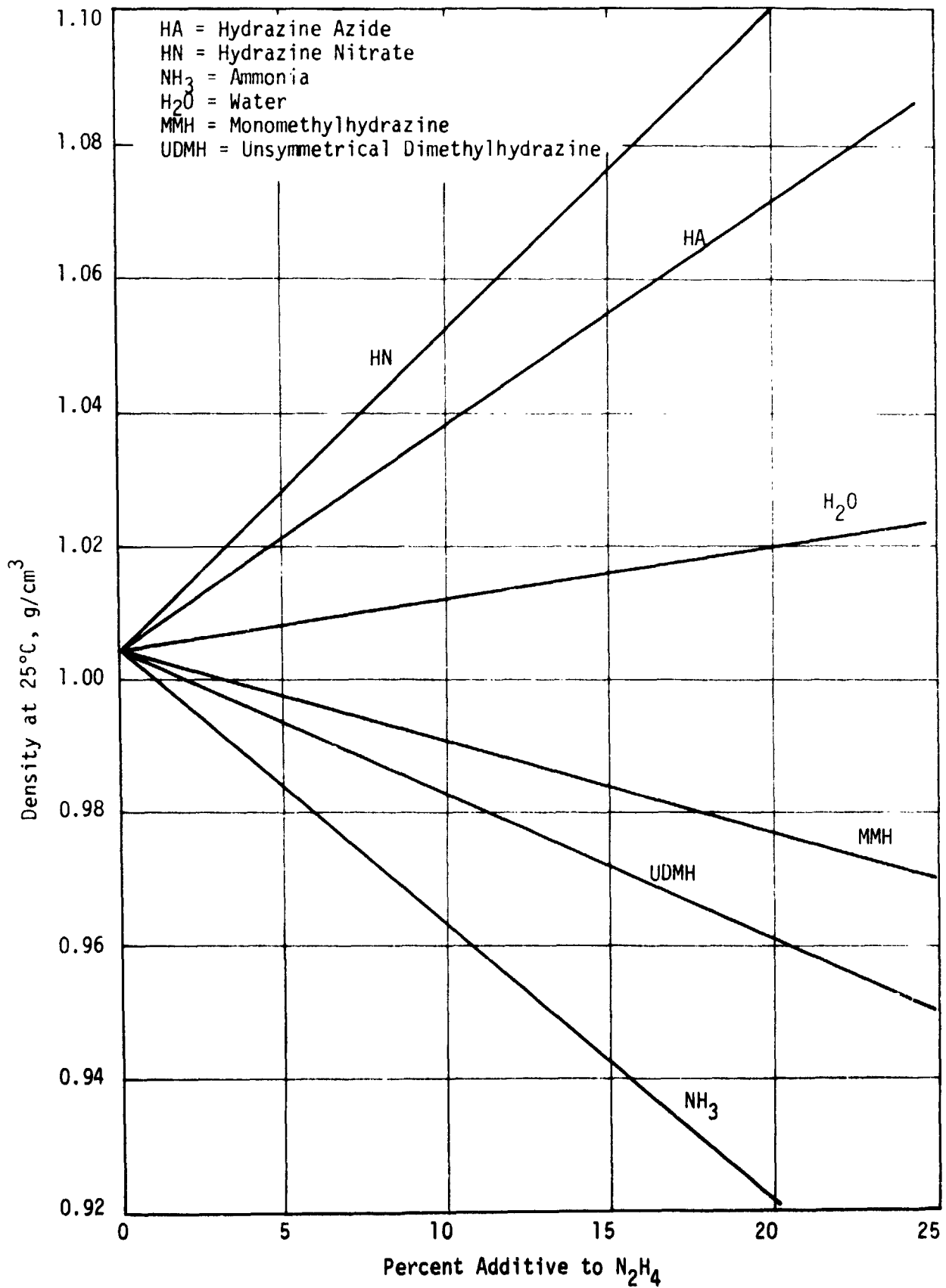
Figure 5. Density of Pure Binary Monopropellants
