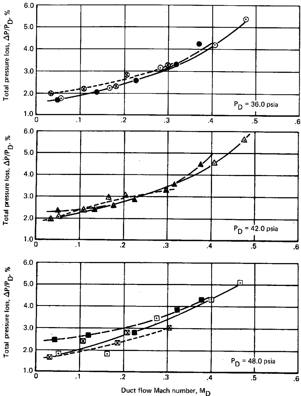
FIGURE 48.—ADDITIONAL PRESSURE LOSS CHARACTERISTICS—DNA-5
