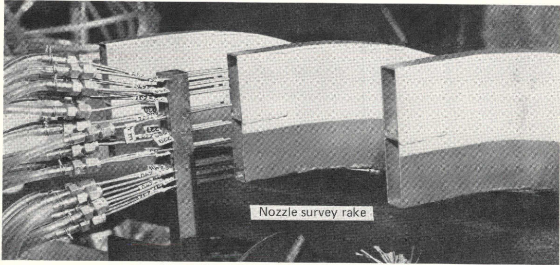
NOZZLE ASSEMBLY FRONT VIEW
