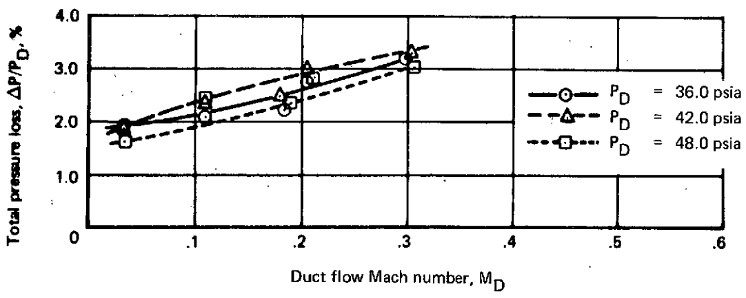
FIGURE 47.—PRESSURE LOSS CHARACTERISTICS—DNA-5
