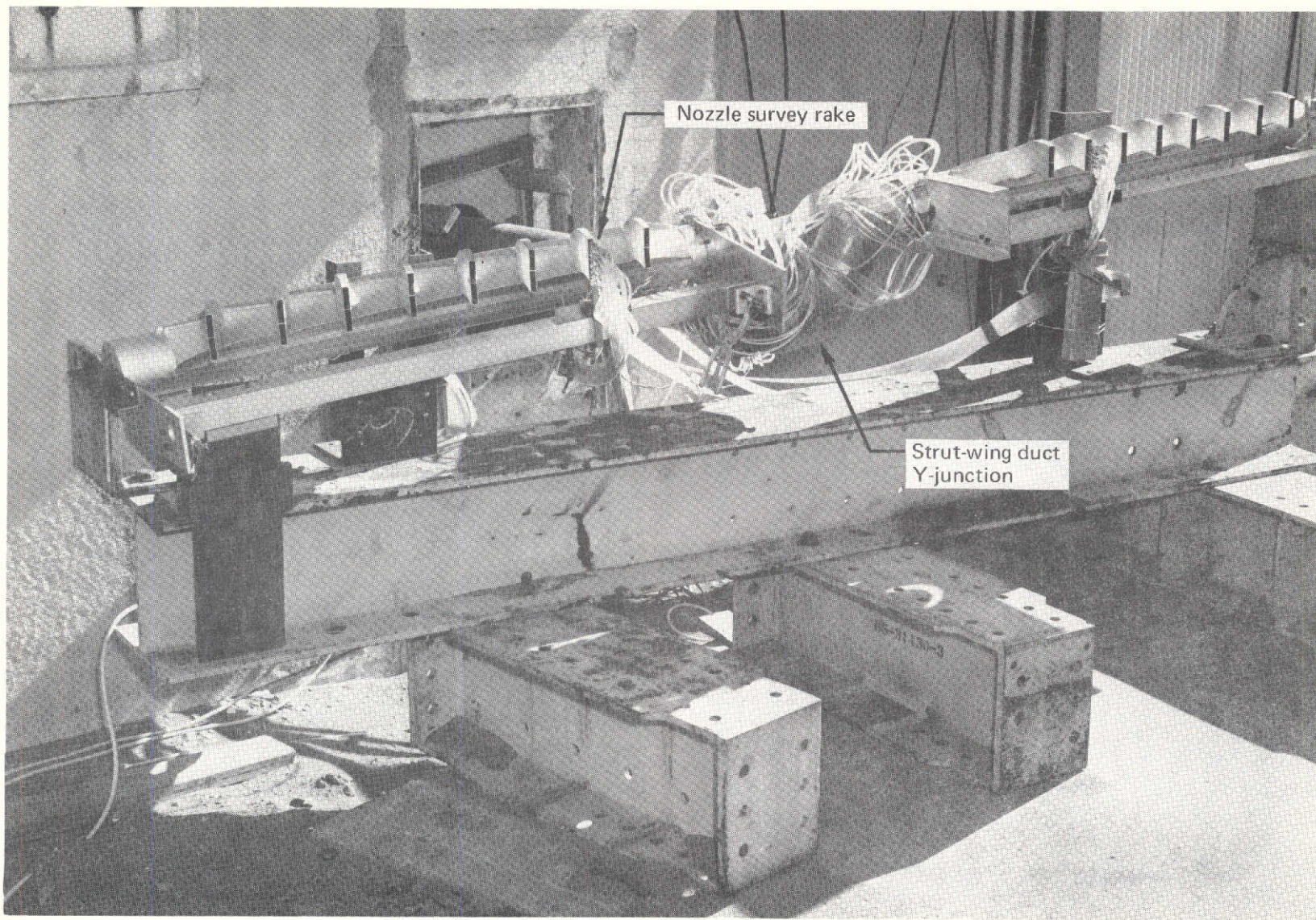
FIGURE 13.—TEST SETUP
