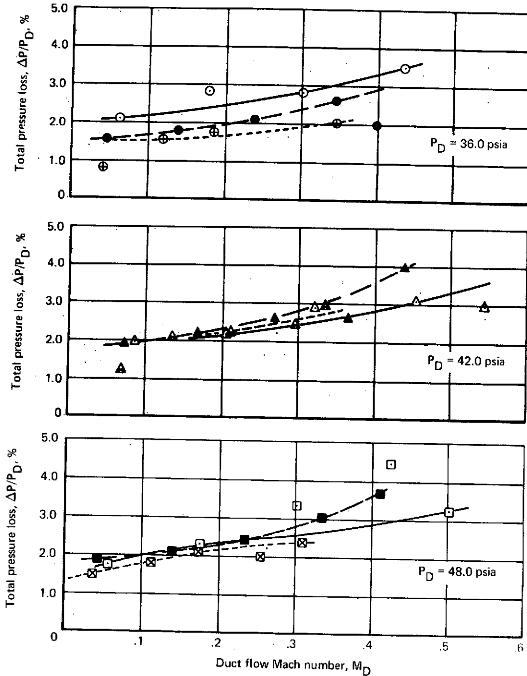
FIGURE 42.—ADDITIONAL PRESSURE LOSS CHARACTERISTICS—DNA-2
