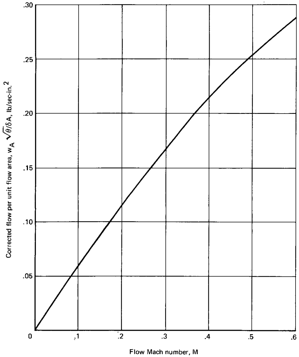
FIGURE 9.—CORRECTED FLOW PER UNIT FLOW AREA VERSUS FLOW MACH NUMBER
