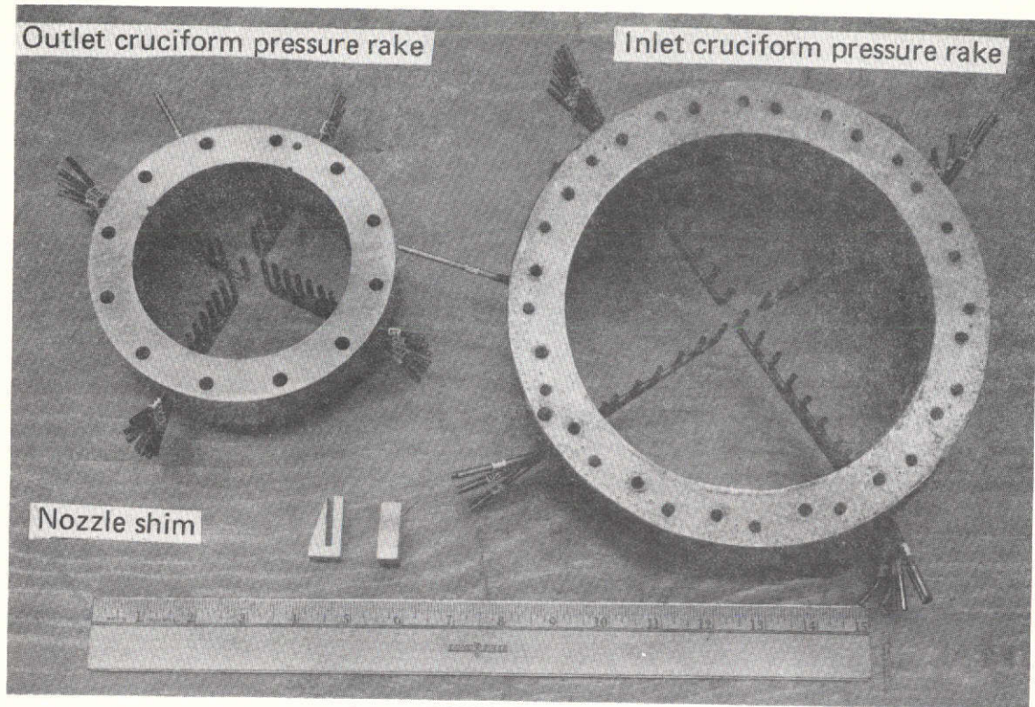
PRESSURE RAKES
