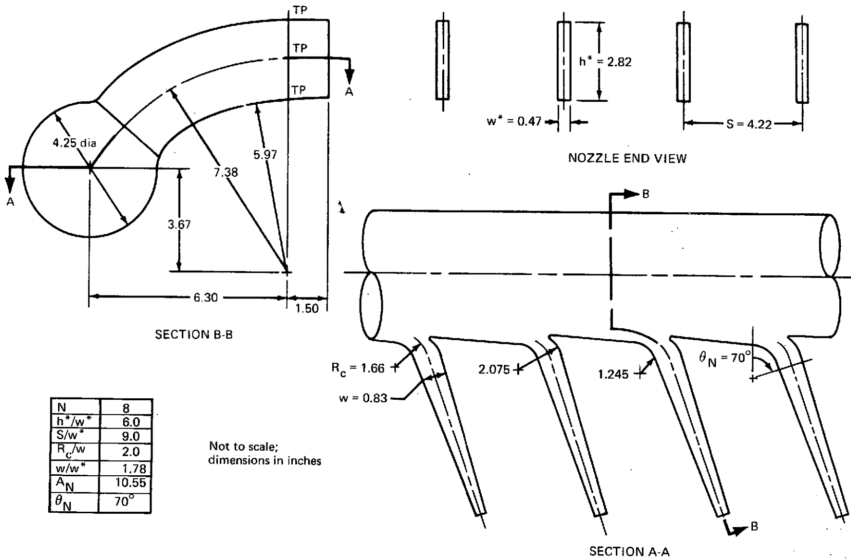
FIGURE 25.—WING-DUCT-LOBE NOZZLE ASSEMBLY DNA-6 DESIGN DETAILS
