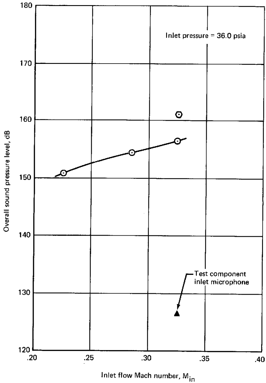
FIGURE 7.—OUTLET DUCT OVERALL SOUND PRESSURE LEVEL
