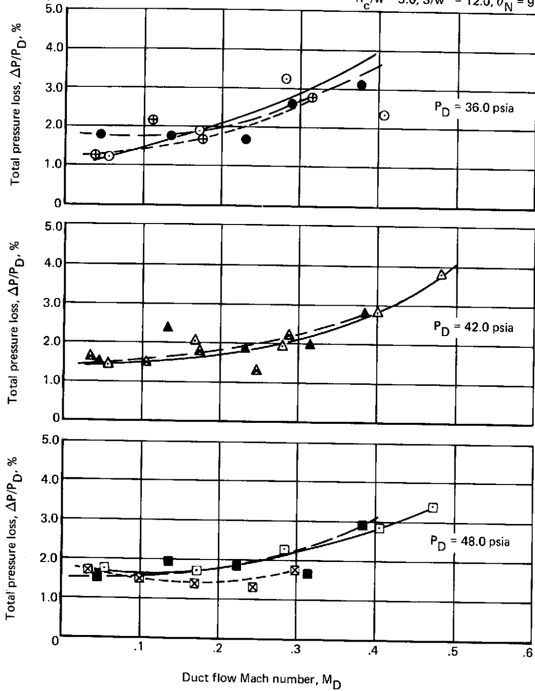
FIGURE 40.—ADDITIONAL PRESSURE LOSS CHARACTERISTICS—DNA-1
