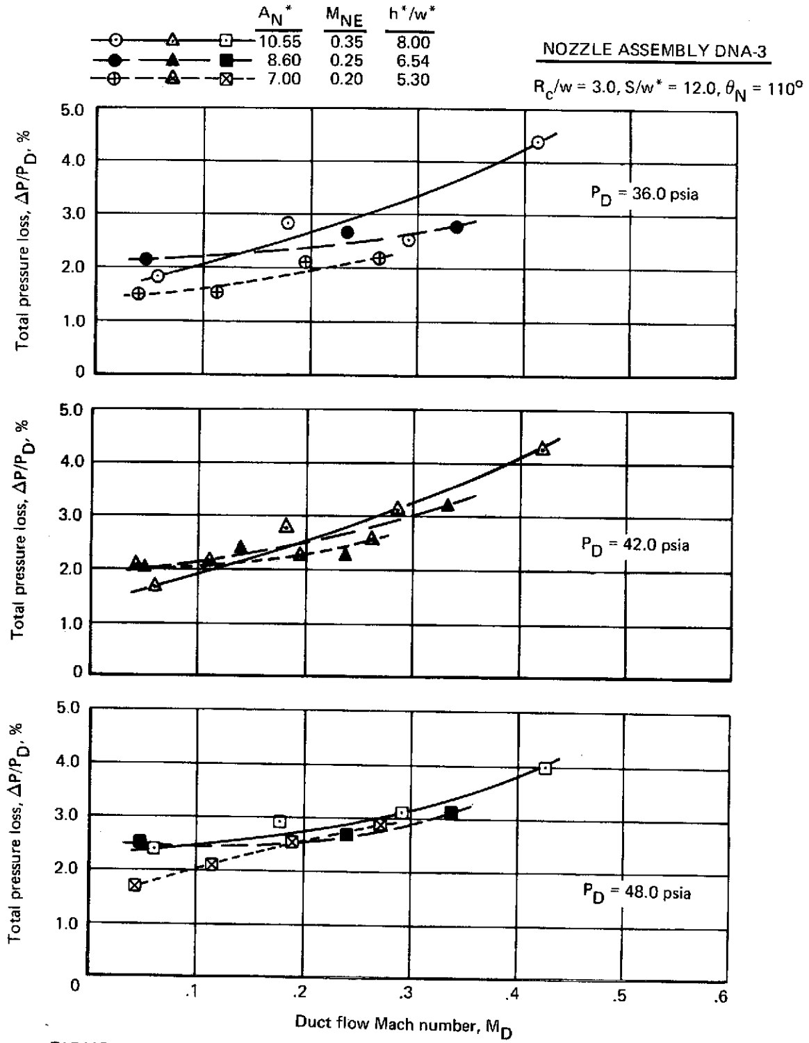
FIGURE 44.—ADDITIONAL PRESSURE LOSS CHARACTERISTICS—DNA-3
