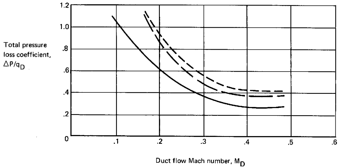
FIGURE 4.—PRESSURE LOSS, SET I LOBE NOZZLE ASSEMBLIES
