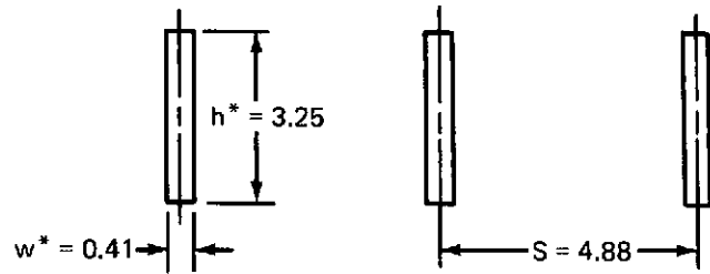
NOZZLE END VIEW
