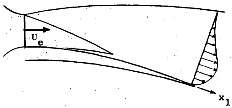
(b) Coanda Surface.
