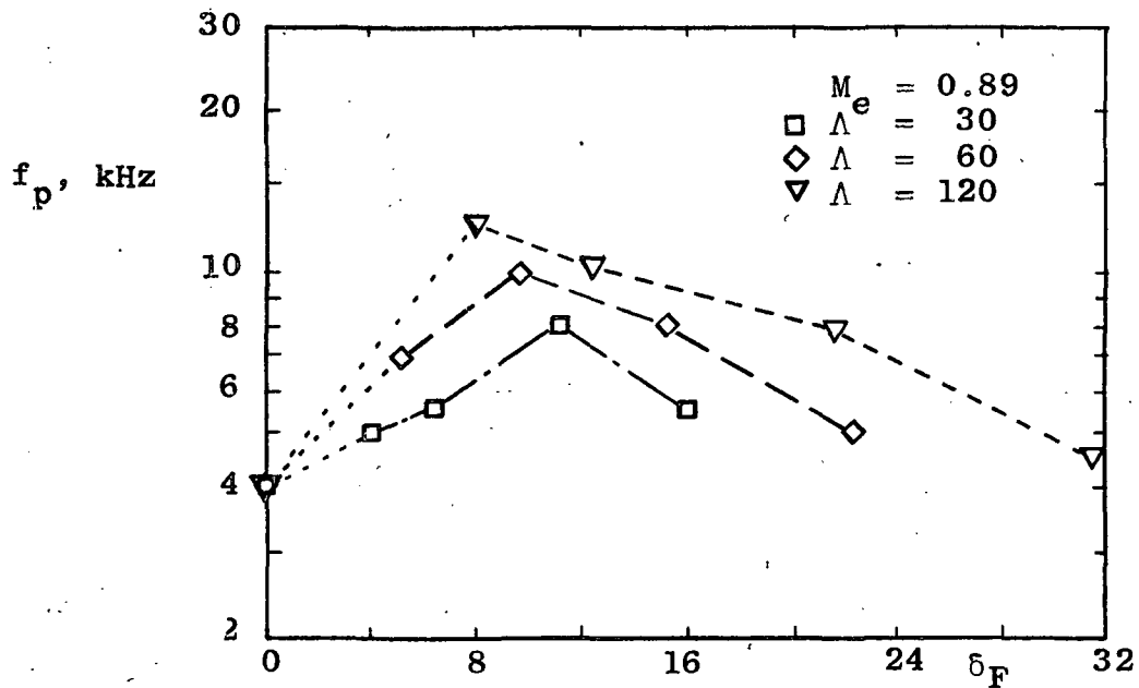
(b) Peak Frequency Versus Dimensionless Flap Length.
