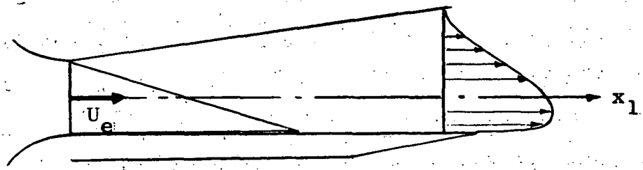
(a) Jet Flap Tested in this Study.
