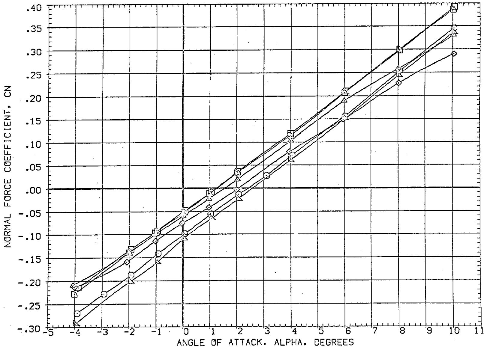
FIG 23 EFFECT OF ORBITER AND SRM PLUMES ON ELEVON AND RUDDER POWER, BETA=0.0 (A)MACH = 1.60
