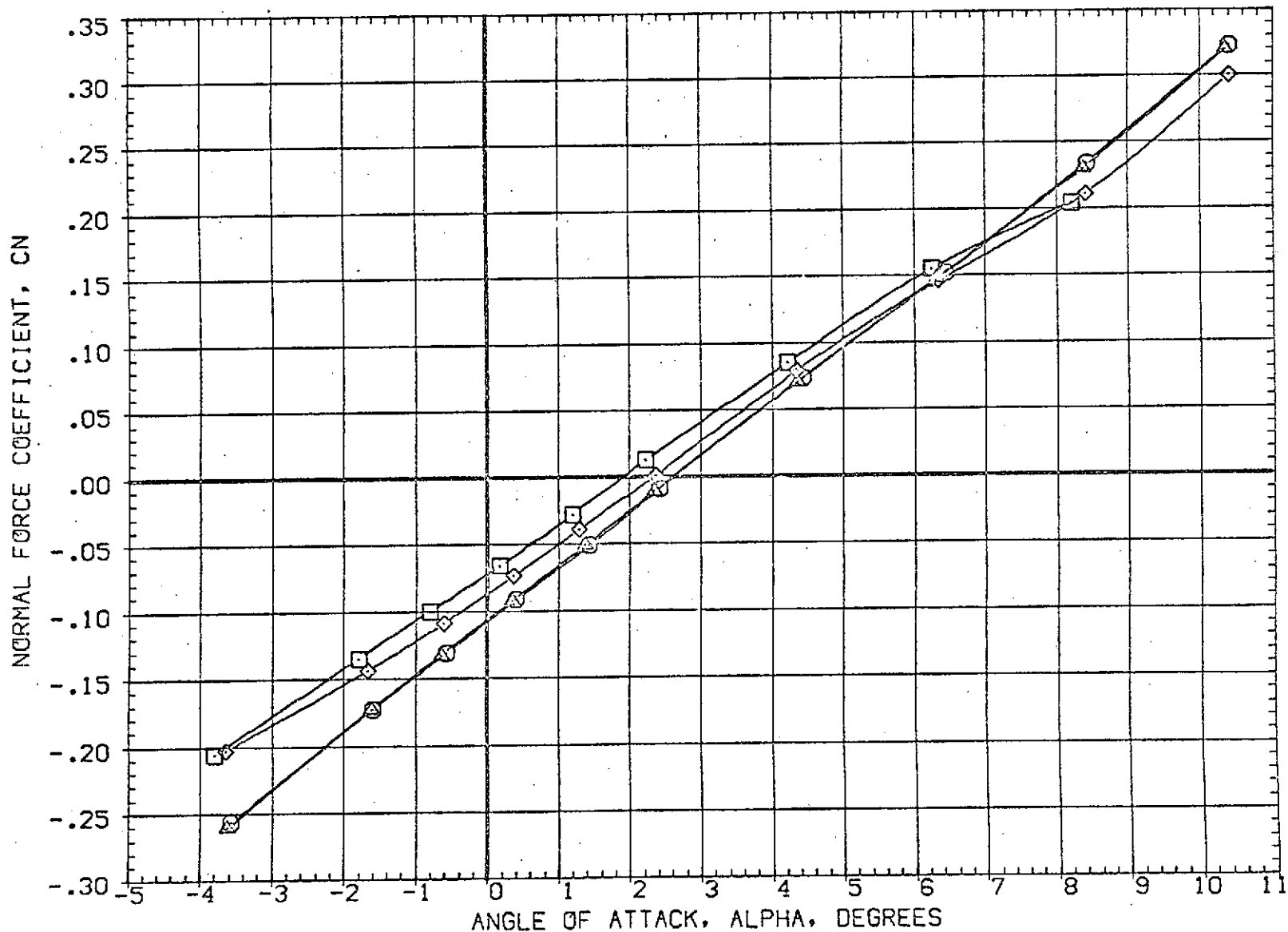
FIG 10 EFFECT OF ORBITER AND SRM PLUMES ON LONGITUDINAL CHARACTERISTICS, BETA=0 (B)MACH = 1.98
