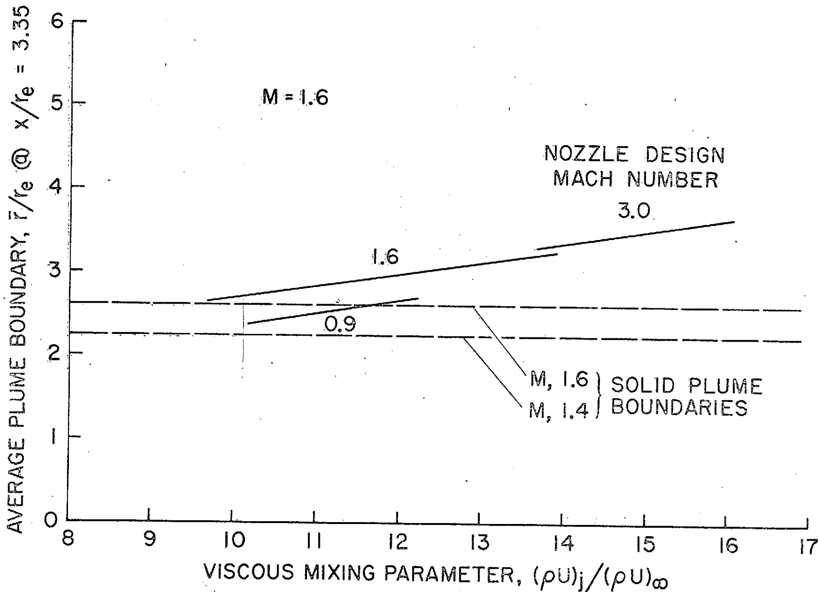
Figure 6. - Variation of the average gaseous SRM plume shape with the viscous mixing parameter at a given distance from the nozzle exit.
