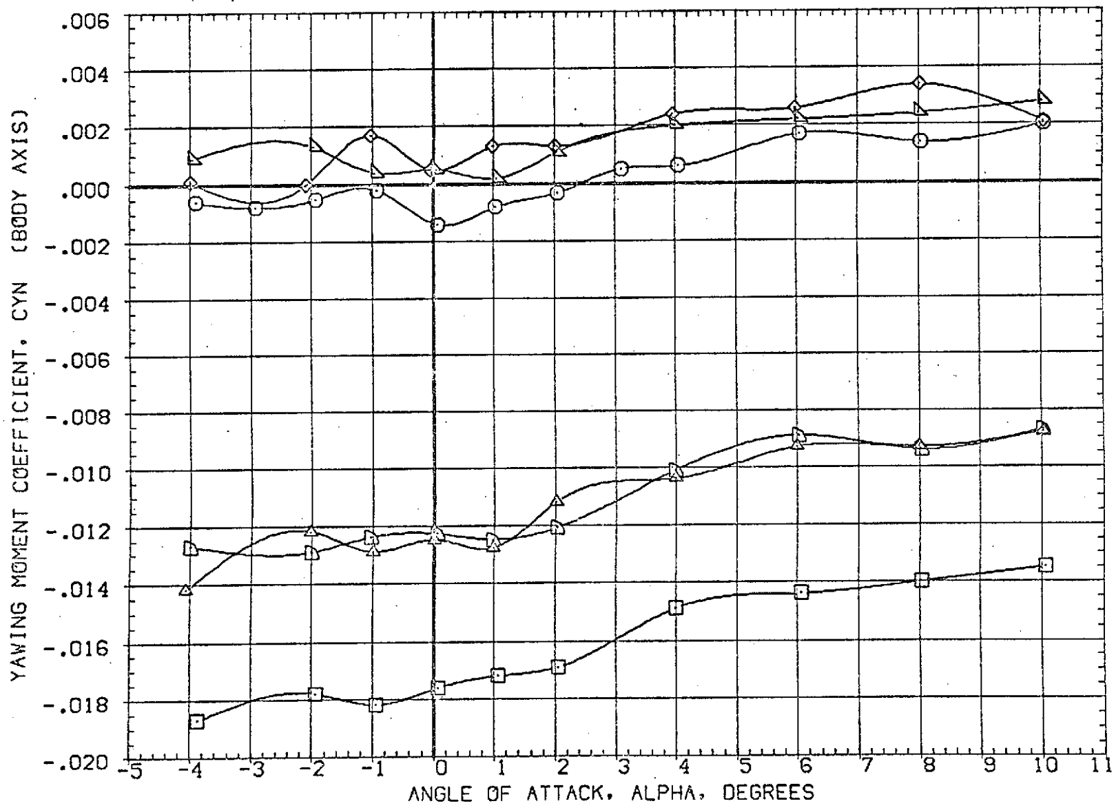
FIG 23 EFFECT OF ORBITER AND SRM PLUMES ON ELEVON AND RUDDER POWER, BETA=0.0 (A)MACH = 1.60 PAGE 189
