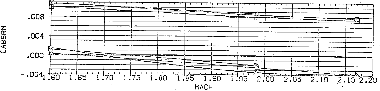
FIG 17 EFFECT OF PLUMES ON ELEVON AND RUDDER POWER, BETA=0.0
