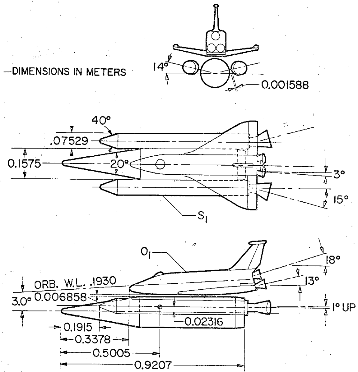
(a) O40A Integrated vehicle
