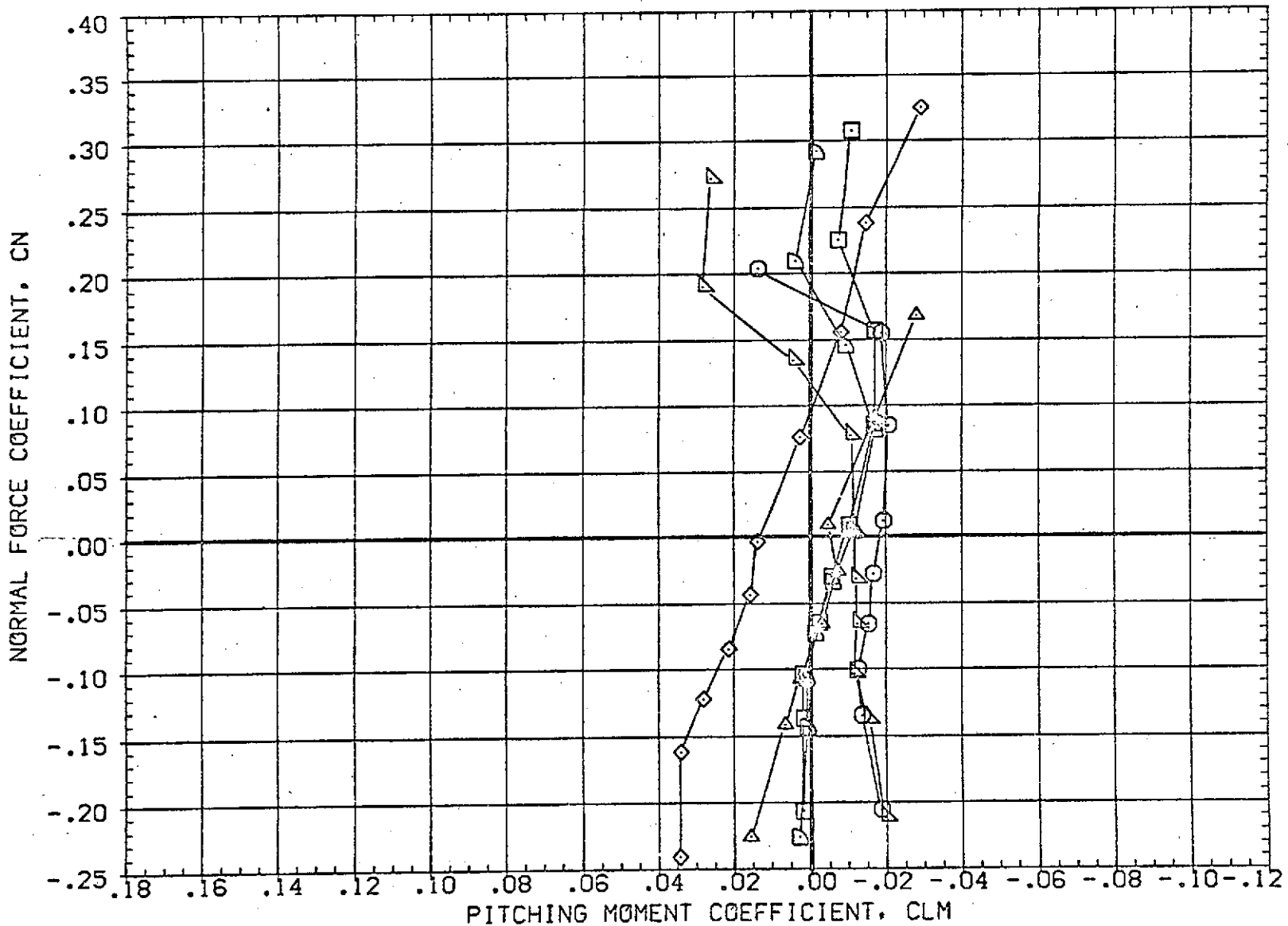
FIG 21 EFFECT OF PLUME SIZE ON ELEVON AND RUDDER POWER, BETA=0.40
