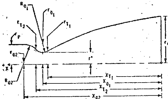
M = 1.6 Nozzle
