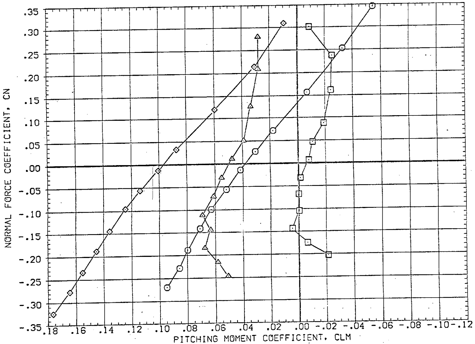
FIG 14 PLUME EFFECTS WITH AND WITHOUT OMS (A) MACH = 1.60
