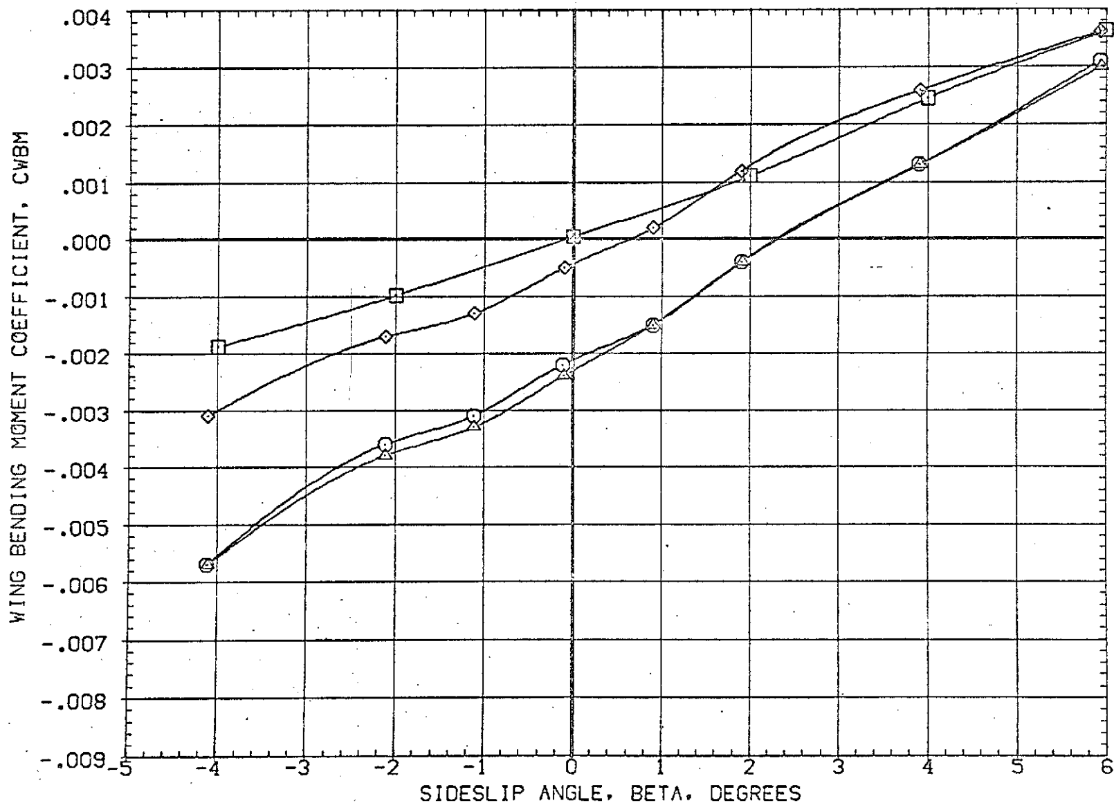
FIG 11 EFFECT OF ORBITER AND SRM PLUMES ON LATERAL CHARACTERISTICS, ALPHA=0.0
