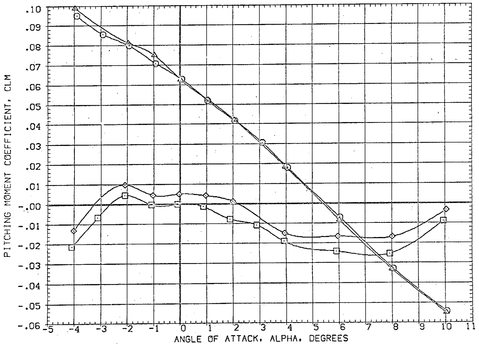
FIG 10 EFFECT OF ORBITER AND SRM PLUMES ON LONGITUDINAL CHARACTERISTICS, BETA=0 (A) MACH = 1.60 PAGE 32
