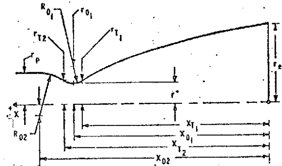
M = 2.0 Nozzle
