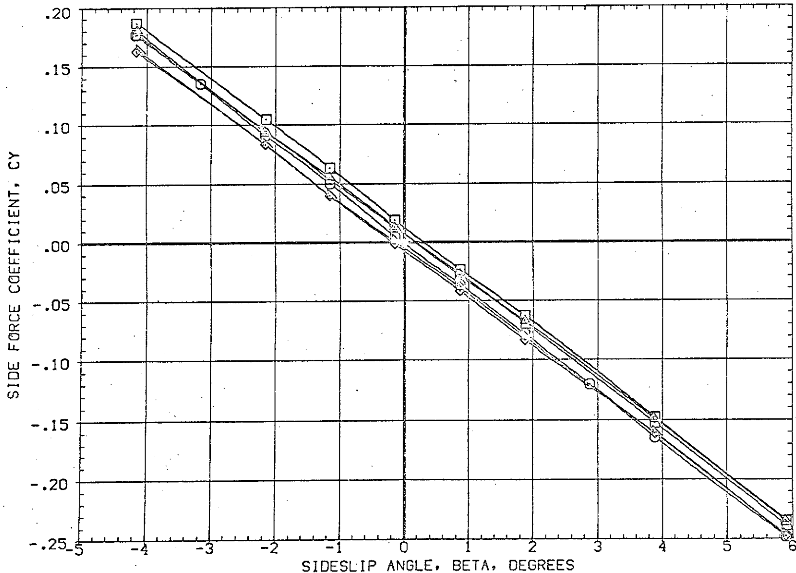
FIG 24 EFFECT OF ORBITER AND SRM PLUMES ON ELEVON AND RUDDER POWER, ALPHA=0.0 (A)MACH = 1.60
