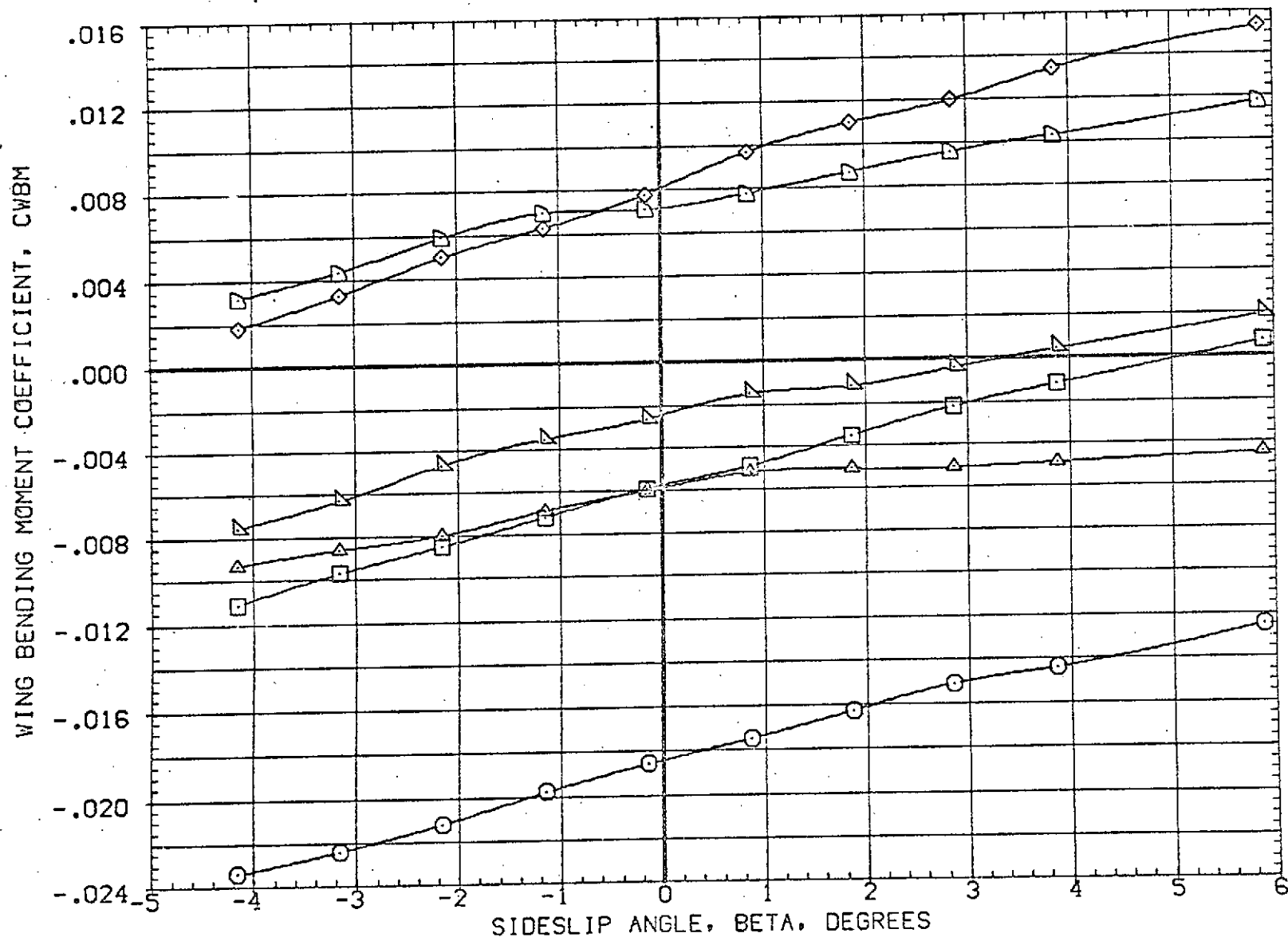
FIG 15 EFFECT OF ALPHA ON LATERAL CHARACTERISTICS WITH PLUMES OMS ON (A) MACH = 1.60
