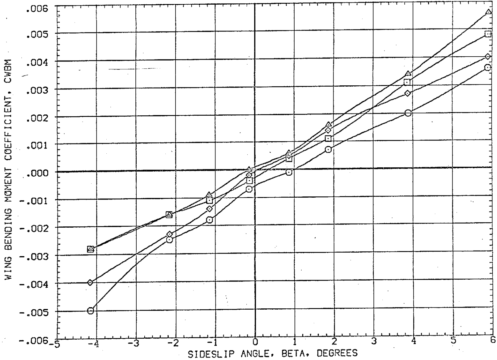
FIG 13 COMPARISON OF CONTROL EFFECTIVENESS WITH GASEOUS AND SOLID SRM PLUMES (A) MACH = 1.60
