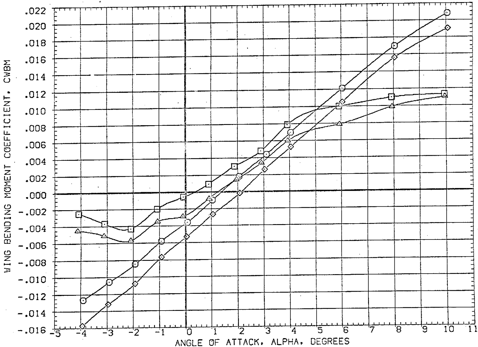
FIG 14 PLUME EFFECTS WITH AND WITHOUT OMS (A)MACH = 1.60
