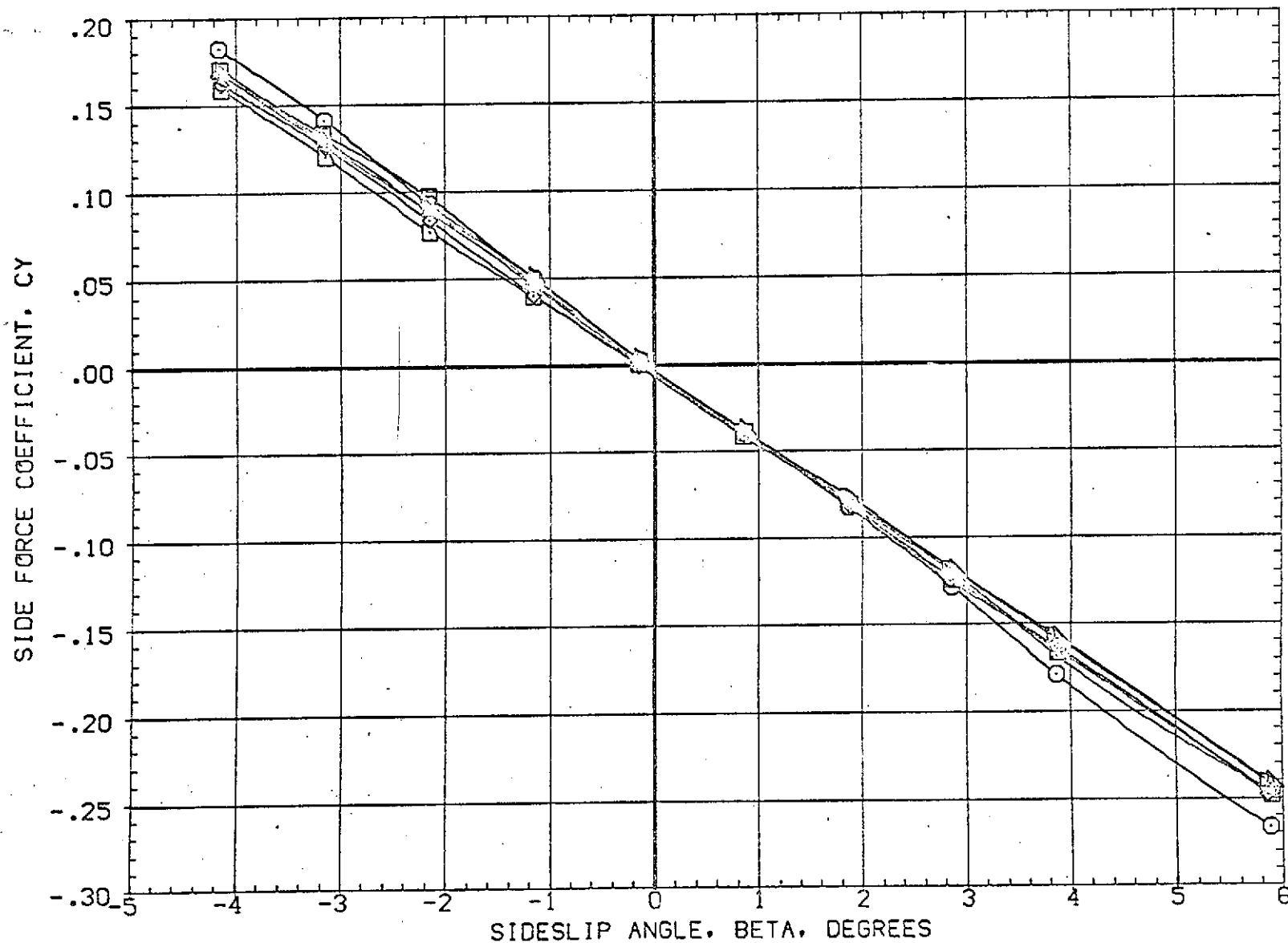
FIG 15 EFFECT OF ALPHA ON LATERAL CHARACTERISTICS WITH PLUMES CMS ON
