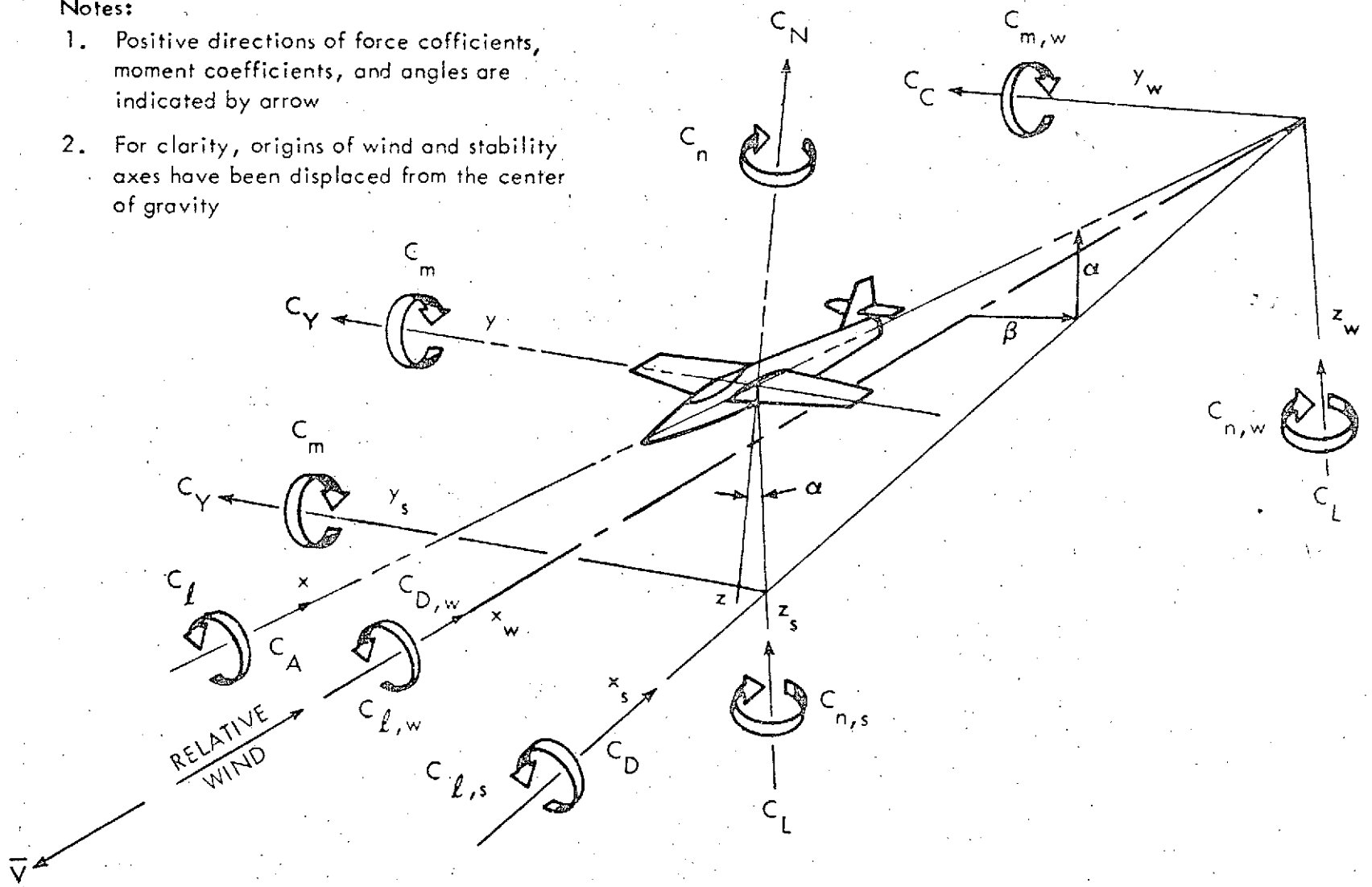
Figure 1. - Axis Systems.
