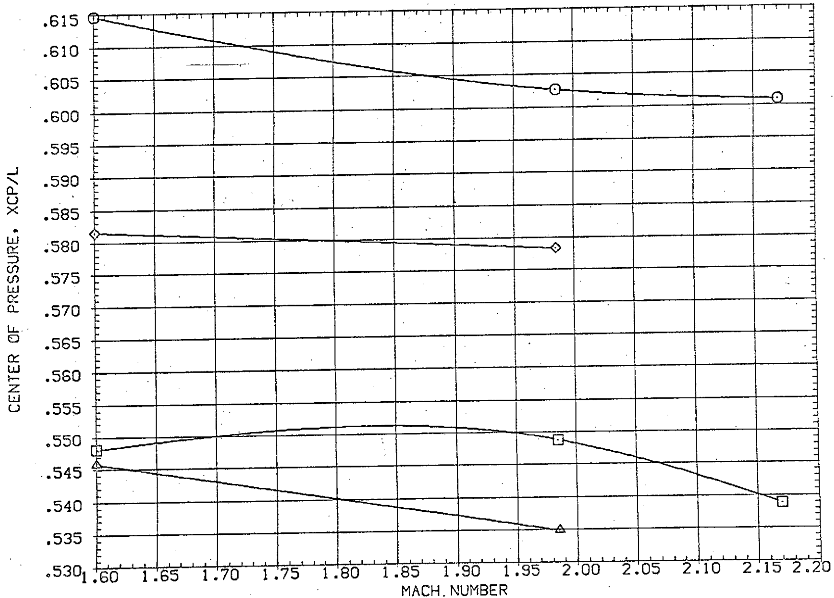
FIG 7 EFFECT OF PLUME SIZE ON LONGITUDINAL CHARACTERISTICS
