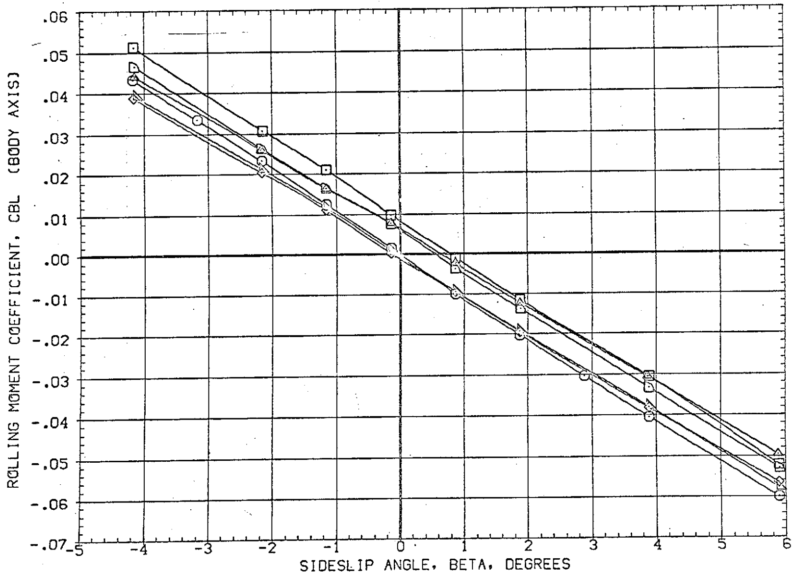
FIG 24 EFFECT OF ORBITER AND SRM PLUMES ON ELEVON AND RUDDER POWER, ALPHA=0.0 (A)MACH = 1.60
