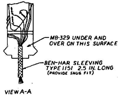
Figure 5. Titanium Blade Instrumentation.
