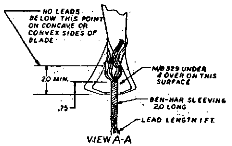
Figure 4. Composite Blade Instrumentation.
