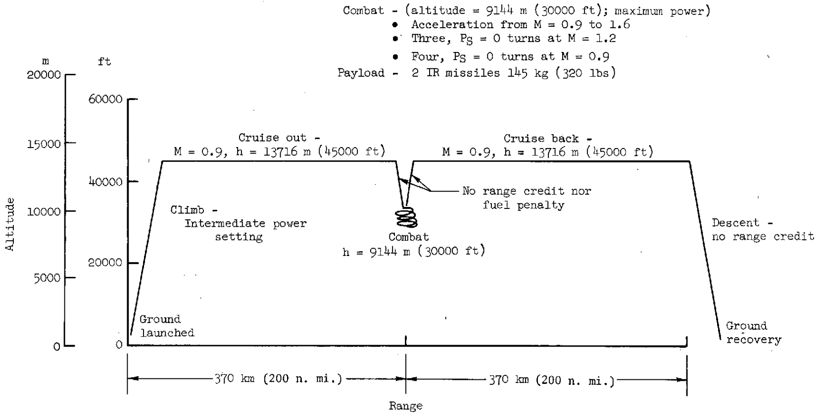
Figure 1.- Nominal mission.
