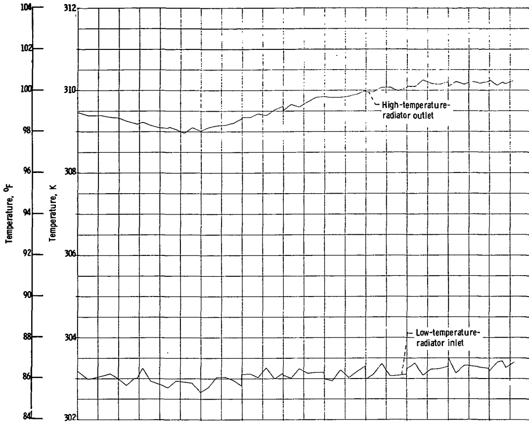
(c) On high-temperature-radiator fluid outlet temperature and on low-temperature-radiator fluid inlet temperature.
