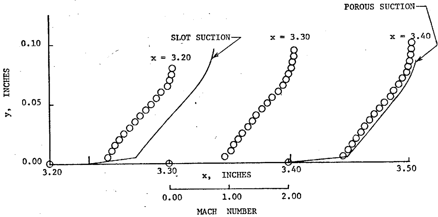
(b) 5.0 PER CENT BLEED RATE
