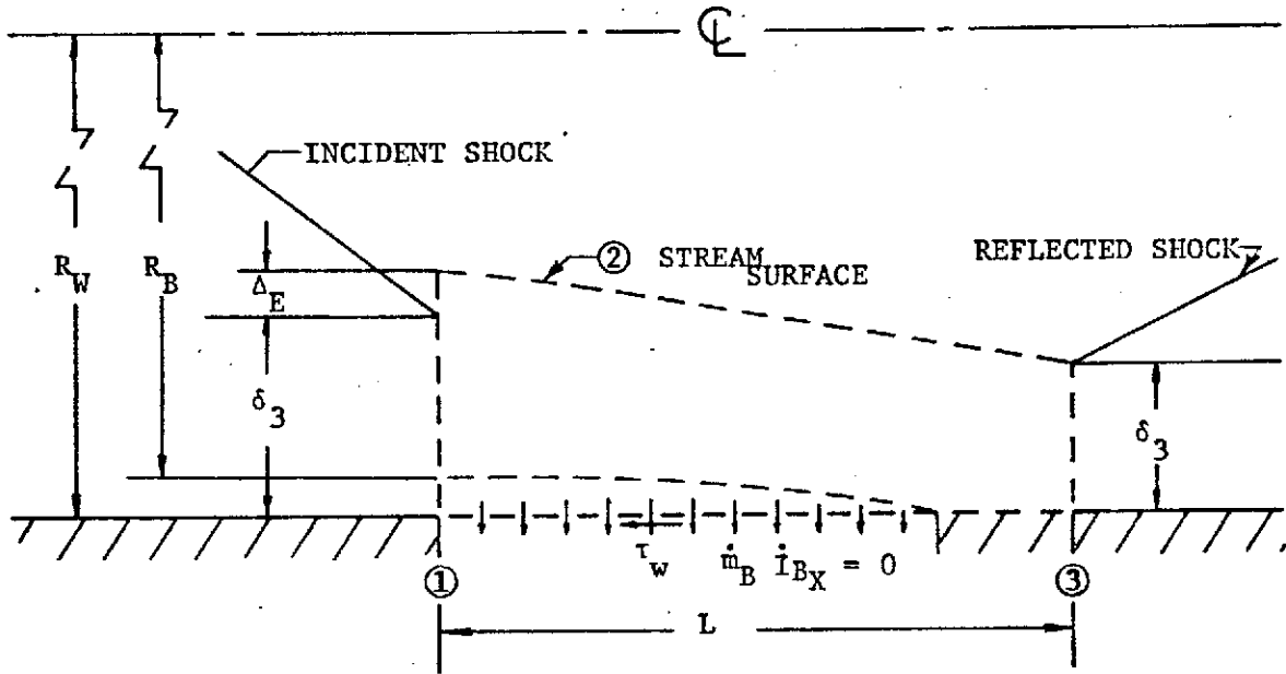
(a) POROUS WALL BLEED
