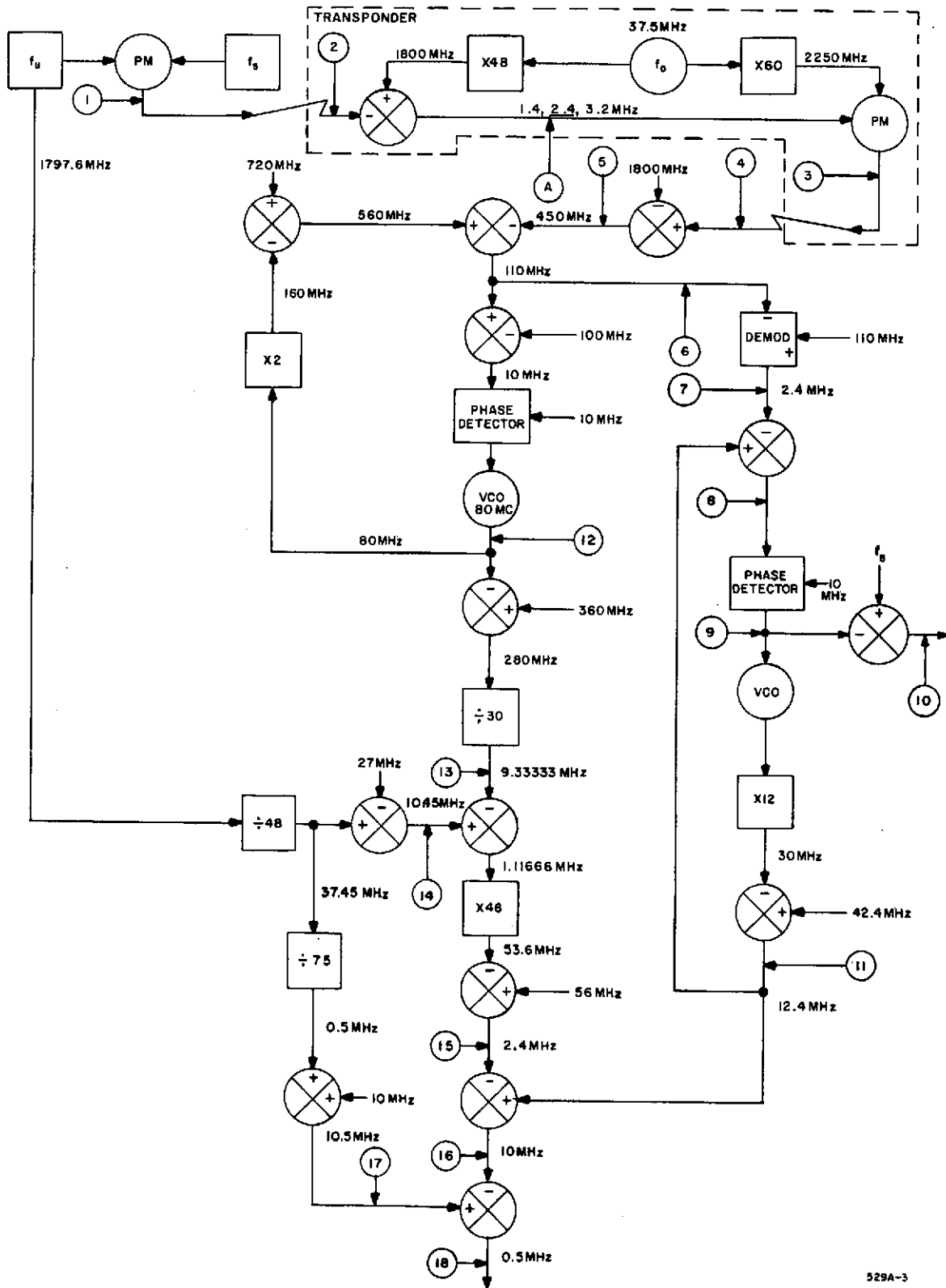
Figure 3. Modified S-Band System, Simplified Diagram
