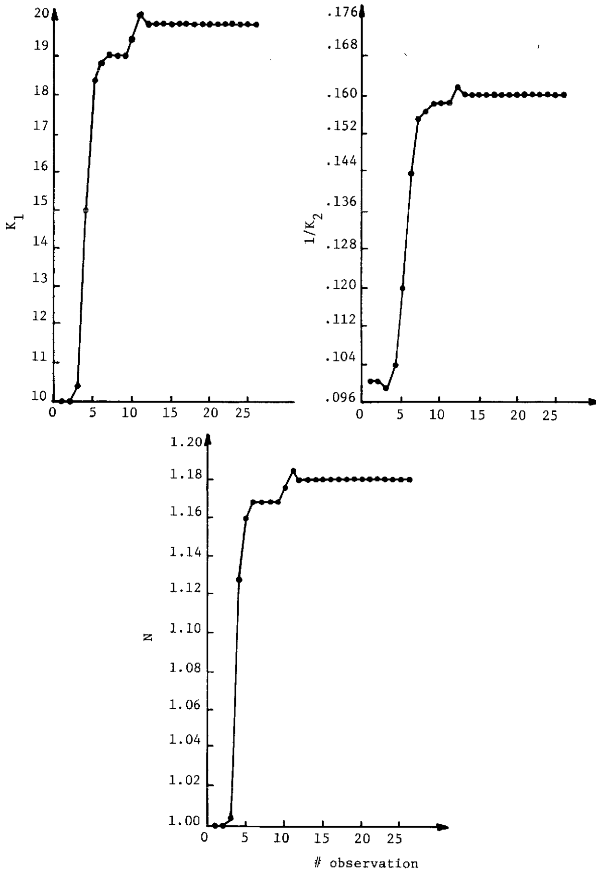
Figure 4-6: Estimation of time-invariant parameters by iterated extended Kalman filter.
