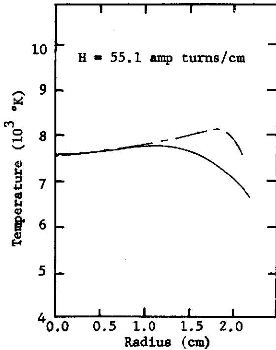
Figure 26. Comparison of Experimental and Theoretical Temperature Profiles for a Tungsten Seeded Argon Plasma at Four Representative Magnetic Field Intensities
