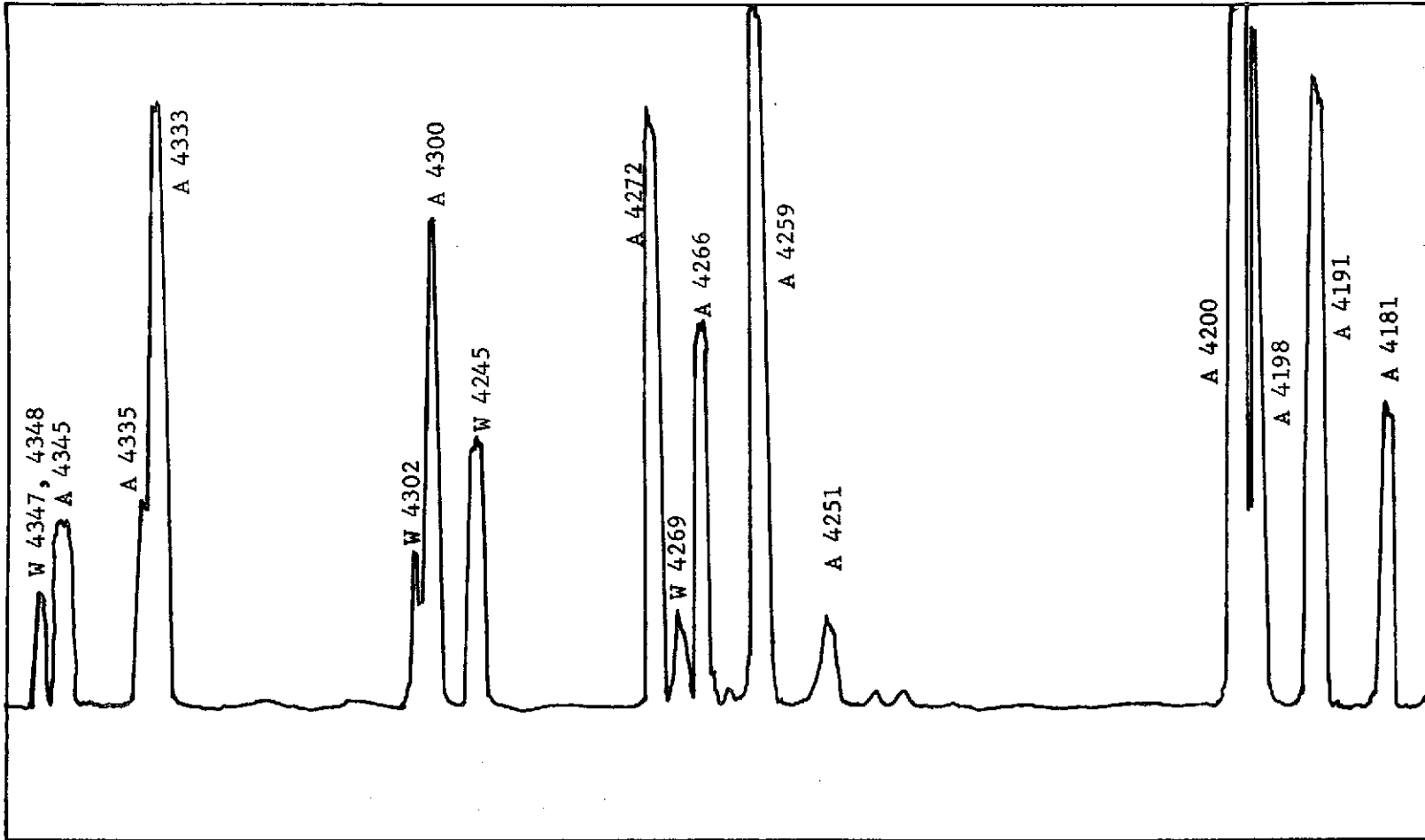
Figure 14. Photoelectric Trace of Tungsten Seeded Argon Spectrum from 4200 Å to 4400 Å
