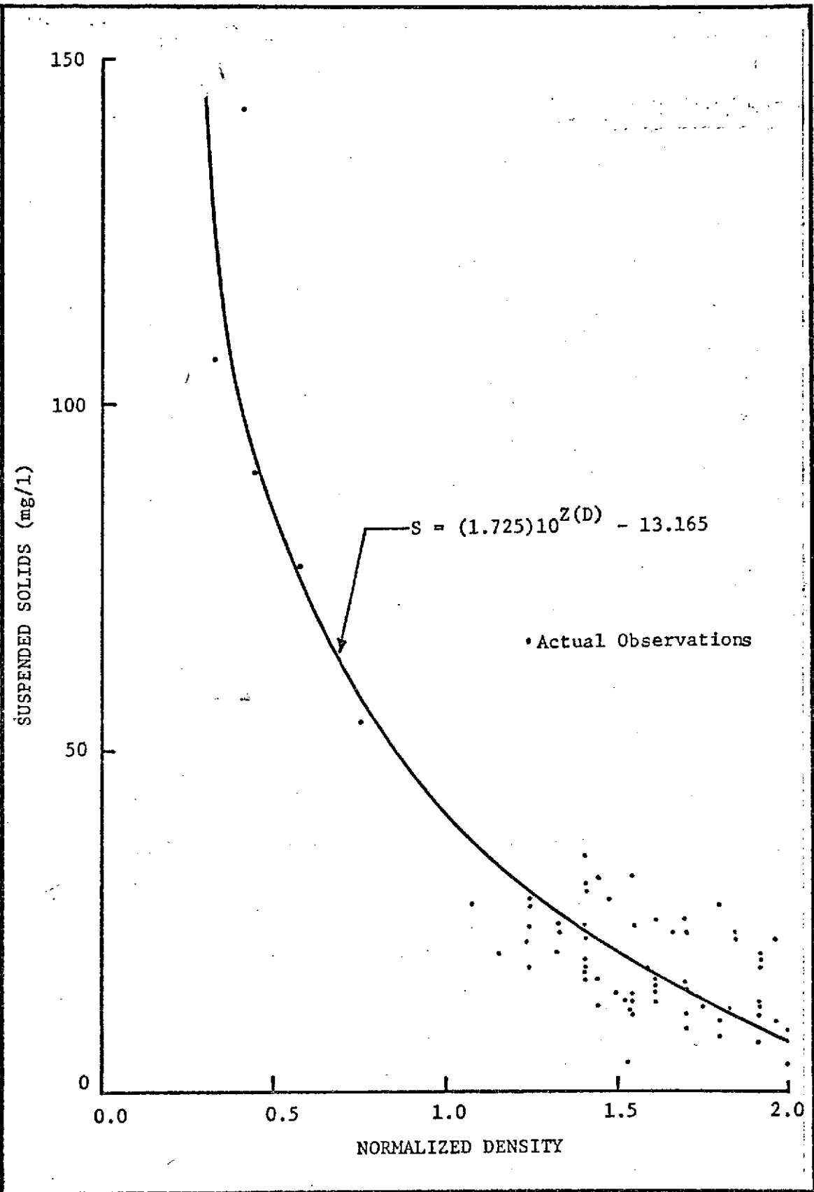
FIGURE 7. SUSPENDED SOLIDS/DENSITY MODEL FOR RED FILM LAYER.
