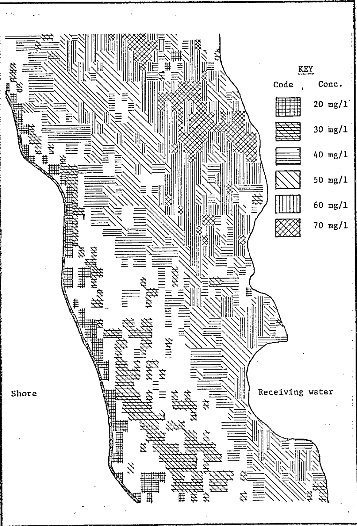
FIGURE 8. PORTION OF EQUAL CONCENTRATION DELINEATION OBTAINED IN THE RED FILM LAYER.
