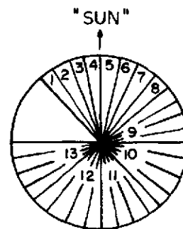
Figure 4 - 2 The data taking sequence. Each row corresponds to a different energy interval and is filled during one spacecraft rotation. The current is averaged over 11.25^\circ angular intervals as the spacecraft spins. For the 45^\circ sectors, 9-13, only the maximum of the four 11.25^\circ subsector average currents is recorded.
