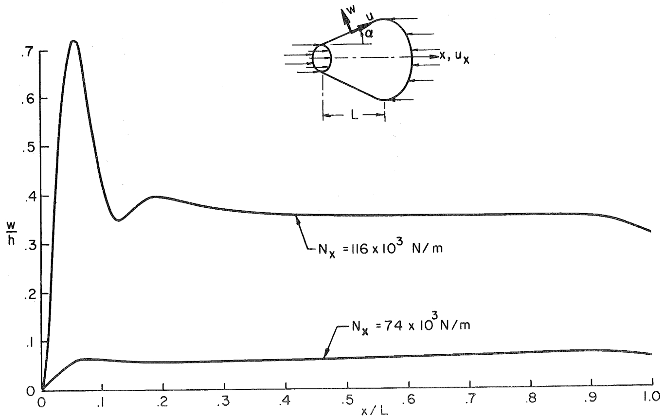
(b) Normal shell displacement along shell axis.
