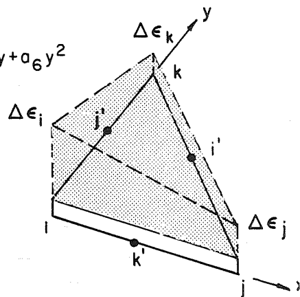
Fig.36 LINEAR STRAIN TRIANGLE (LST)
