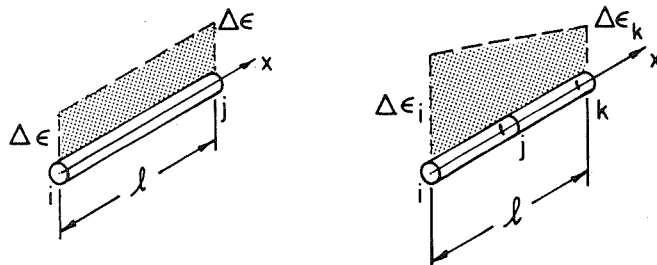
(a) Constant strain element (b) Linear strain element
