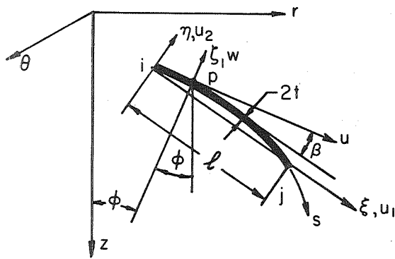
Fig. 41 AXISYMMETRIC REVOLVED TRIANGLE
