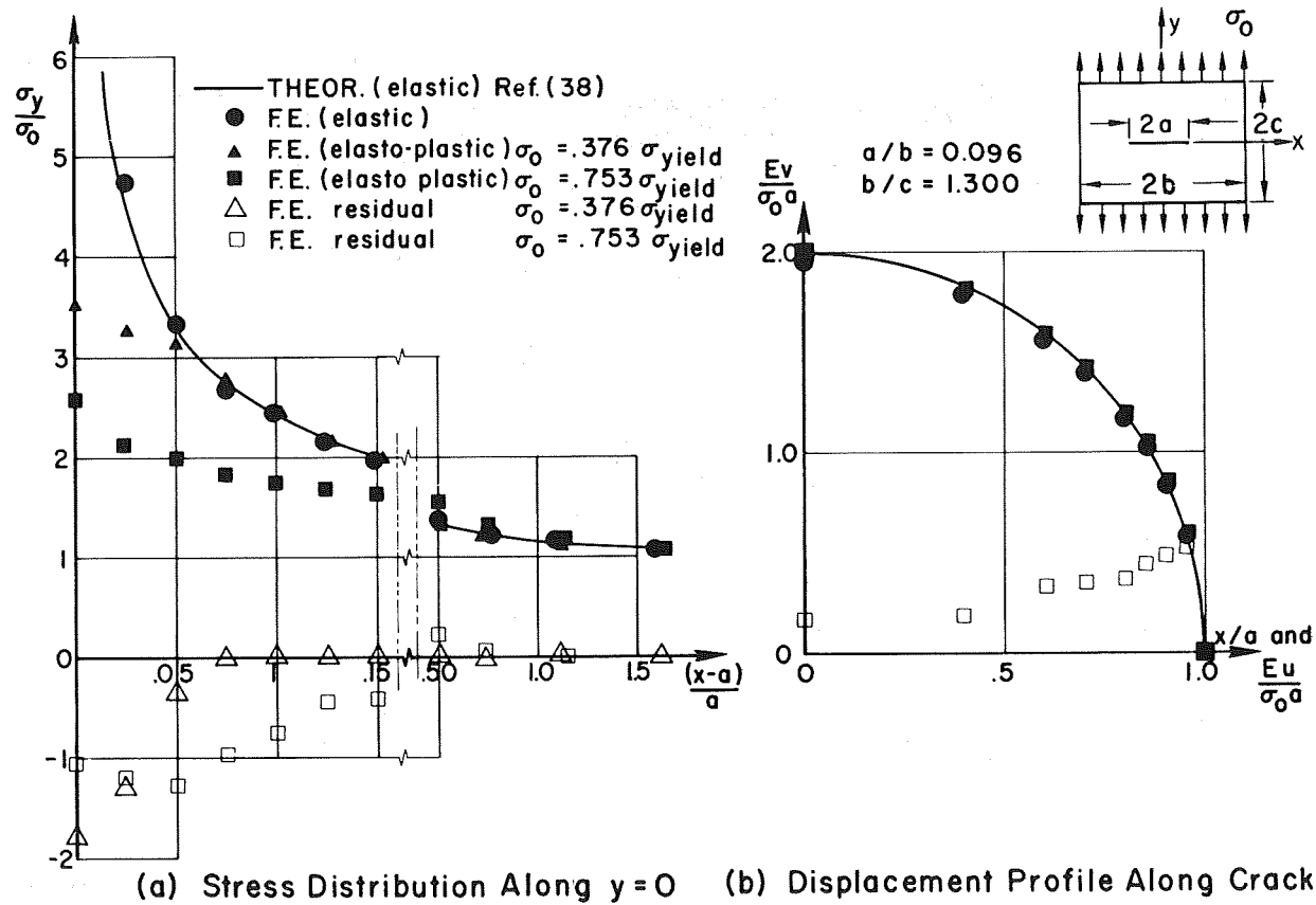
Fig 4. ELASTIC-PLASTIC ANALYSIS OF A UNIFORMLY LOADED SHEET WITH A CENTRAL CRACK
