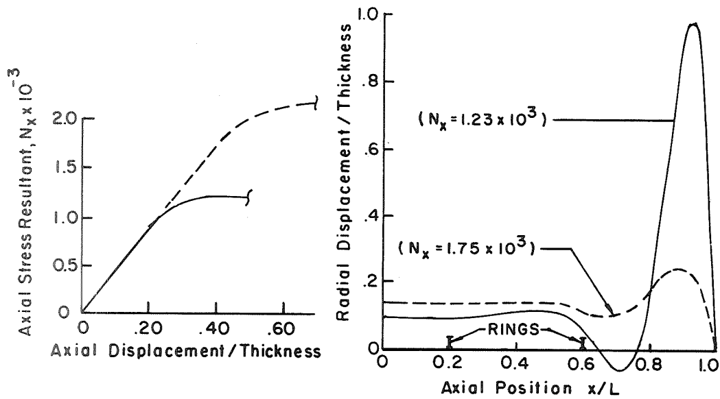
(a) Load vs axial end displacement. (b) Elastic and plastic radial displacement profile.
