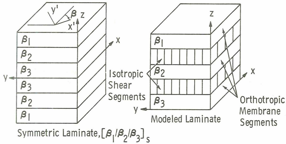
(a) Laminate Model
