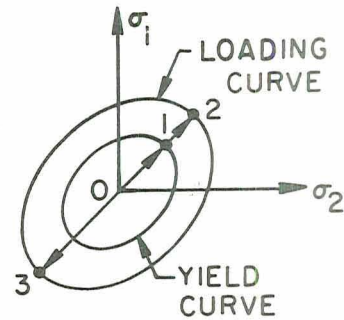
Fig. 48 ISOTROPIC HARDENING
