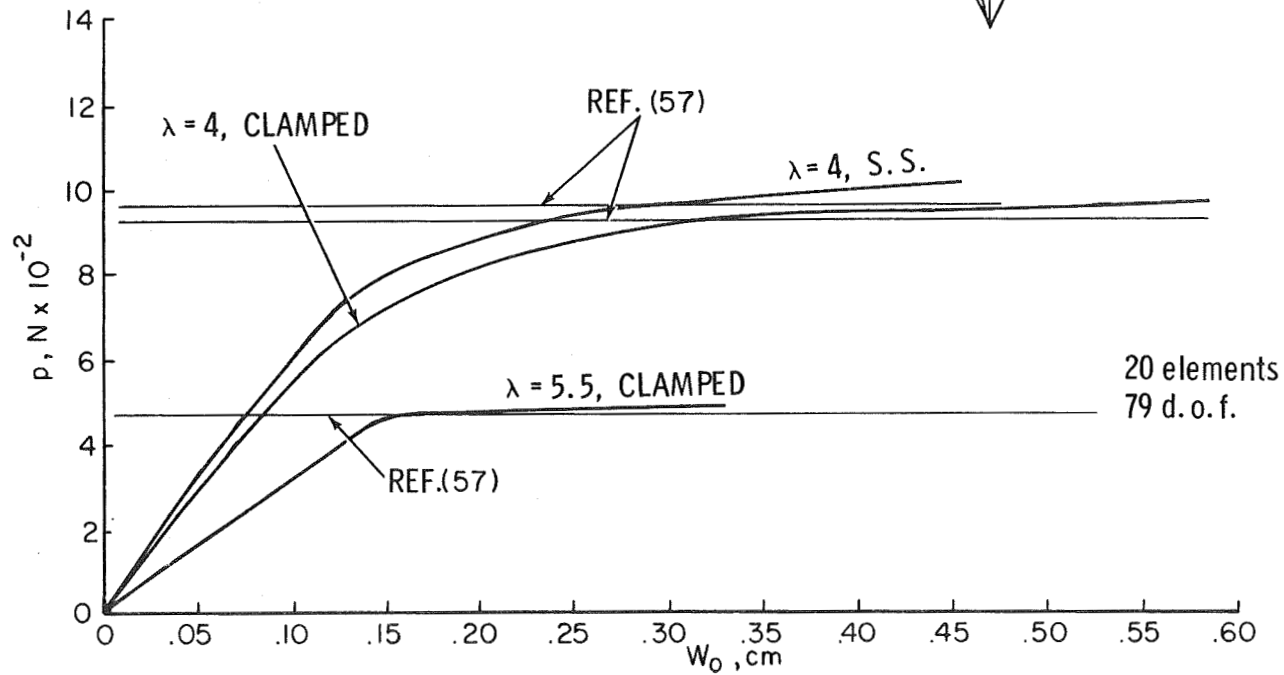
FIG. 28. ELASTO-PLASTIC BUCKLING OF SIMPLY-SUPPORTED AND CLAMPED SPHERICAL CAPS UNDER UNIFORM EXTERNAL PRESSURE (LOAD VS. CENTRAL DEFLECTION CURVES)
