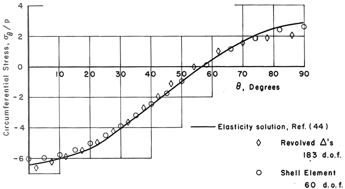
Fig. 8 CIRCUMFERENTIAL STRESS, \sigma_\theta , vs MERIDIONAL DIRECTION
