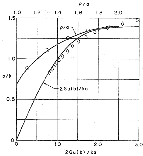
Fig. 9 PRESSURE p VERSUS RADIAL DISPLACEMENT u(b) AND RADIUS OF ELASTIC-PLASTIC BOUNDARY, \rho .
