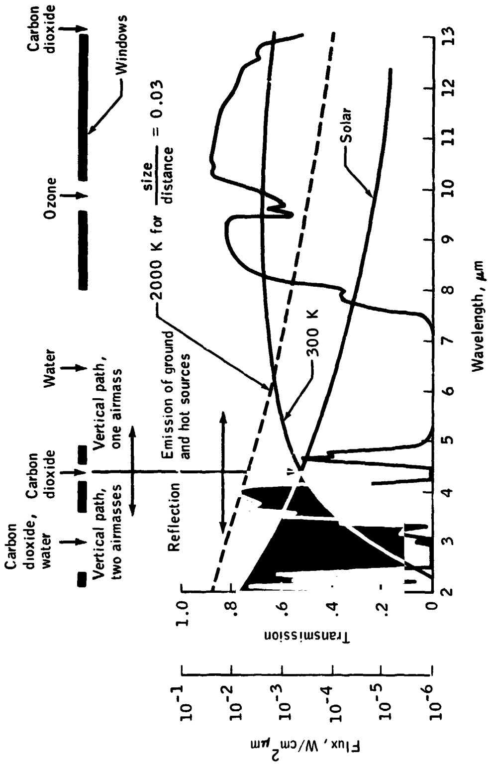
Figure 2.- Atmospheric transmission.
