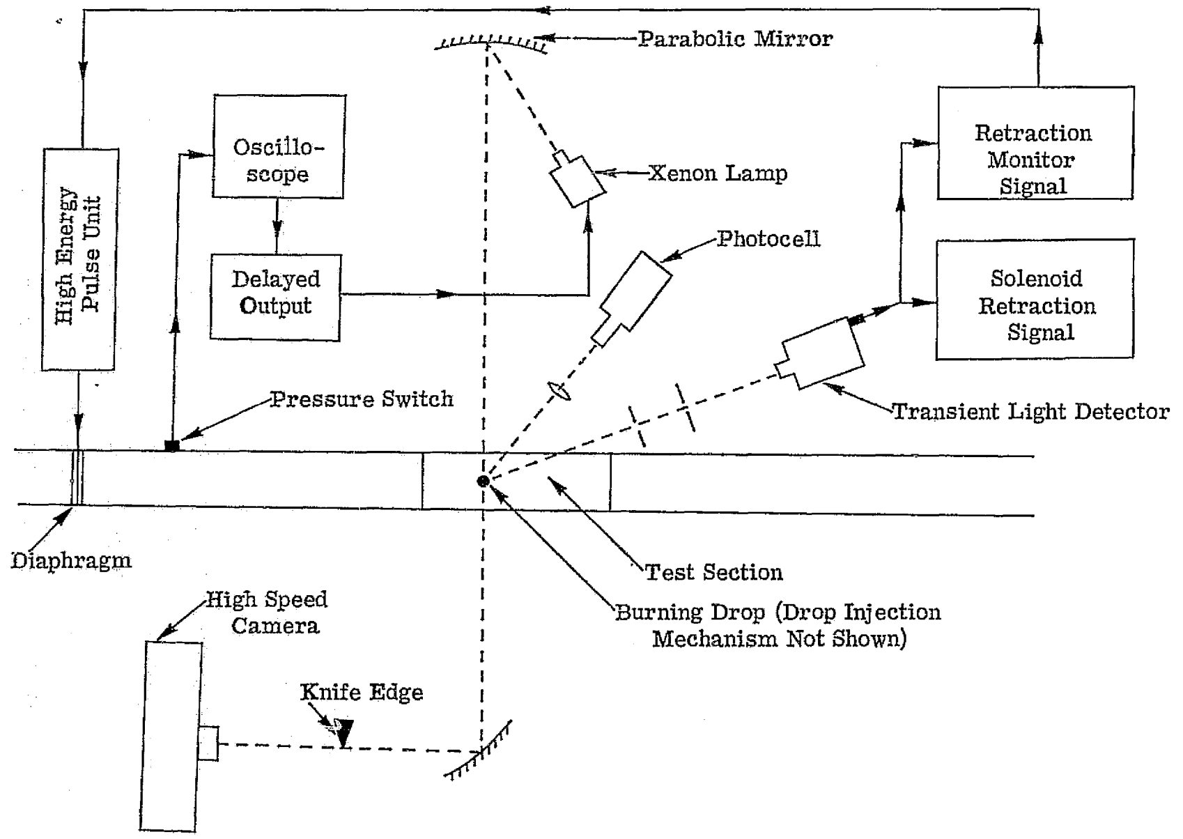
Figure 3. Equipment Arrangement.
