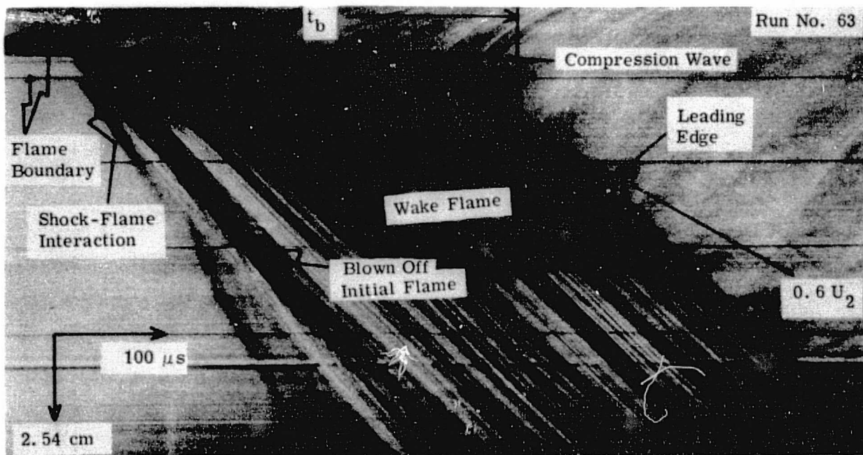
Figure 6. Streak Schlieren Photograph of Drop with Wake Flame, P_1 = 30 \text{ in. Hg O}_2 , M_s = 1.72 .
