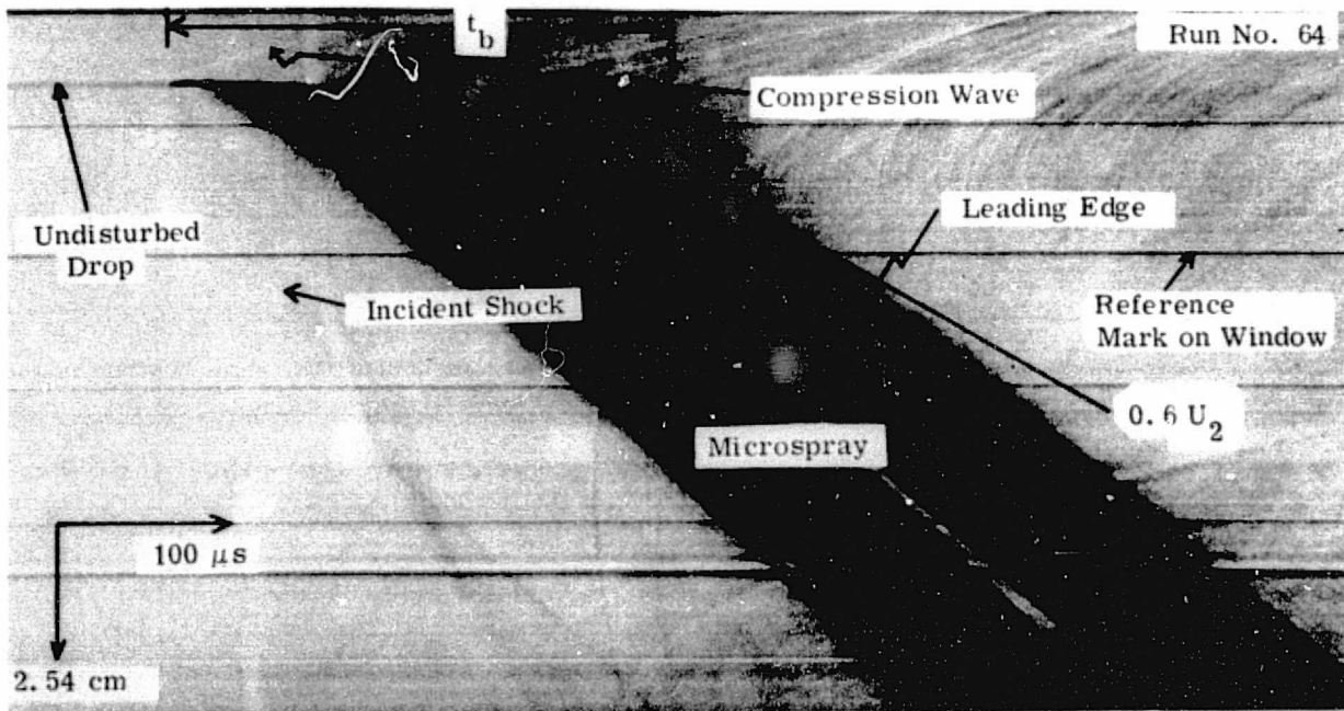
Figure 5. Streak Schlieren Photograph of Non-ignited Drop, P_1 = 30 \text{ in. Hg O}_2 , M_s = 1.73 .
