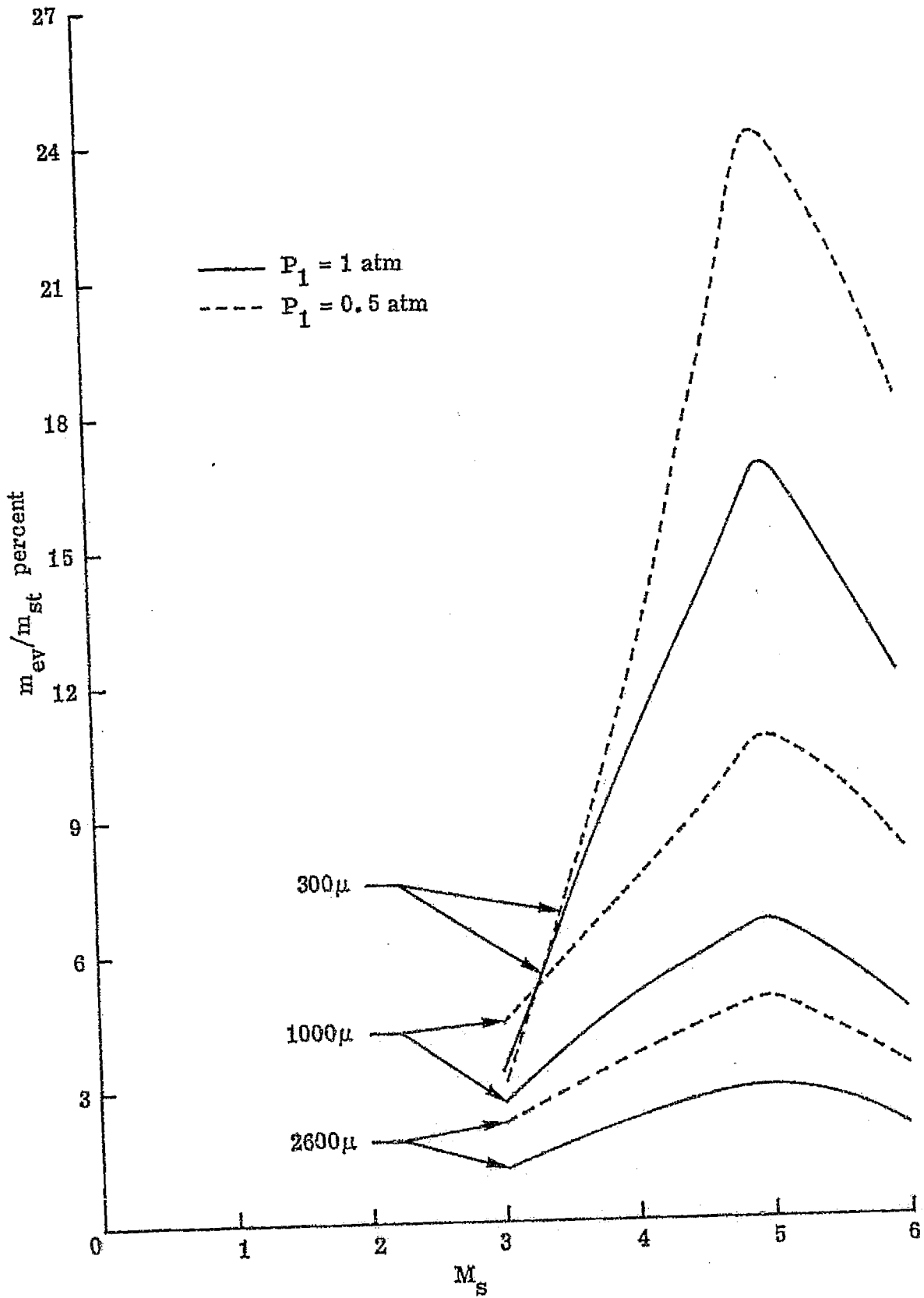
Figure 17. m_{ev}/m_{st} vs M_s .
