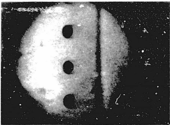
Figure 13. Shock Wave over a Water Drop, d = 750 \mu\text{m} , M_s = 2.7 , t = 2.6 \mu\text{s} .
