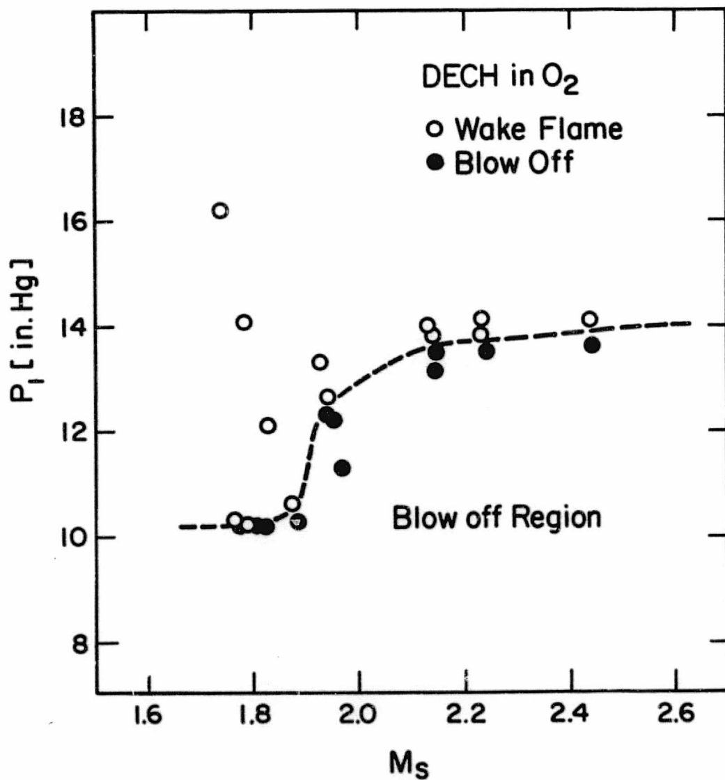
Figure 9. Limiting Initial Pressure of Pure Oxygen for Blow Off.
