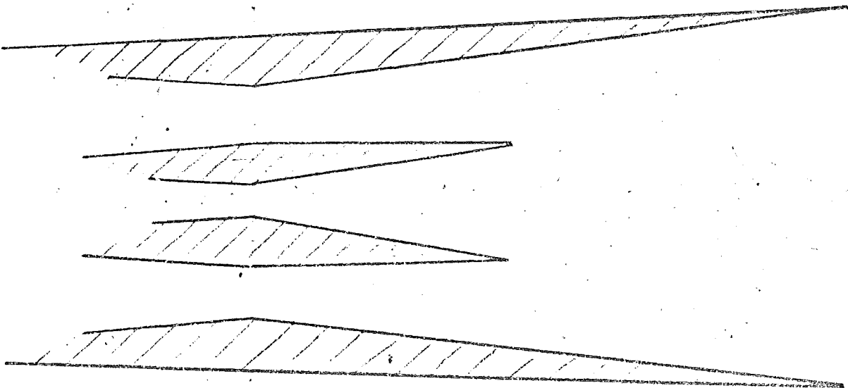
FIGURE 4. INTERNAL NOZZLE SHAPES WITH ADDITIONAL LATERAL EXPANSION
