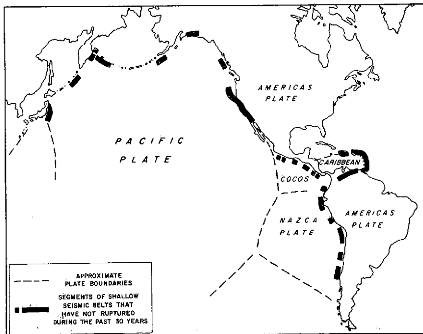
Figure 7a. (Top) Major shallow seismic belts examined by Kelleher, Sykes and Oliver. (3)
