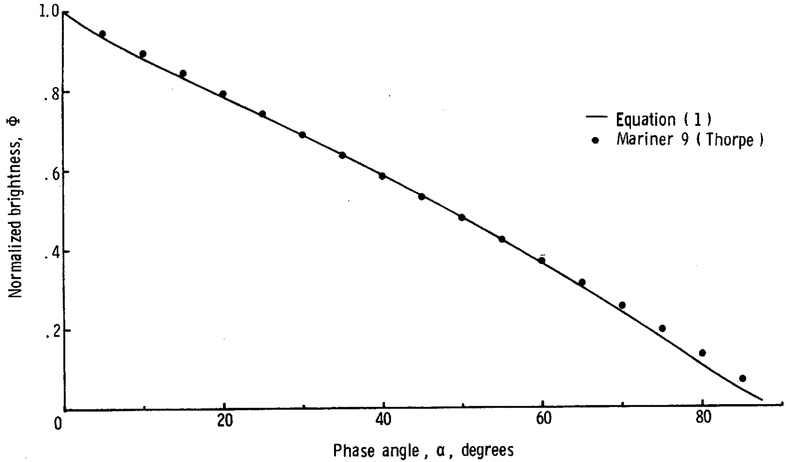
Figure 3. - Comparison of the normalized brightness of Mars (Mariner 9, Thorpe) and the value given by equation (1).
