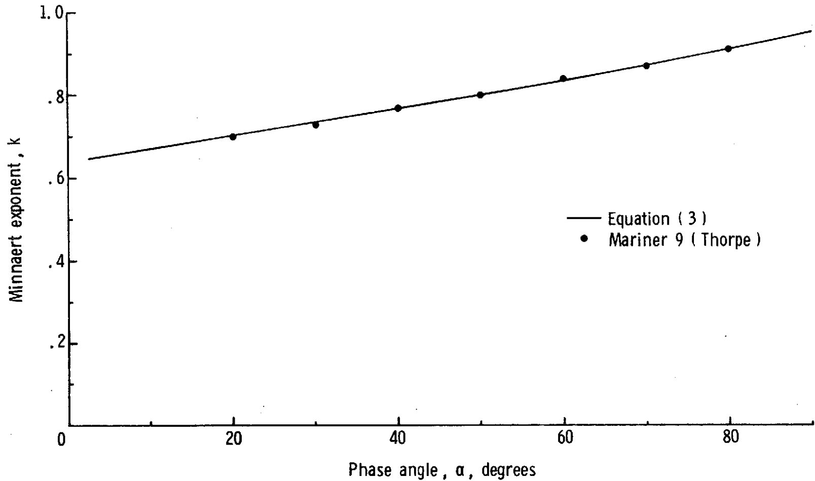
Figure 4. - Comparison of the Minnaert exponent for Mars (Mariner 9, Thorpe) and the value given by equation (3).
