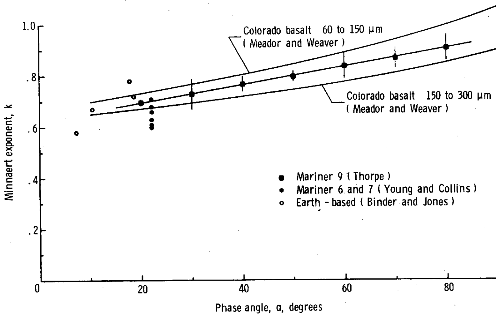
Figure 2. - Comparison of the Minnaert exponent for Mars (derived from Earth-based and Mariner 6, 7, and 9 data) and a basalt.
