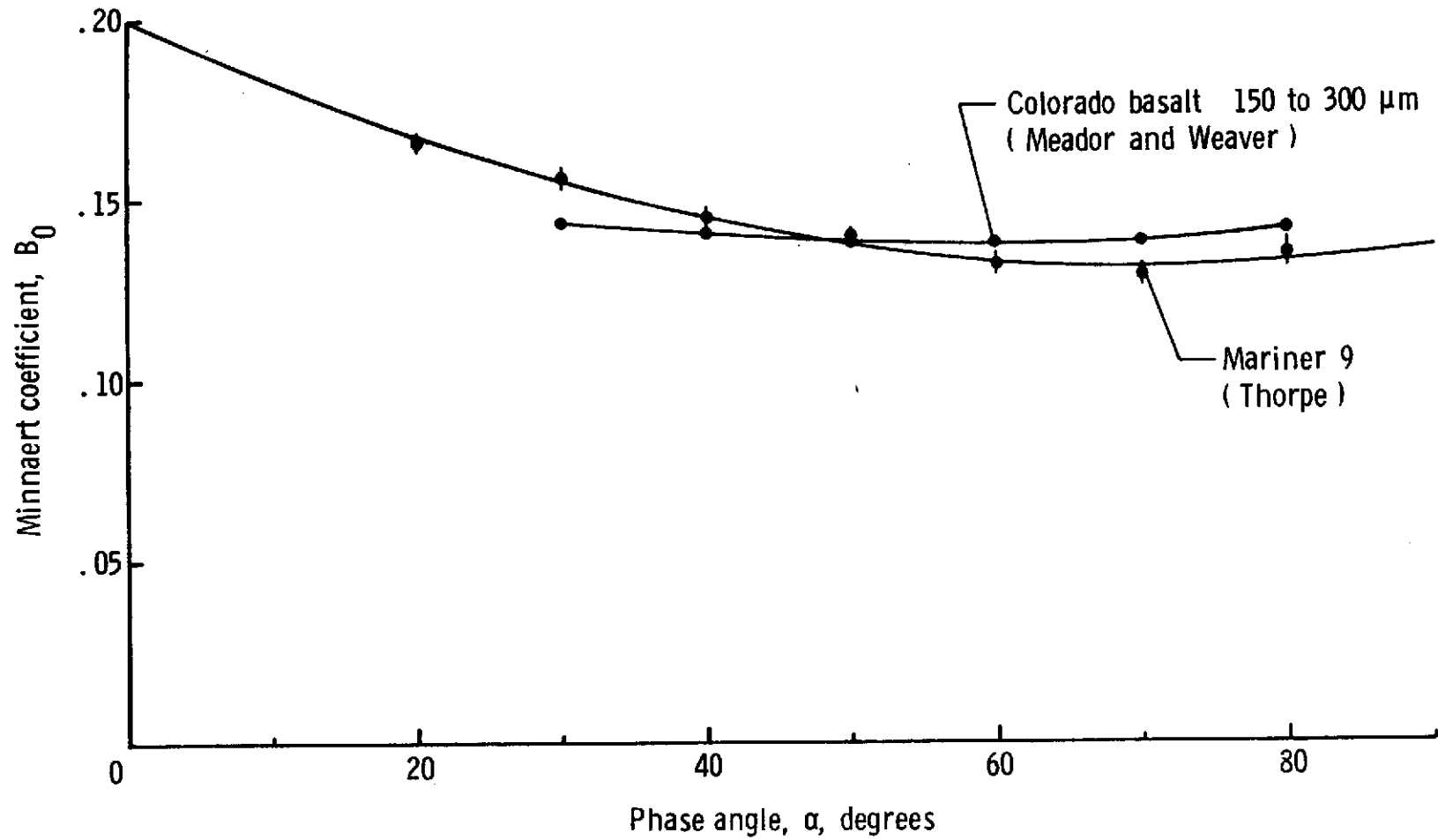
Figure 1. - Comparison of the Minnaert coefficient for Mars (Mariner 9, Thorpe) and a basalt.
