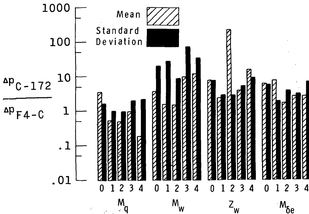
(b) Short Period (C-172).
