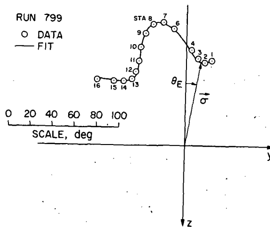
(b) Large amplitude motion about a near 90^\circ trim point.
