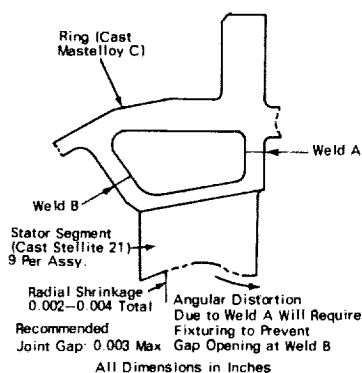
Figure 1. Illustration of Cross-Section of Electron Beam Weld Joint.
