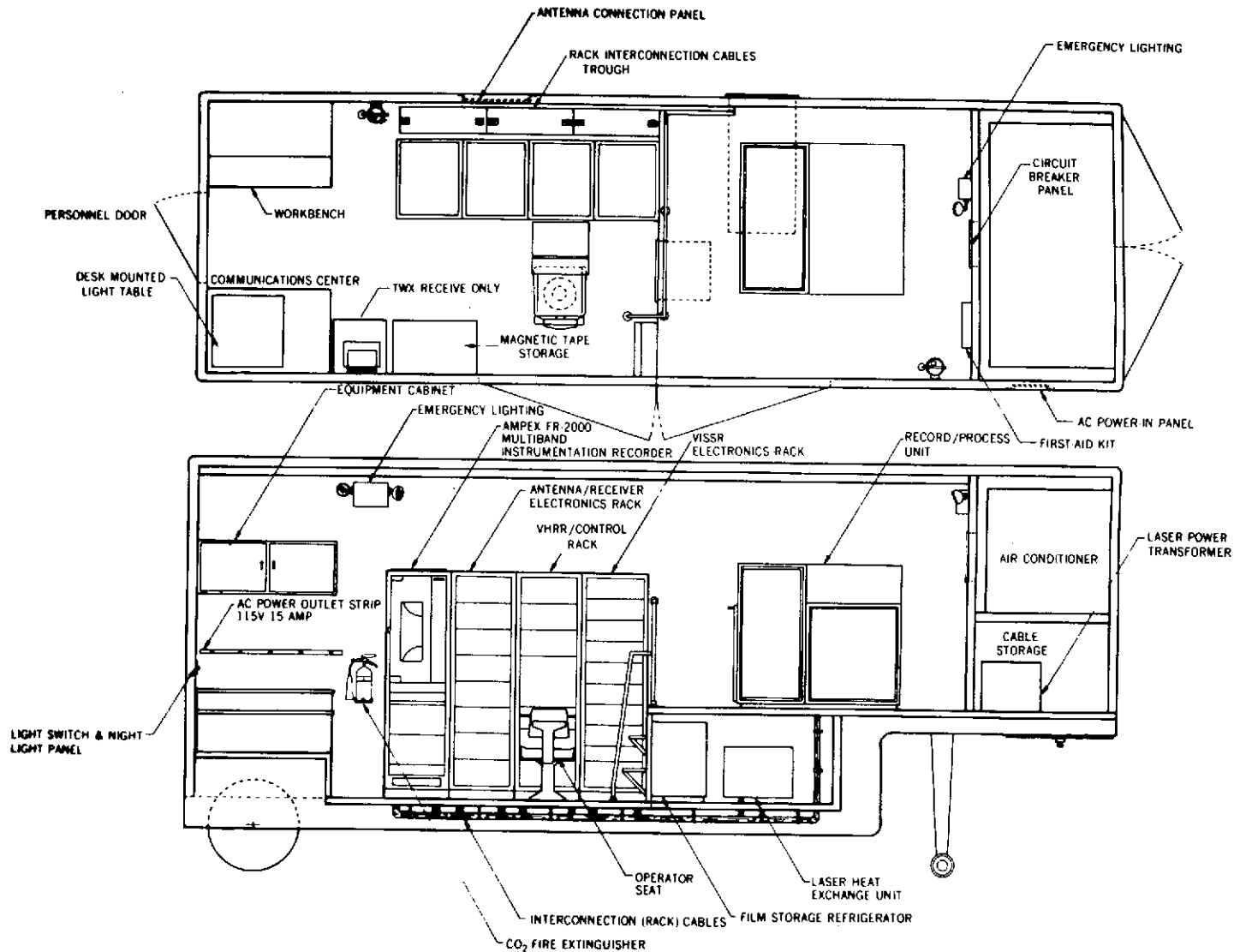
Figure 6-37. Direct Readout Ground System Instrumentation Van
