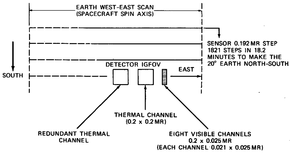
Figure 6-28. Synchronizer/Data Buffer System Configuration
