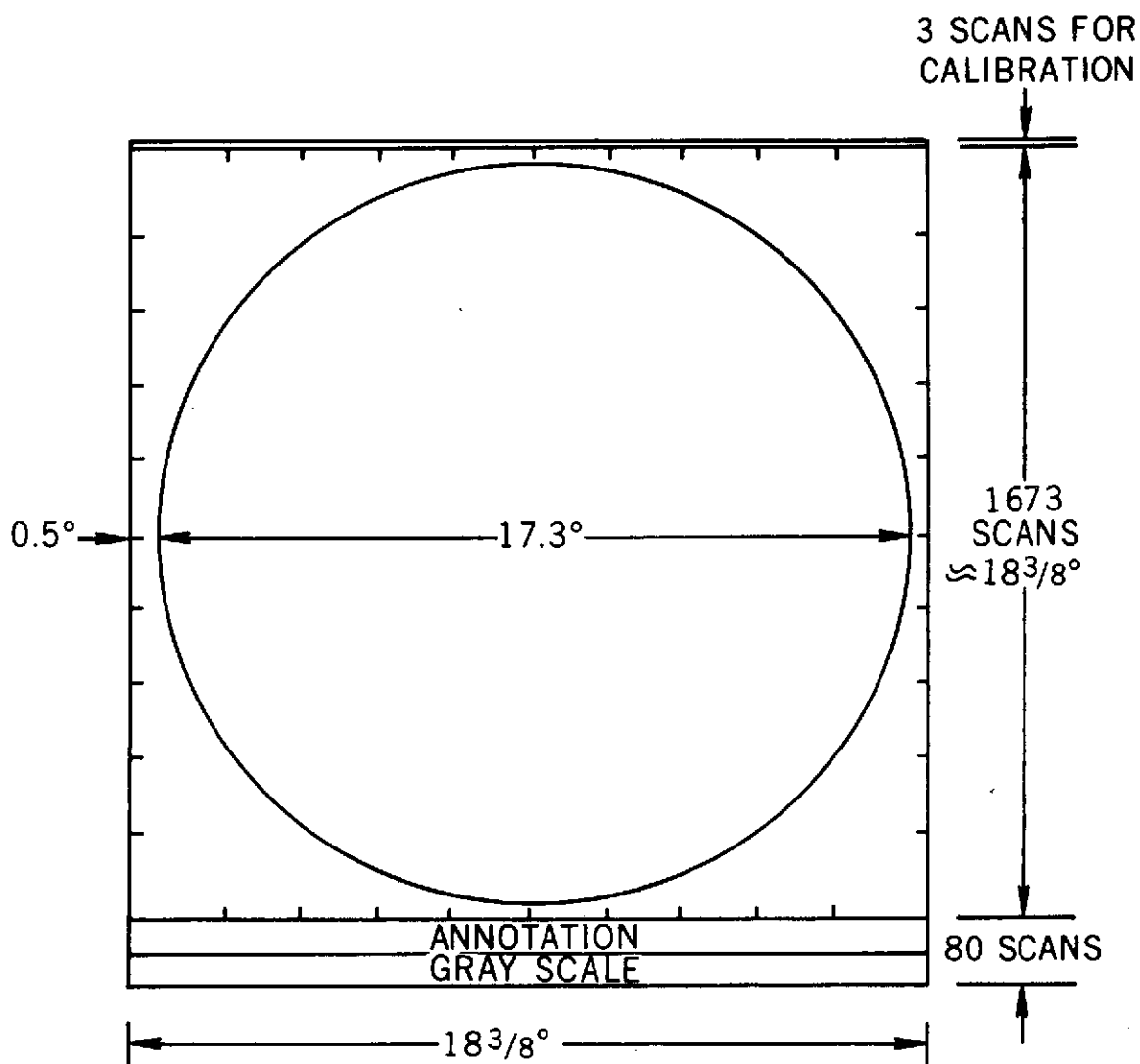
Figure 6-36. VISSR Image
