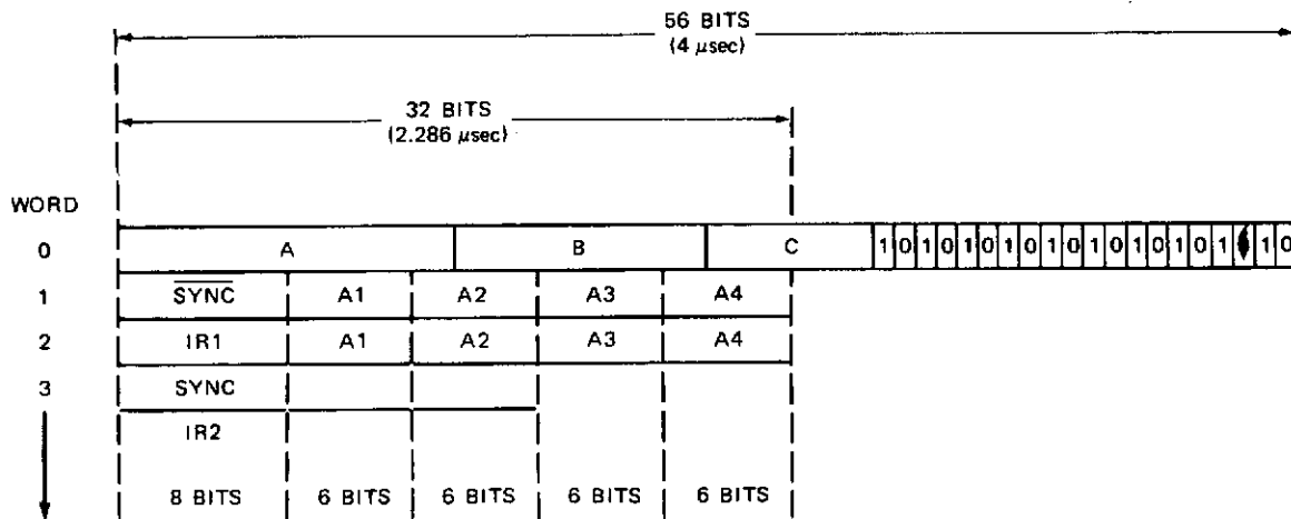
Figure 6-34. VISSR PCM Data Format, Mode 2
