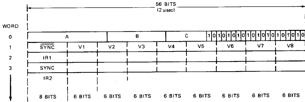
Figure 6-33. VISSR PCM Data Format, Mode 1
