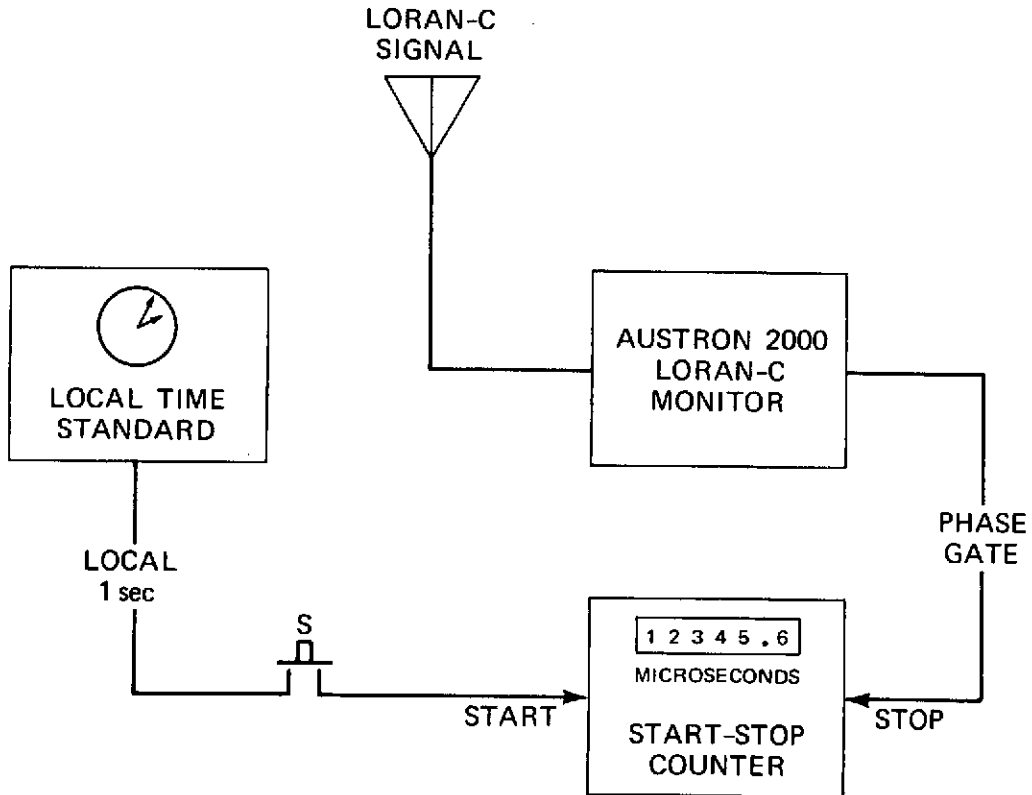
Figure 6-20. Basic System for Loran-C Timing
