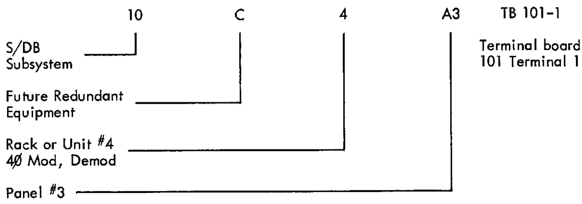
Figure 6-7. Typical Examples of Rack Numbering System
