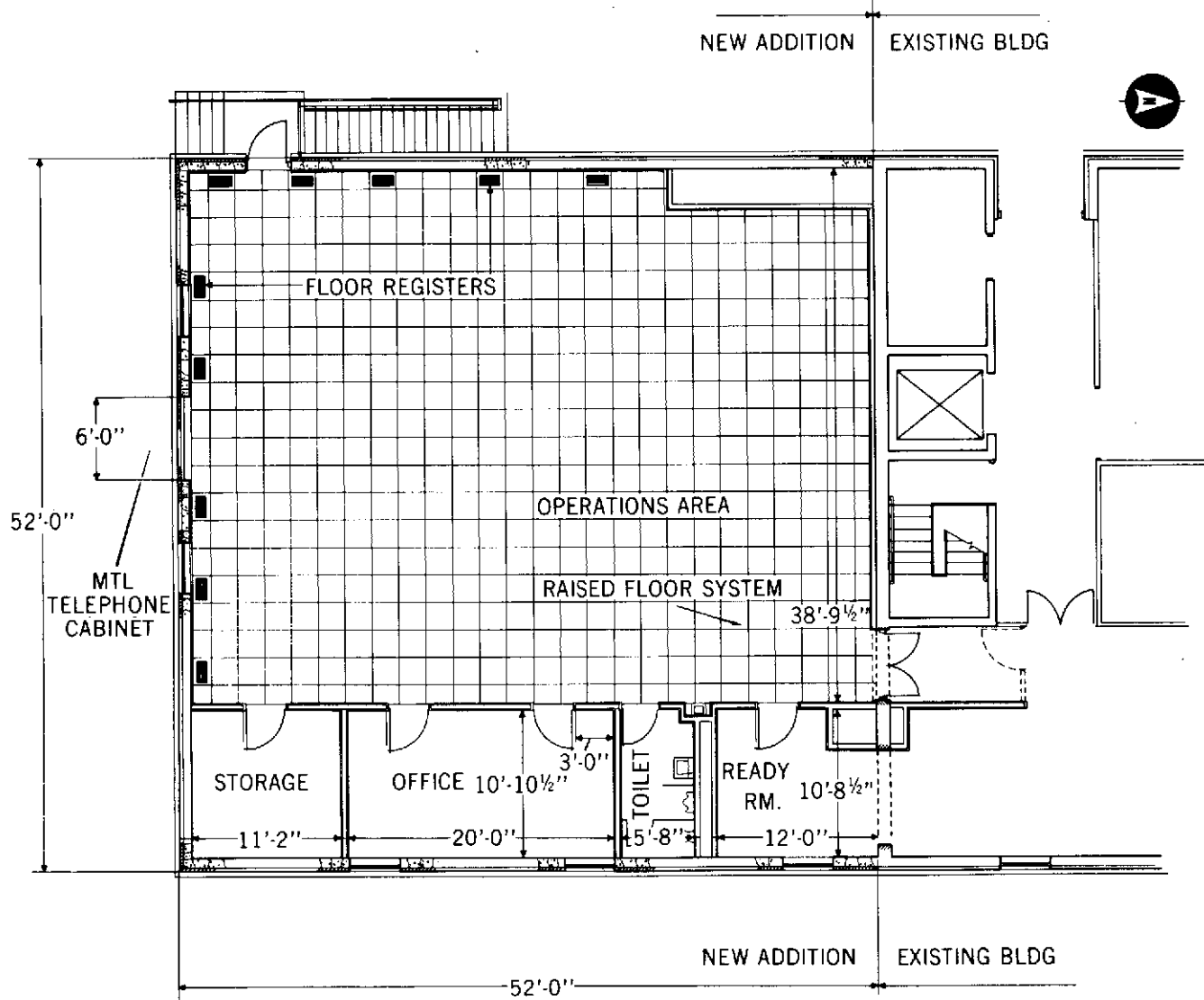
Figure 6-3. First Floor Layout Plan
