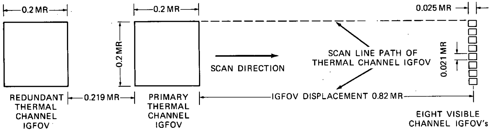
Figure 6-29. VISSR Thermal Channel and Visible Channels IGFOV Arrangement
