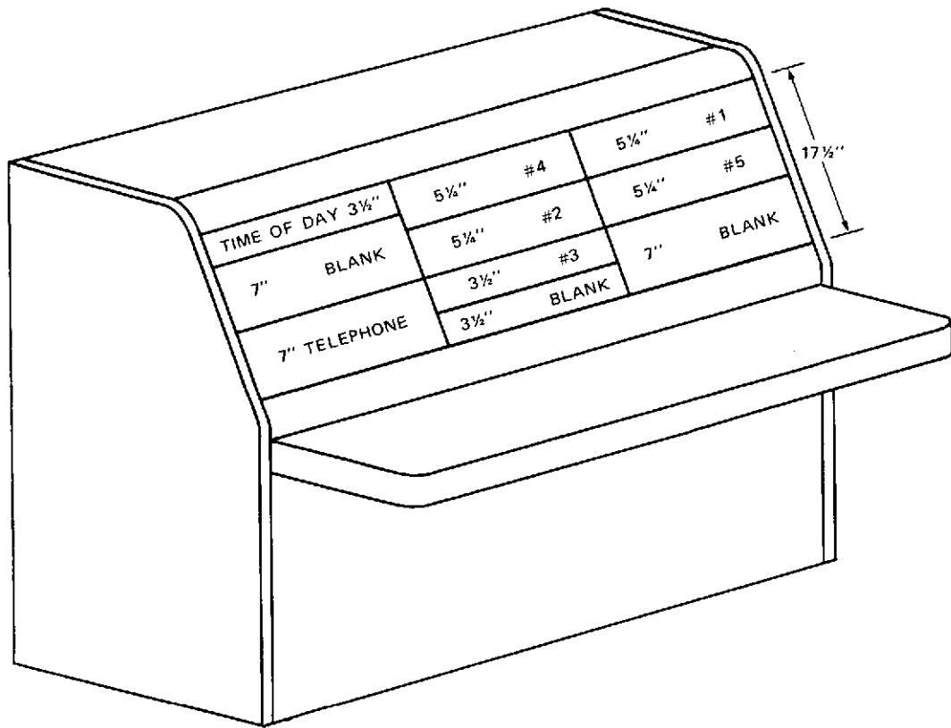
Figure 6-8. Master Control Console
