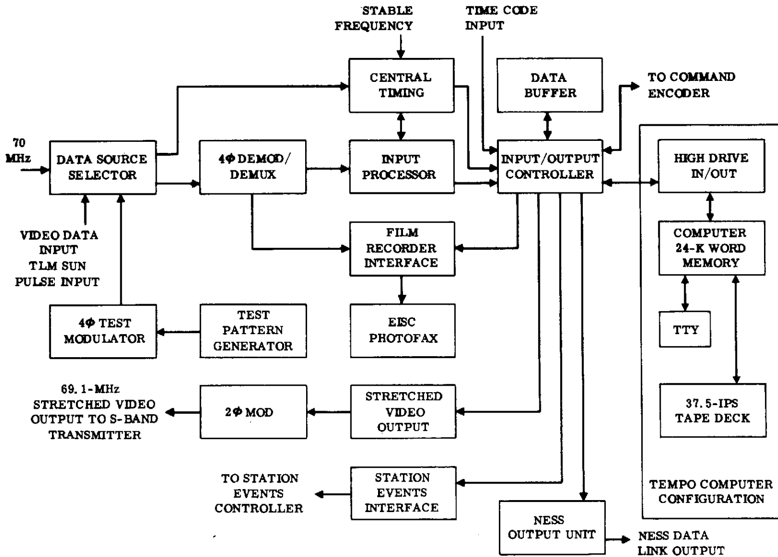
Figure 6-32. Synchronizer/Data Buffer System, Block Diagram
