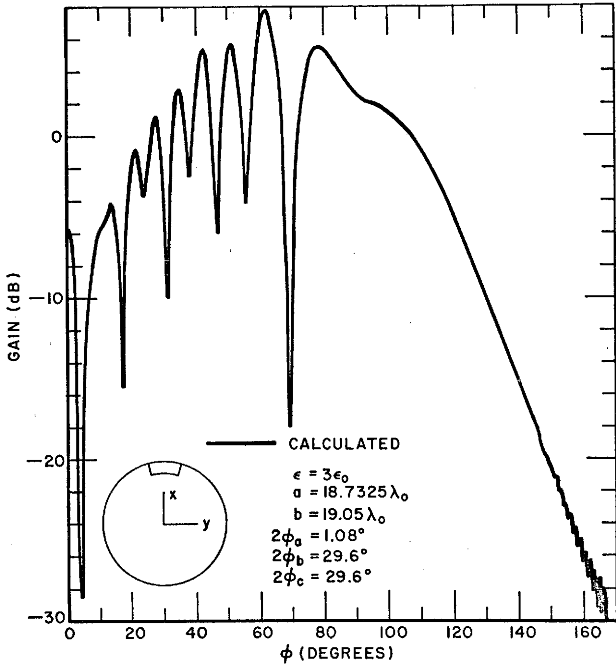
Fig. 5. Far-field pattern of TE axial slot radiating through a flush-mounted dielectric window in a circular cylinder. The dielectric constant is 3.
