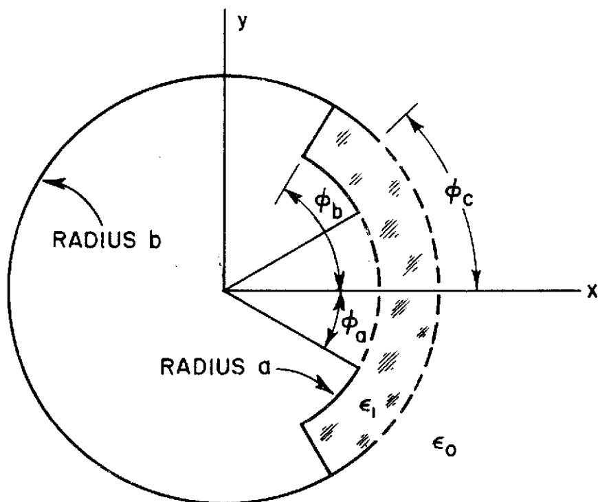
Fig. 3. An axial-slot antenna radiates through a flush-mounted dielectric window in a conducting circular cylinder. The principal field components are E_\phi and H_z .
