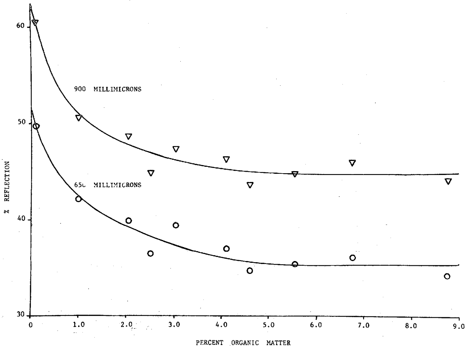
Fig. 14. Relationship of reflection for Sassafra fsl at 650 and 900 millimicrons to various levels of soil organic matter.
