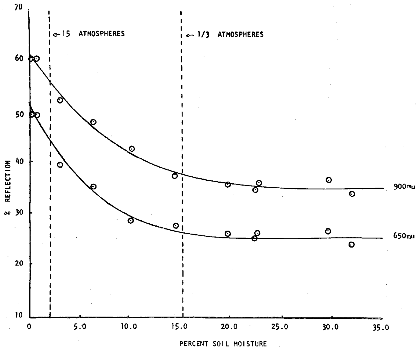
Fig. 13. Relationship of percent reflection to percent soil moisture for Sassafras fs1 with 0.2% organic matter at 650 and 900 millimicrons.
