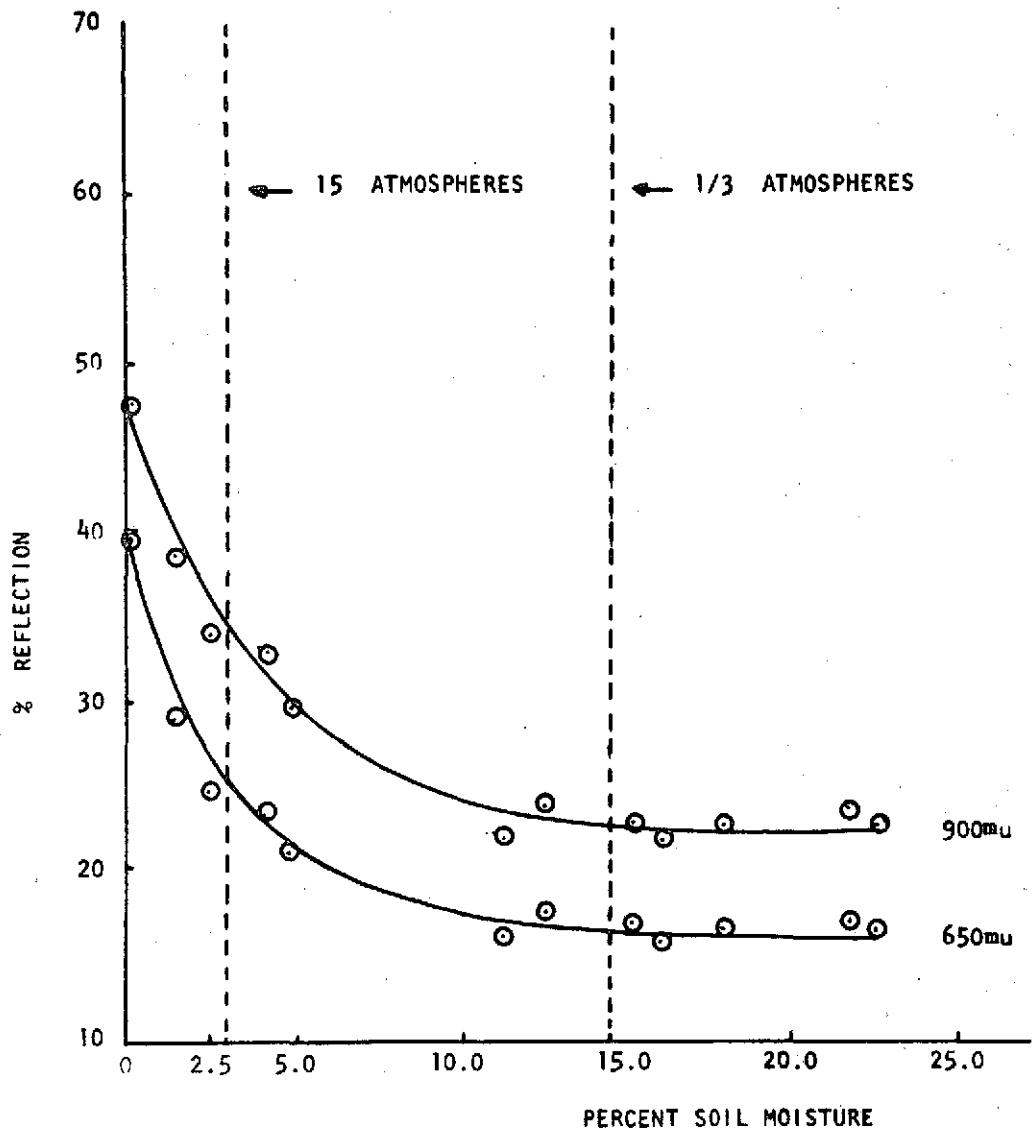
Fig. 12. Relationship of percent reflection to percent soil moisture for Sassafra fsl with 3.0% O.M. at 650 and 900 millimicrons.
