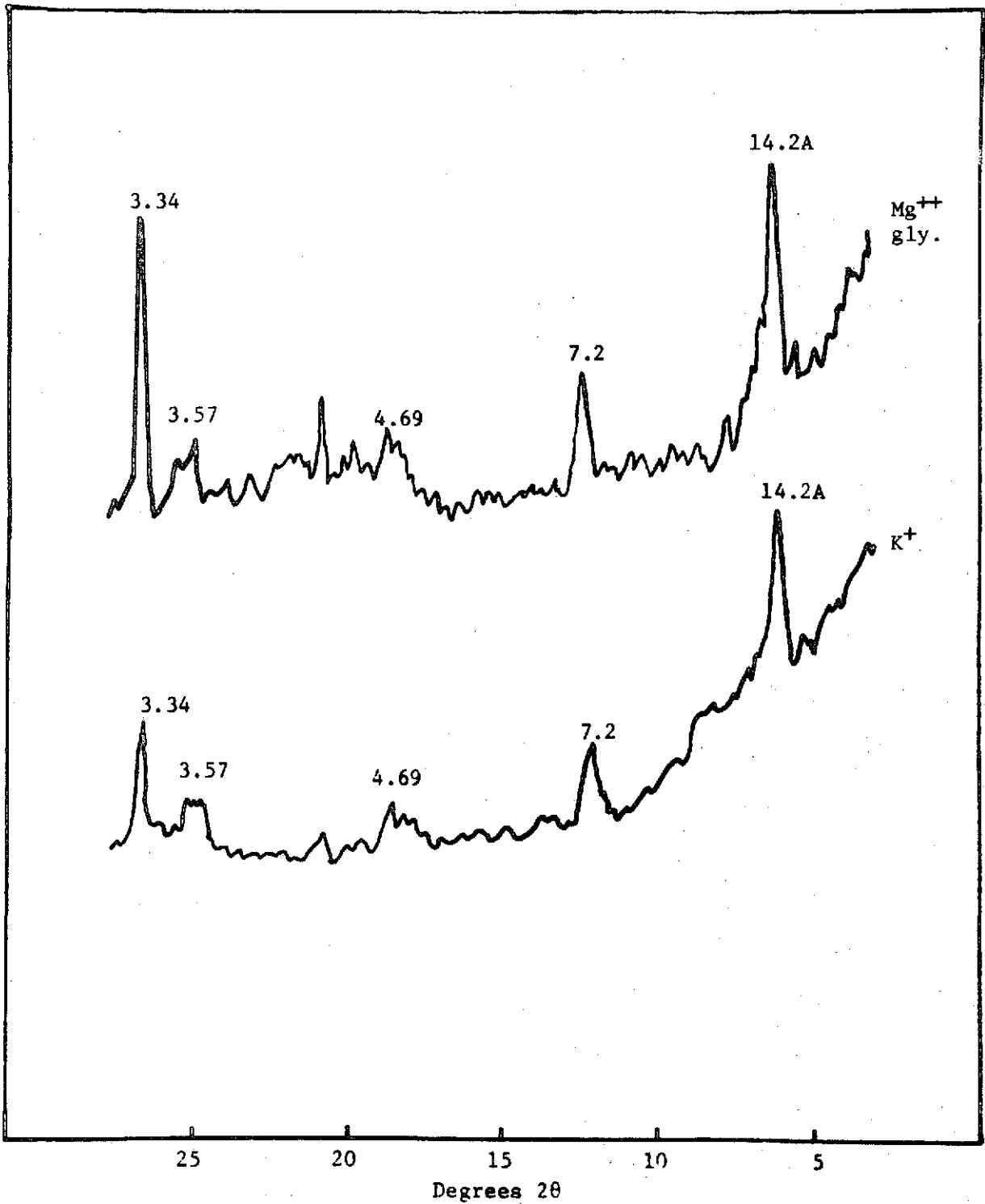
Fig. 3. X-ray diffraction patterns of the clay fraction (<math><2\mu</math>) of a typical SassafRAS Ap horizon, Mg 2+ saturated-glycerol solvated, and K + saturated.
