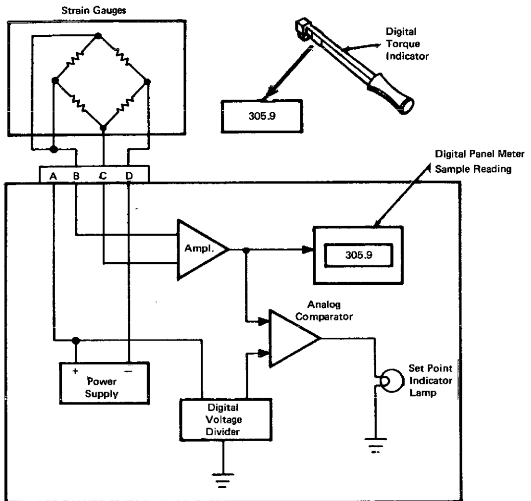
Digital Torque Indicator With Digital Set Point
