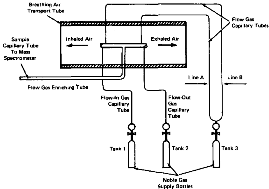
Breathing Air and Tracing Gas, Flow-Volume and Flow-Direction Mixing Chamber
