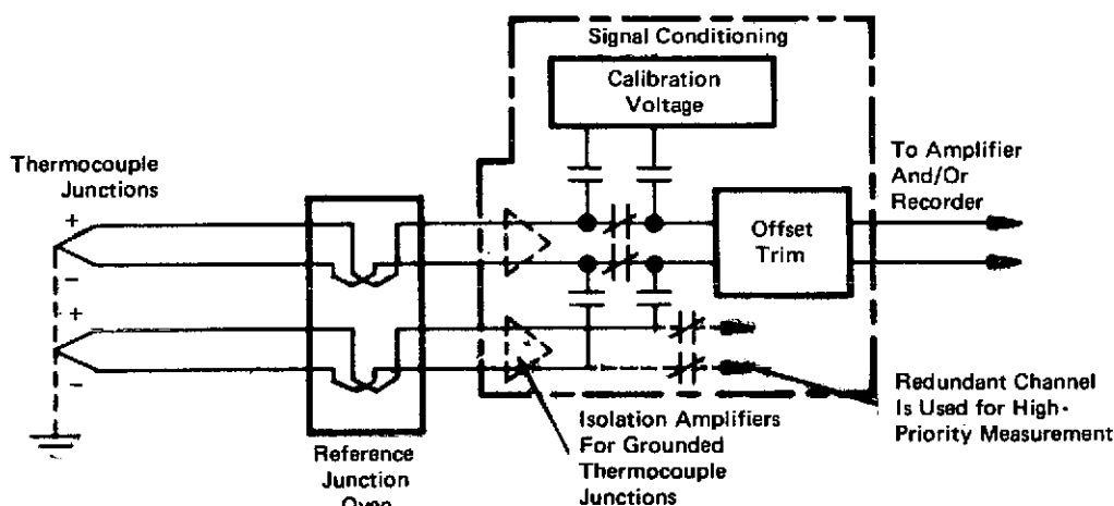
Figure 1. Modified Circuit
