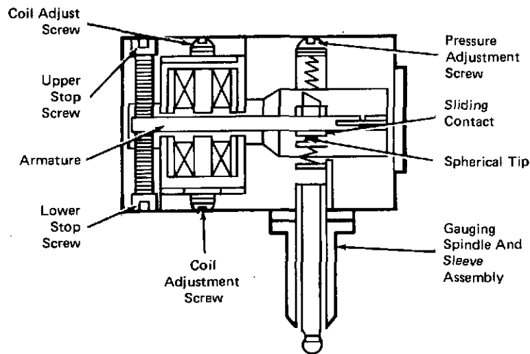
Figure 1. Conventional Device
