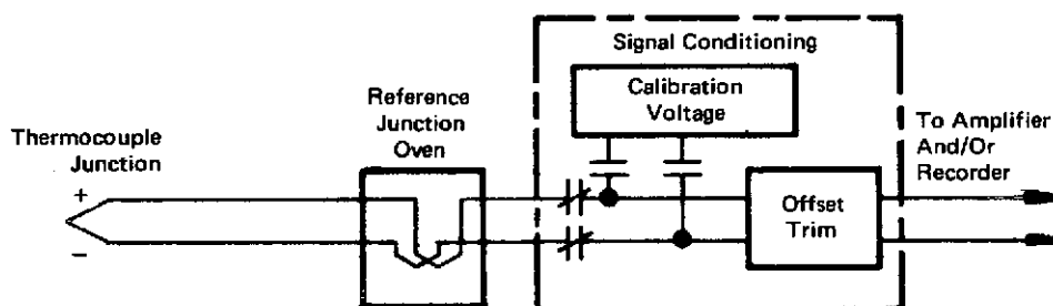
Figure 2. Conventional Circuit
