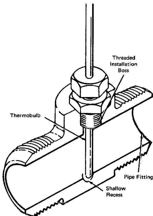
Thermobulb Installed in a Pipe Fitting
