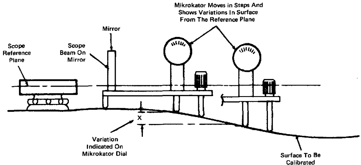
Calibration of Inspection Grade Surface Plates
