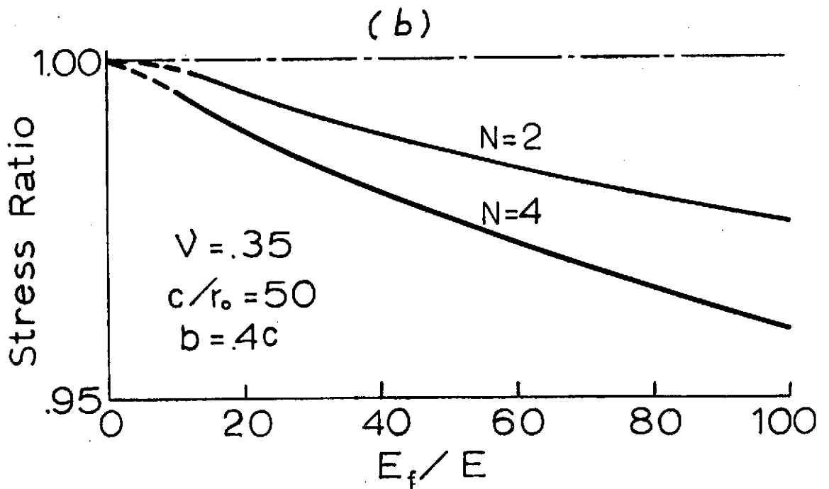
Figure 14. The ratio of the maximum filament stress for N > 1 to that for N=1 as a function of the distance parameter b and the modulus ratio E_f/E .
