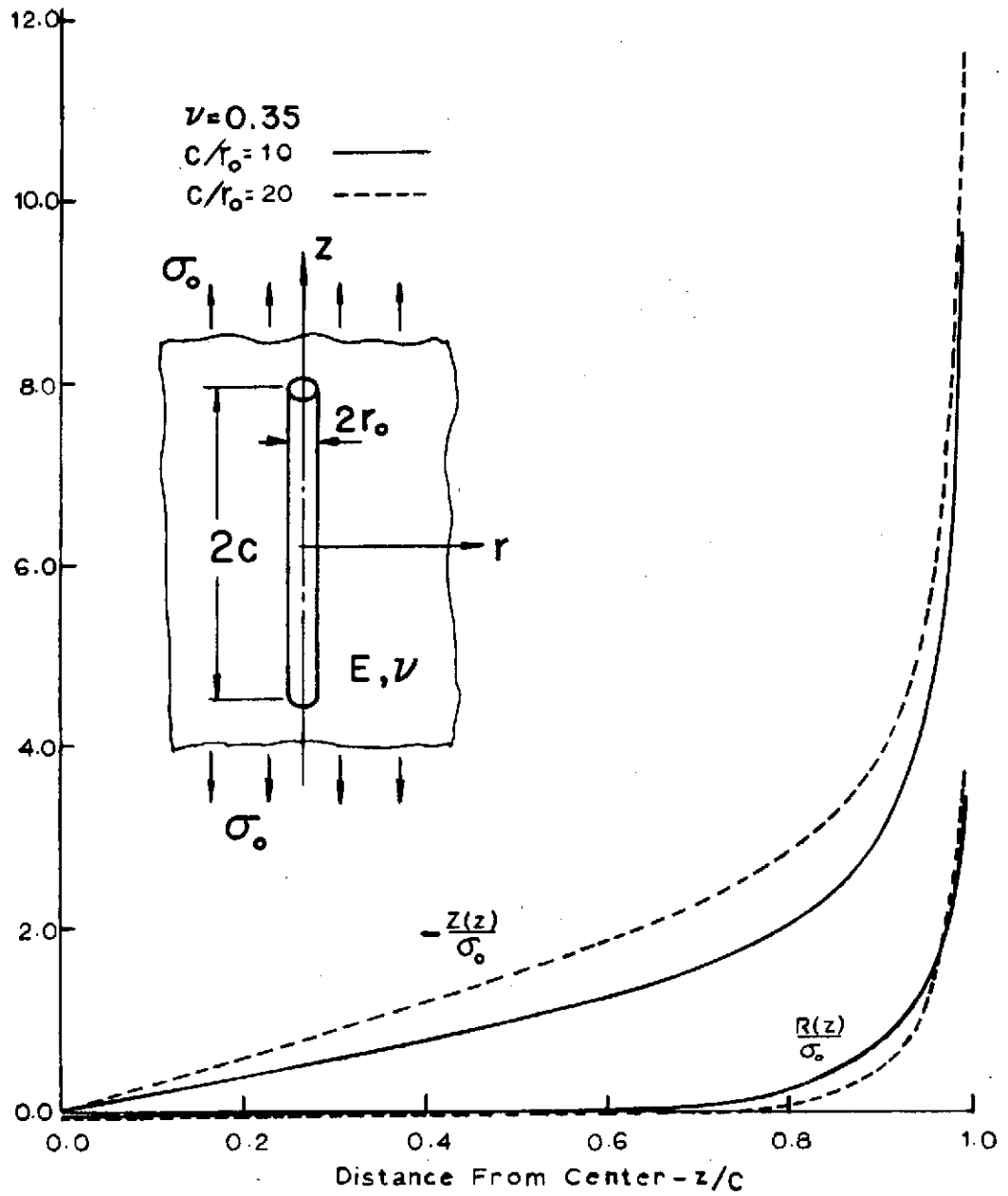
Figure 2. Radial and axial contact stresses for a rigid filament.
