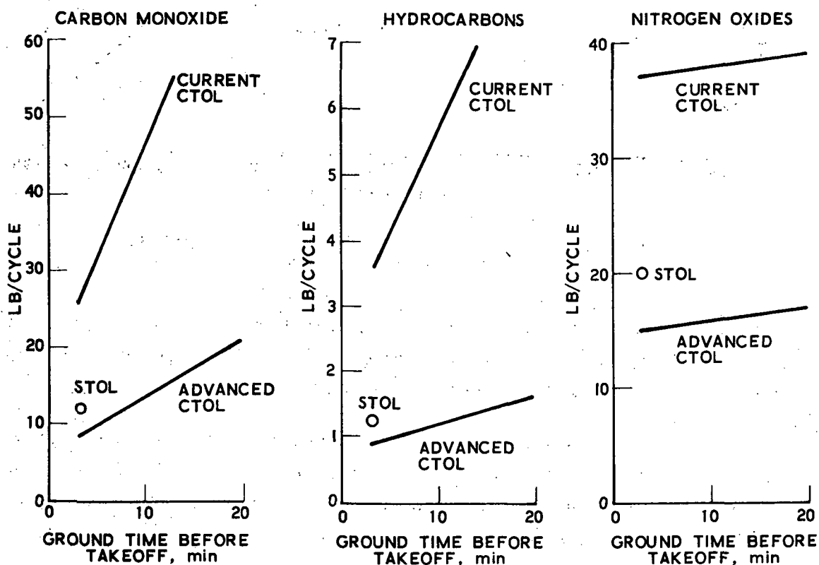
Figure 6. Comparative Emissions for 150-Passenger STOL and CTOL Aircraft
