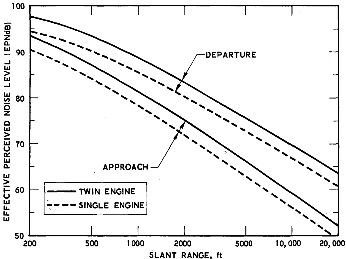
Figure 38. General Aviation Aircraft Noise Characteristics
