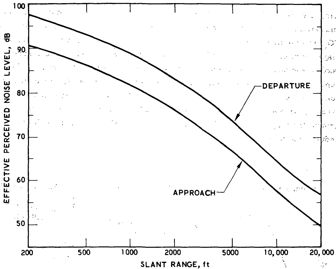
Figure 5. Noise Characteristics, 150-Passenger Augmentor Wing Aircraft
