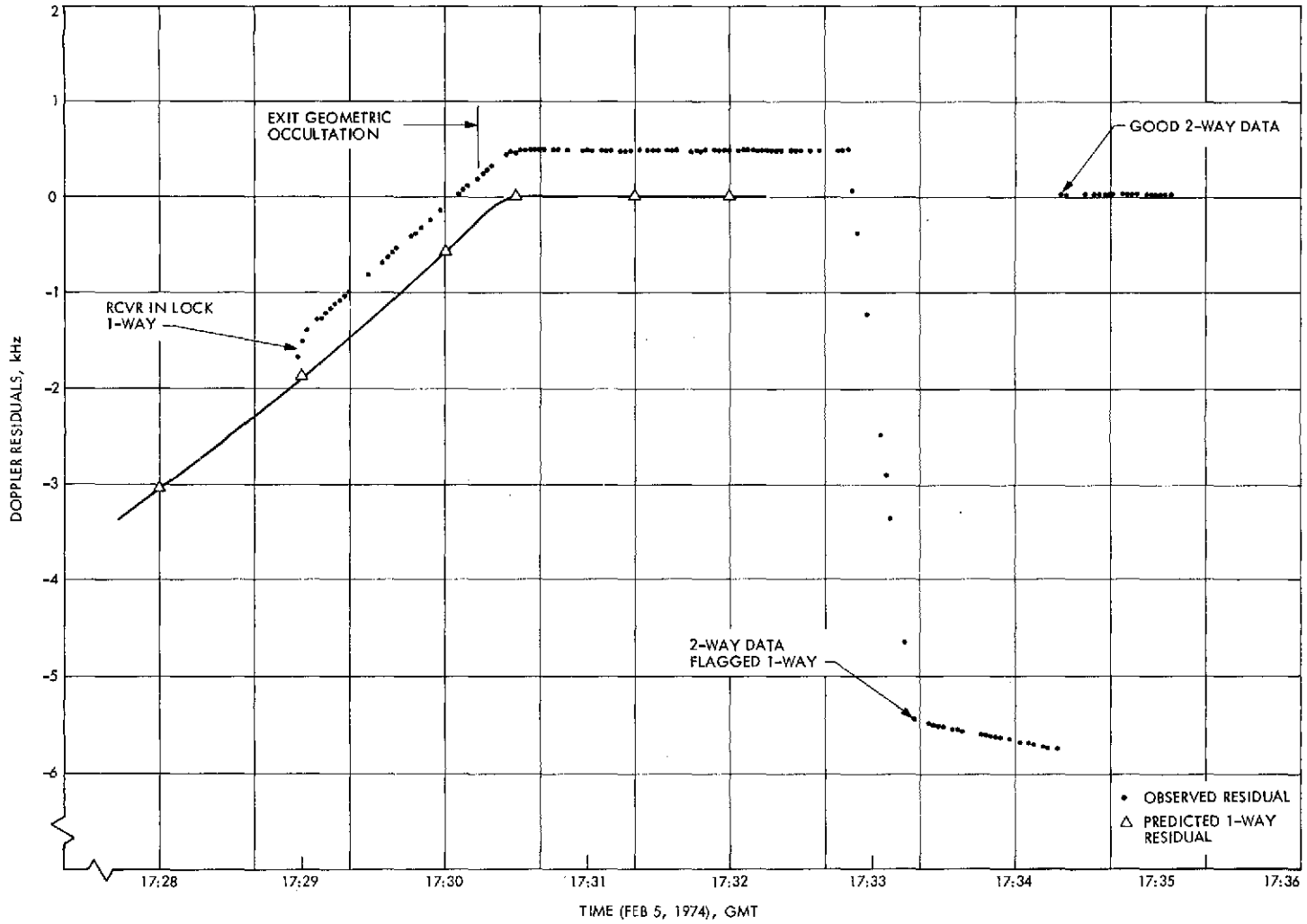
Fig. 6. Exit occultation dopper residuals for Venus encounter (DSS 14 Block IV S-band)
