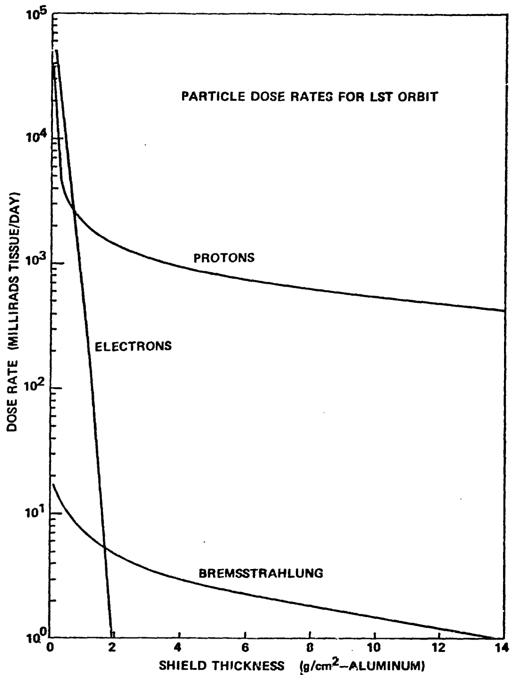
Figure 3. Dose rates due to protons, electrons, and bremsstrahlung versus shield thickness for the LST orbit.
