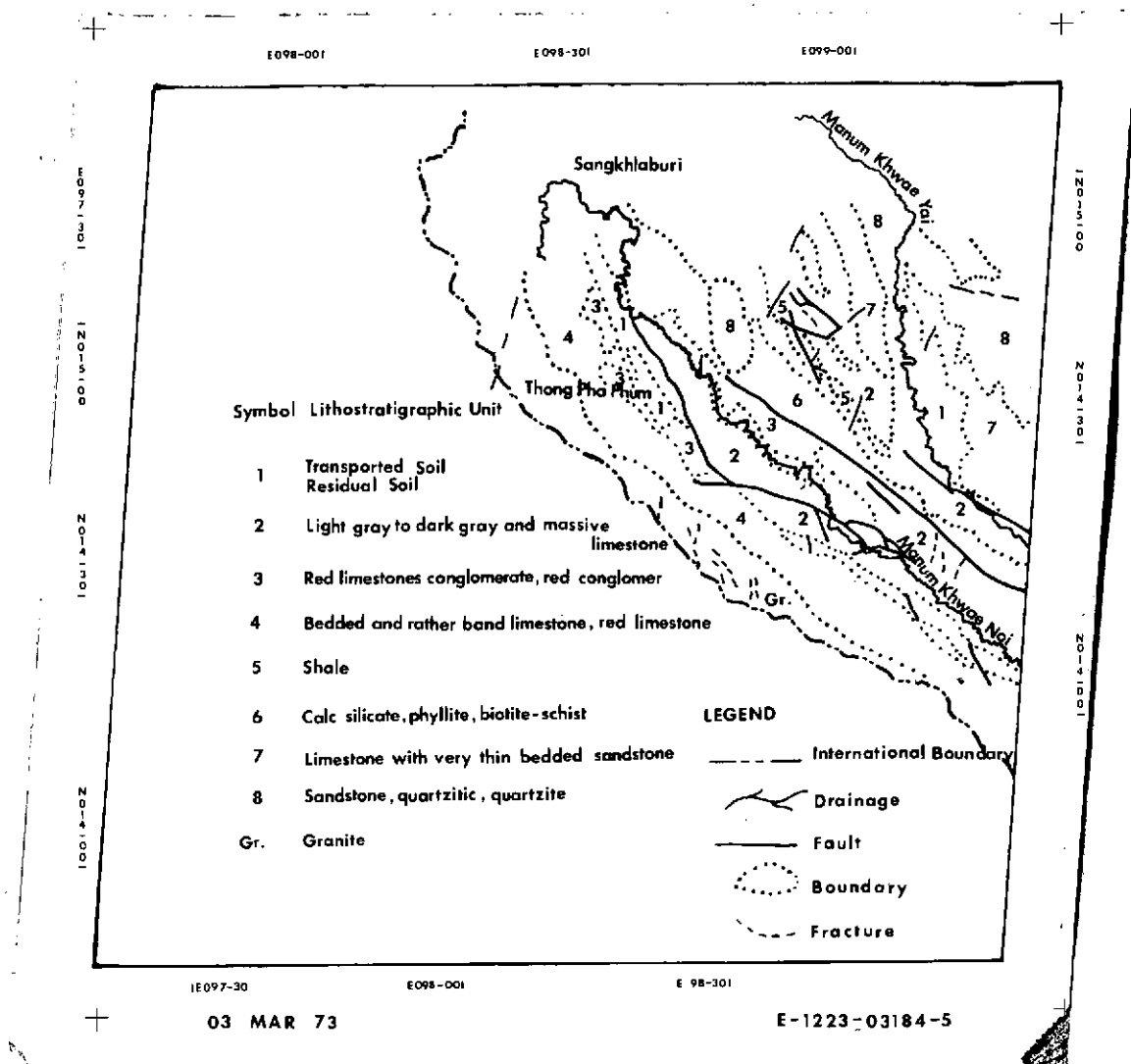
FIGURE 1. Geological Mapping, from ERTS-1 Imagery and Field Survey, Kanchanaburi and River Kwai Area, Thailand.
