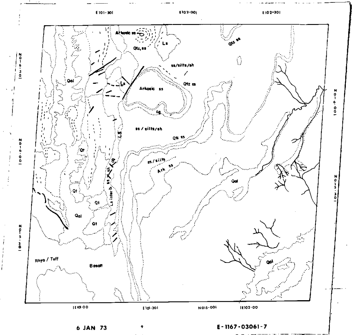
FIGURE 4. Geological Mapping of Figure 3 ERTS-1 Imagery
