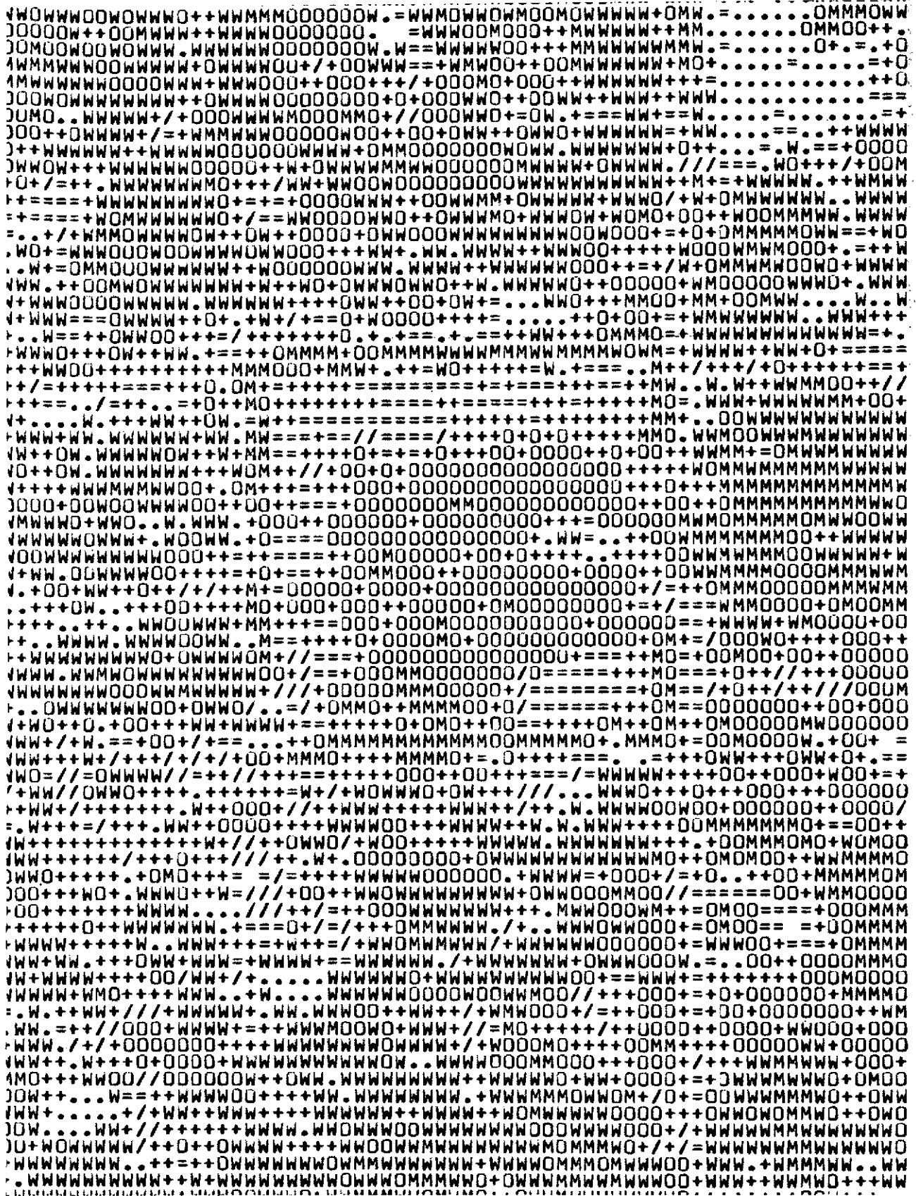
FIGURE 3. Small Section of Purdue IARS Printout, referred to in text. The well defined square area near center is a moated Buddhist compound about 1.5 km square. Original Scale 1:24,000.
