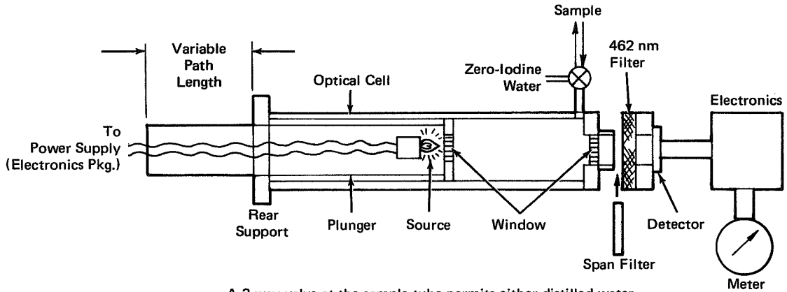
A 3-way valve at the sample tube permits either distilled water (zero iodine) or sample water to enter or leave the cell
