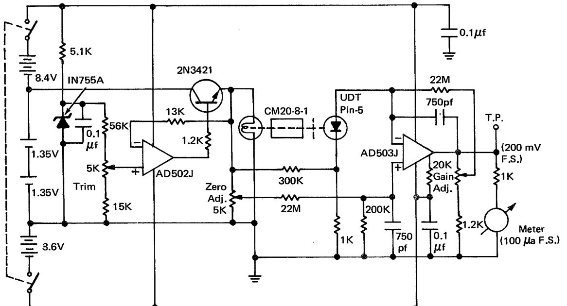
Figure 2. Prototype Circuit
