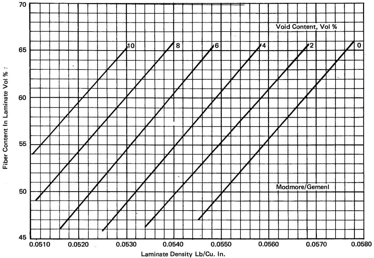
Figure 2. Laminare Density vs. Fiber Volume % for Constant Void Content
