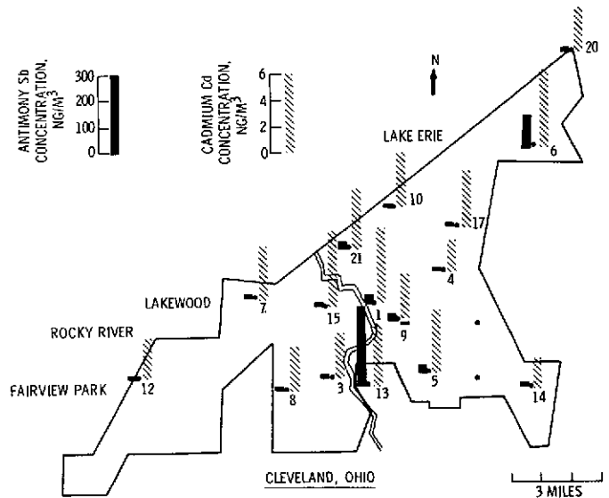
Figure 4. - Comparison of antimony and cadmium concentrations.
