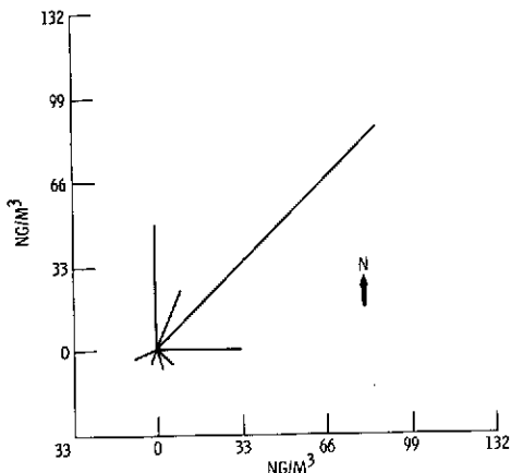
Figure 5. - Concentration rose for antimony at George Washington elementary school.
