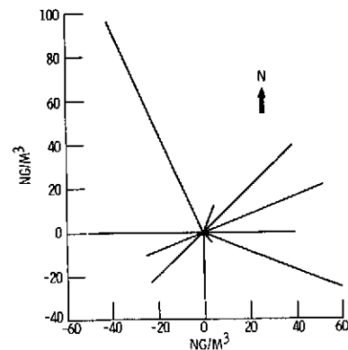
Figure 6. - Concentration rose for antimony at fire station 19.
