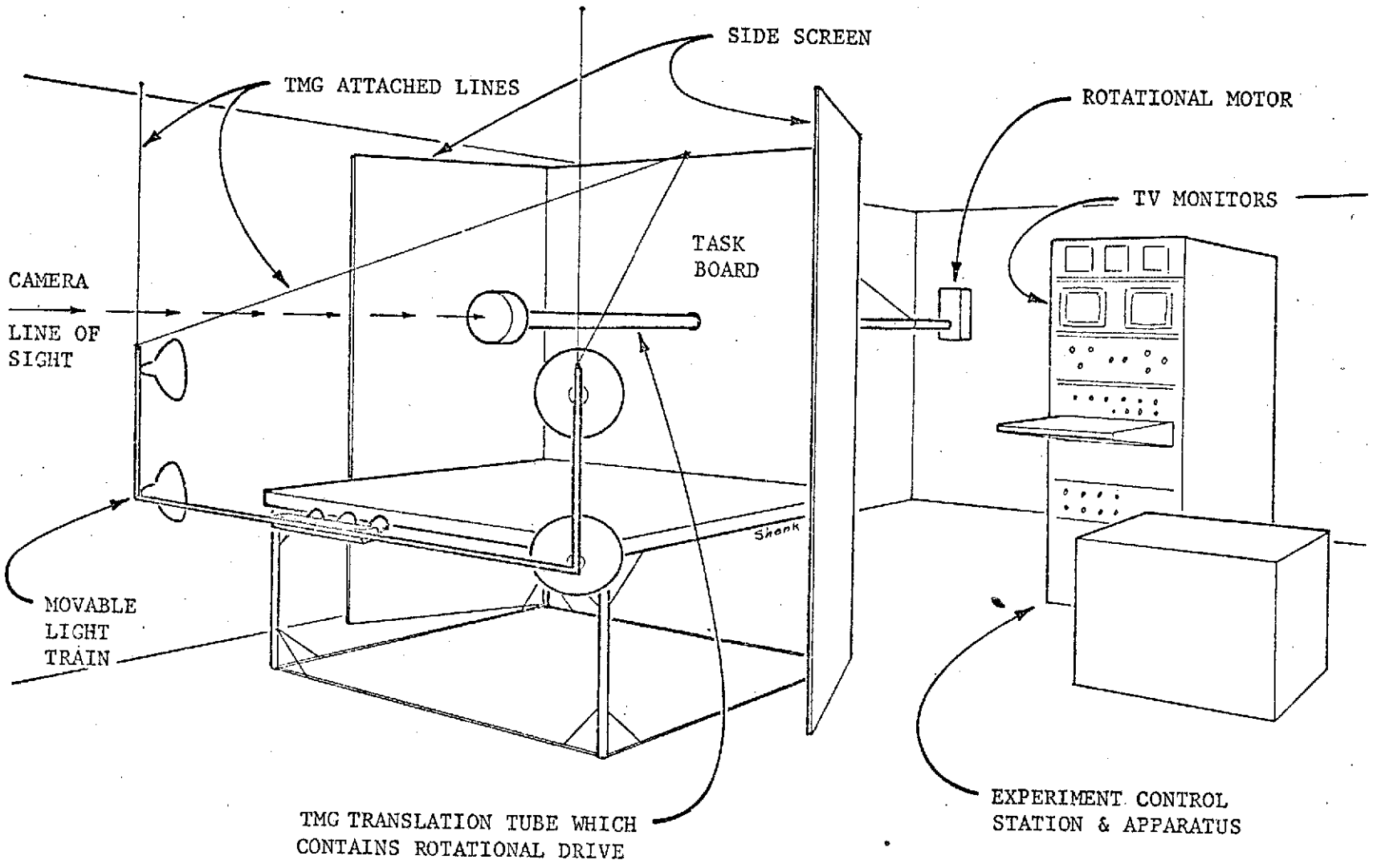
Figure 14. TMG SETUP
