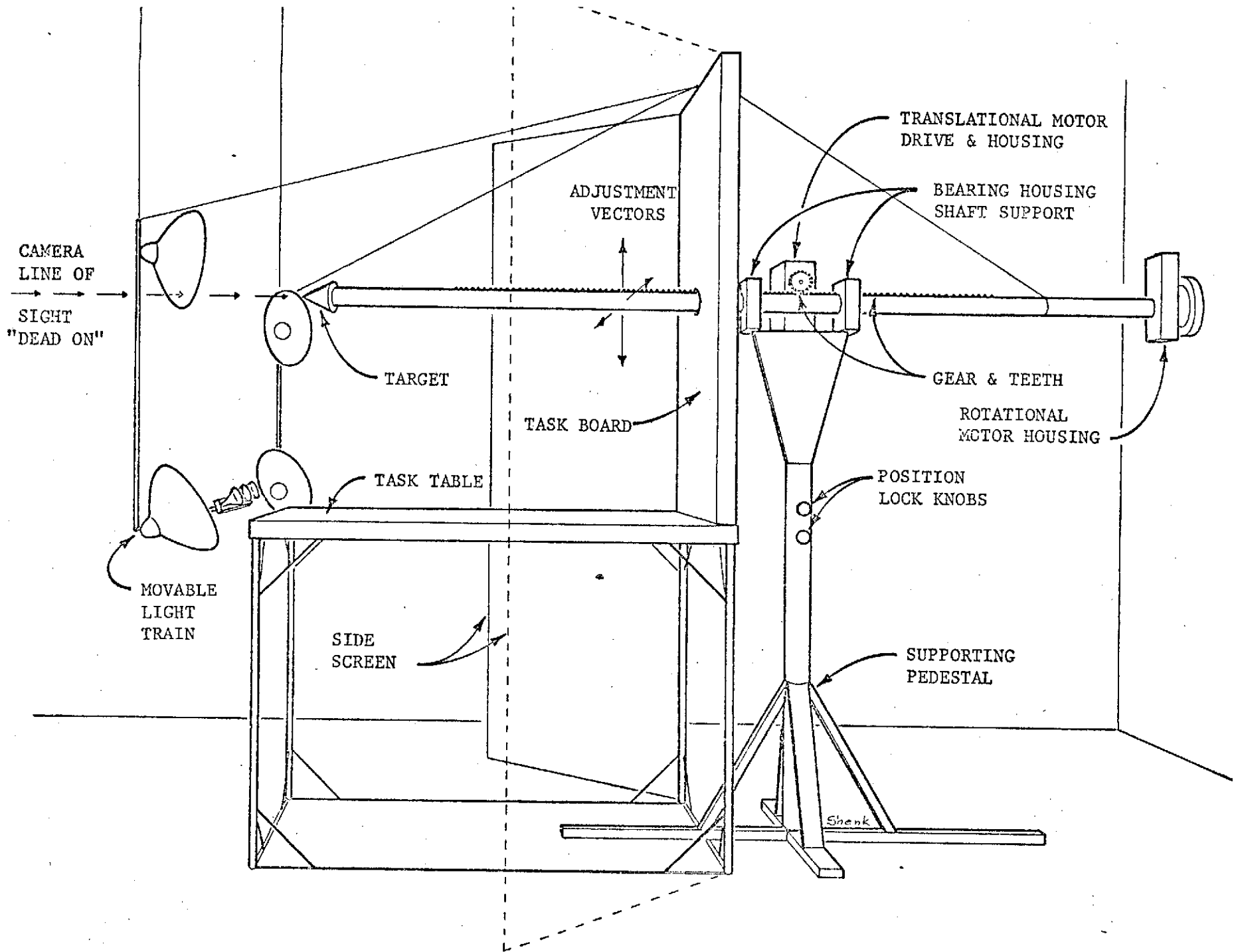
Figure 15. TMG APPARATUS
